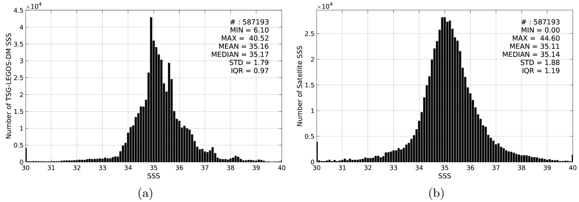
Figure 2: Histograms of SSS from TSG-LEGOS-DM (a) and SMAP-L3-RSS-V2-8DAY-RUNNING-40KM (b) considering all match-up pairs per bins of 0.1 over the SMOS coastal zone ( \approx 800 km) 60N-60S Pi-MEP region and for the full satellite product period.
