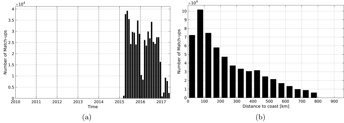
Figure 1: Number of match-ups between TSG-LEGOS-DM and SMAP-L3-RSS-V2-8DAY-RUNNING-40KM SSS as a function of time (a) and as function of the distance to coast (b) over the SMOS coastal zone ( \approx 800 km) 60N-60S Pi-MEP region and for the full satellite product period.
