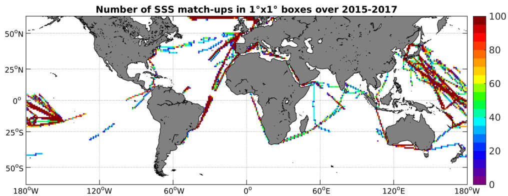
Figure 4: Number of SSS match-ups between TSG-LEGOS-DM SSS and the SMAP-L3-RSS-V2-8DAY-RUNNING-40KM SSS product for the SMOS coastal zone ( \pm 800\text{km} ) 60N-60S Pi-MEP region over 1^\circ \times 1^\circ boxes and for the full satellite product period.
