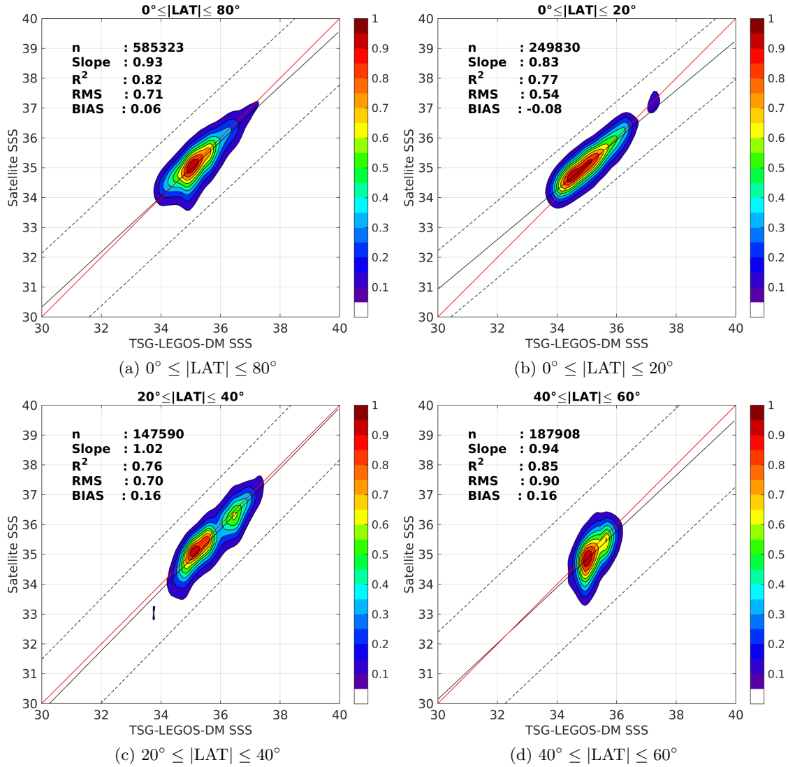
Figure 9: Contour maps of the concentration of SMAP-L3-RSS-V2-8DAY-RUNNING-40KM SSS (y-axis) versus TSG-LEGOS-DM SSS (x-axis) at match-up pairs for different latitude bands. For each plot, the red line shows x=y . The black thin and dashed lines indicate a linear fit through the data cloud and the \pm 95\% confidence levels, respectively. The number match-up pairs n , the slope and R^2 coefficient of the linear fit, the root mean square (RMS) and the mean bias between satellite and in situ data are indicated for each latitude band in each plots.
