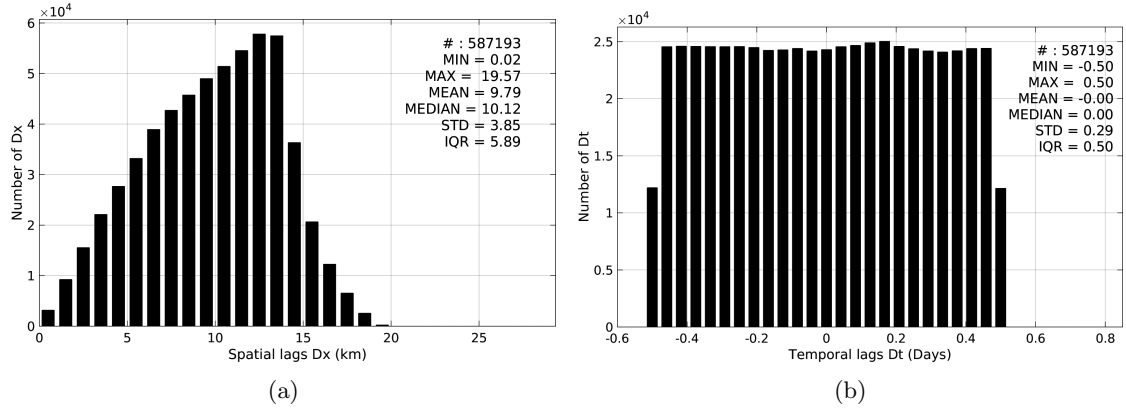
Figure 5: Histograms of the spatial (a) and temporal (b) lags between the time of the TSG-LEGOS-DM measurements and the date of the corresponding SMAP-L3-RSS-V2-8DAY-RUNNING-40KM SSS product.
