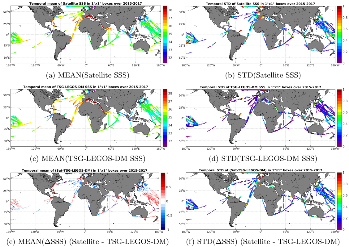
Figure 6: Temporal mean (left) and STD (right) of SSS from SMAP-L3-RSS-V2-8DAY-RUNNING-40KM (top), TSG-LEGOS-DM (middle), and of \Delta SSS (Satellite - TSG-LEGOS-DM). Only match-up pairs are used to generate these maps.
