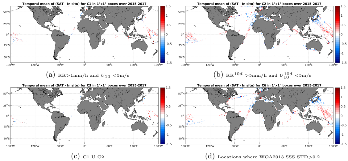
Figure 12: Temporal mean gridded over spatial boxes of size 1^\circ \times 1^\circ of \Delta SSS (SMAP-L3-RSS-V2-8DAY-RUNNING-40KM - TSG-LEGOS-DM) for 4 different subdatasets corresponding to: RR > 1\text{mm/h} and U_{10} < 5\text{m/s} (a), RR^{10d} > 5\text{mm/h} and U_{10}^{10d} < 5\text{m/s} (b), C1 U C2 (c), Locations where WOA2013 SSS STD > 0.2 (d).
