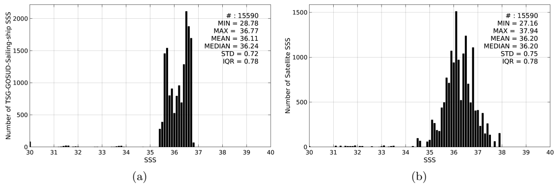
Figure 2: Histograms of SSS from TSG-GOSUD-Sailing-ship (a) and SMAP-L3-RSS-V2-8DAY-RUNNING-40KM (b) considering all match-up pairs per bins of 0.1 over the SMOS coastal zone ( \approx 800\text{km} ) 60N-60S Pi-MEP region and for the full satellite product period.
