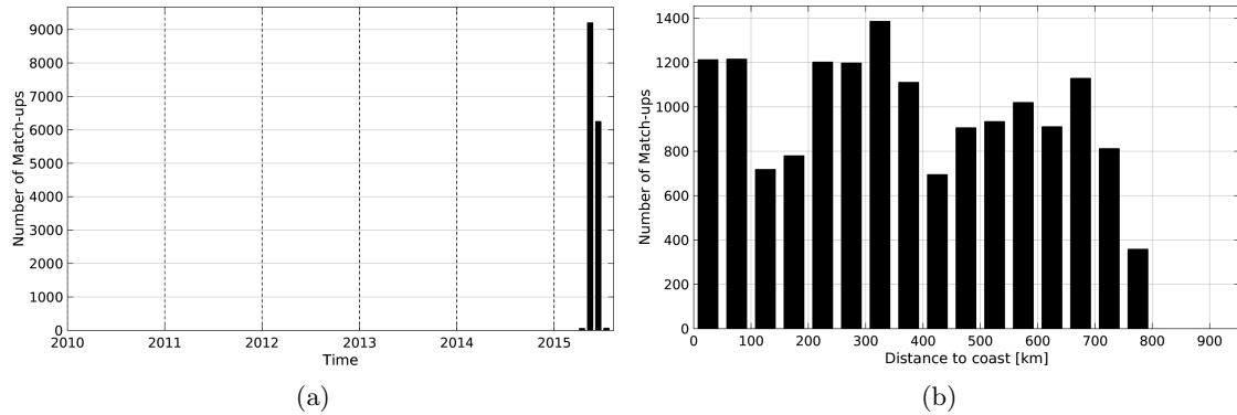
Figure 1: Number of match-ups between TSG-GOSUD-Sailing-ship and SMAP-L3-RSS-V2-8DAY-RUNNING-40KM SSS as a function of time (a) and as function of the distance to coast (b) over the SMOS coastal zone ( \approx 800\text{km} ) 60N-60S Pi-MEP region and for the full satellite product period.
