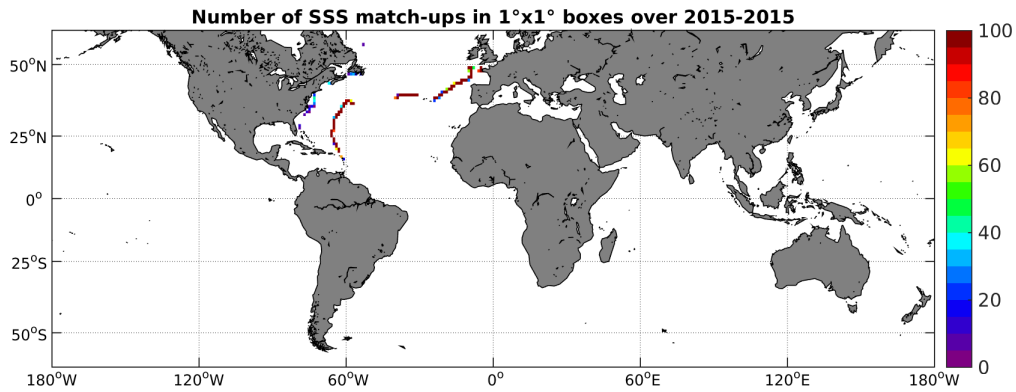
Figure 4: Number of SSS match-ups between TSG-GOSUD-Sailing-ship SSS and the SMAP-L3-RSS-V2-8DAY-RUNNING-40KM SSS product for the SMOS coastal zone ( \pm 800\text{km} ) 60N-60S Pi-MEP region over 1^\circ \times 1^\circ boxes and for the full satellite product period.
