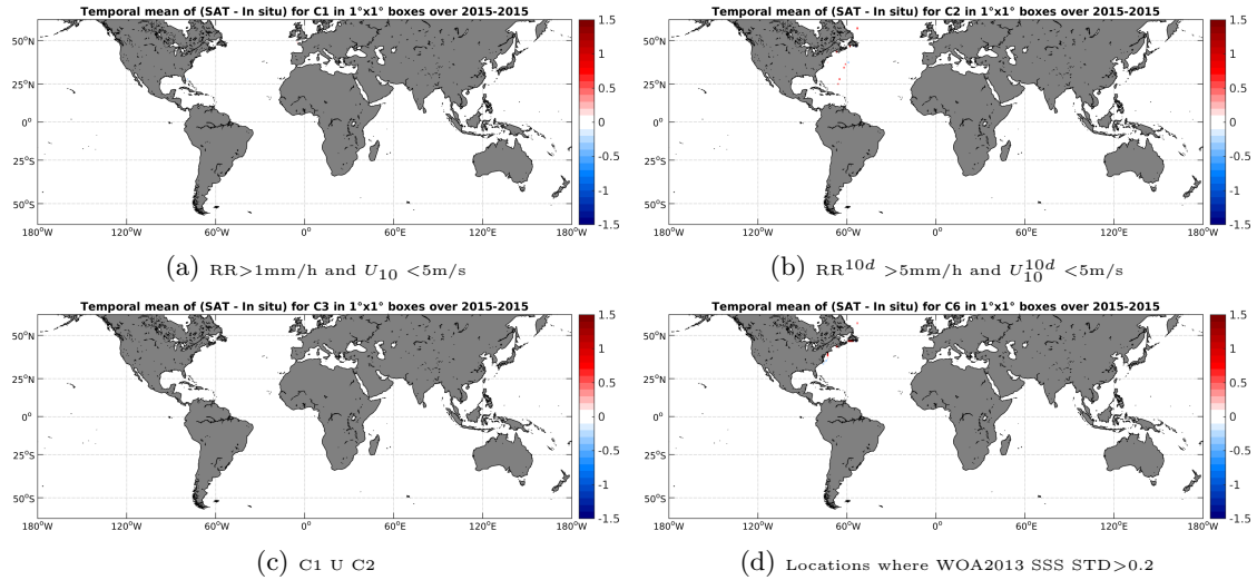
Figure 12: Temporal mean gridded over spatial boxes of size 1^\circ \times 1^\circ of \Delta SSS (SMAP-L3-RSS-V2-8DAY-RUNNING-40KM - TSG-GOSUD-Sailing-ship) for 4 different subdatasets corresponding to: RR > 1\text{mm/h} and U_{10} < 5\text{m/s} (a), RR^{10d} > 5\text{mm/h} and U_{10}^{10d} < 5\text{m/s} (b), C1 U C2 (c), Locations where WOA2013 SSS STD > 0.2 (d).
