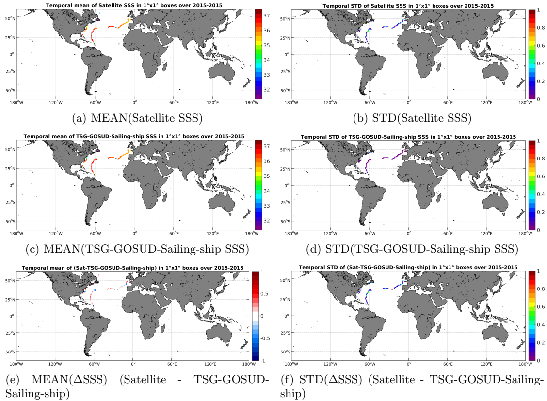
Figure 6: Temporal mean (left) and STD (right) of SSS from SMAP-L3-RSS-V2-8DAY-RUNNING-40KM (top), TSG-GOSUD-Sailing-ship (middle), and of \Delta SSS (Satellite - TSG-GOSUD-Sailing-ship). Only match-up pairs are used to generate these maps.
