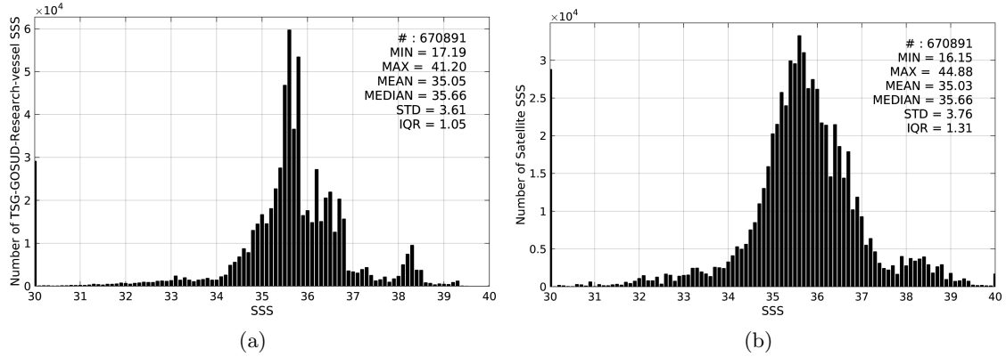
Figure 2: Histograms of SSS from TSG-GOSUD-Research-vessel (a) and SMAP-L3-RSS-V2-8DAY-RUNNING-40KM (b) considering all match-up pairs per bins of 0.1 over the SMOS coastal zone ( \leq 800 km) 60N-60S Pi-MEP region and for the full satellite product period.
