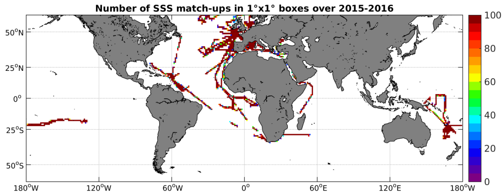
Figure 4: Number of SSS match-ups between TSG-GOSUD-Research-vessel SSS and the SMAP-L3-RSS-V2-8DAY-RUNNING-40KM SSS product for the SMOS coastal zone ( \geq 800\text{km} ) 60N-60S Pi-MEP region over 1^\circ \times 1^\circ boxes and for the full satellite product period.
