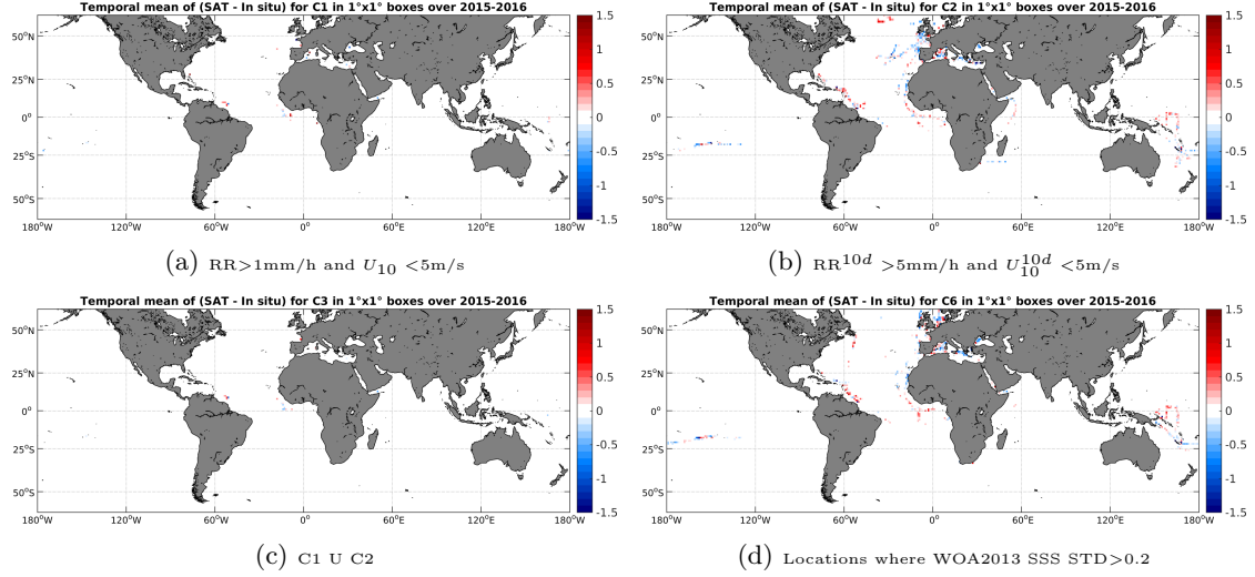
Figure 12: Temporal mean gridded over spatial boxes of size 1^\circ \times 1^\circ of \Delta SSS (SMAP-L3-RSS-V2-8DAY-RUNNING-40KM - TSG-GOSUD-Research-vessel) for 4 different subdatasets corresponding to: RR > 1 mm/h and U_{10} < 5 m/s (a), RR^{10d} > 5 mm/h and U_{10}^{10d} < 5 m/s (b), C1 U C2 (c), Locations where WOA2013 SSS STD > 0.2 (d).
