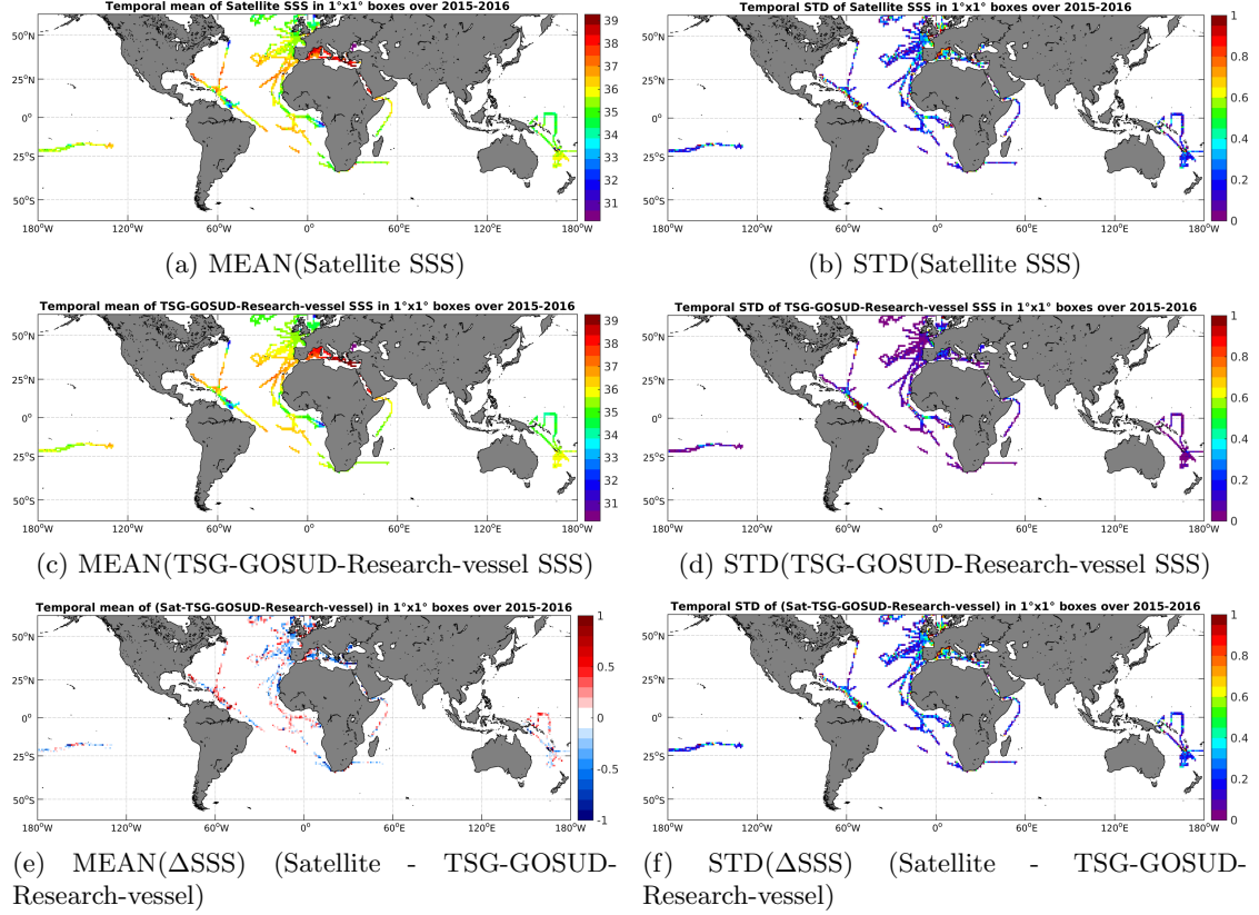
Figure 6: Temporal mean (left) and STD (right) of SSS from SMAP-L3-RSS-V2-8DAY-RUNNING-40KM (top), TSG-GOSUD-Research-vessel (middle), and of \Delta SSS (Satellite - TSG-GOSUD-Research-vessel). Only match-up pairs are used to generate these maps.
