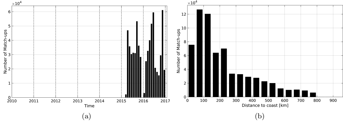
Figure 1: Number of match-ups between TSG-GOSUD-Research-vessel and SMAP-L3-RSS-V2-8DAY-RUNNING-40KM SSS as a function of time (a) and as function of the distance to coast (b) over the SMOS coastal zone ( \leq 800 km) 60N-60S Pi-MEP region and for the full satellite product period.
