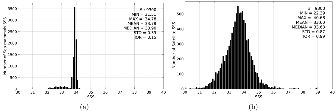
Figure 2: Histograms of SSS from Sea mammals (a) and SMAP-L3-RSS-V2-8DAY-RUNNING-40KM (b) considering all match-up pairs per bins of 0.1 over the SMOS coastal zone ( \leq 800 km) 60N-60S Pi-MEP region and for the full satellite product period.
