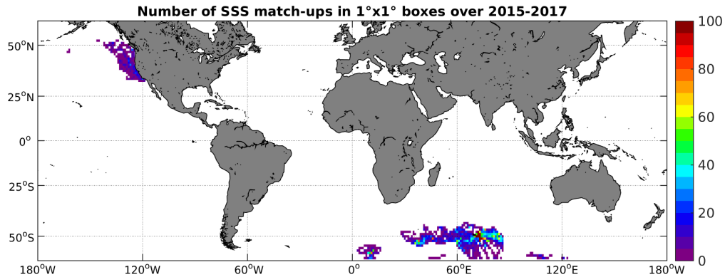
Figure 4: Number of SSS match-ups between Sea mammals SSS and the SMAP-L3-RSS-V2-8DAY-RUNNING-40KM SSS product for the SMOS coastal zone ( \pm 800\text{km} ) 60N-60S Pi-MEP region over 1^\circ \times 1^\circ boxes and for the full satellite product period.
