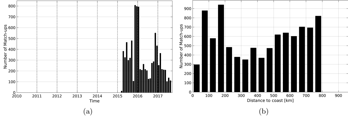
Figure 1: Number of match-ups between Sea mammals and SMAP-L3-RSS-V2-8DAY-RUNNING-40KM SSS as a function of time (a) and as function of the distance to coast (b) over the SMOS coastal zone ( \leq 800 km) 60N-60S Pi-MEP region and for the full satellite product period.
