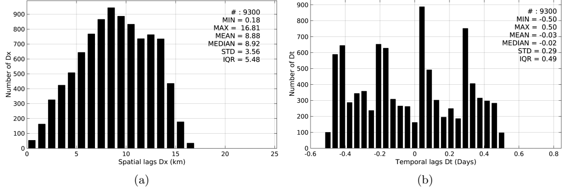
Figure 5: Histograms of the spatial (a) and temporal (b) lags between the time of the Sea mammals measurements and the date of the corresponding SMAP-L3-RSS-V2-8DAY-RUNNING-40KM SSS product.
