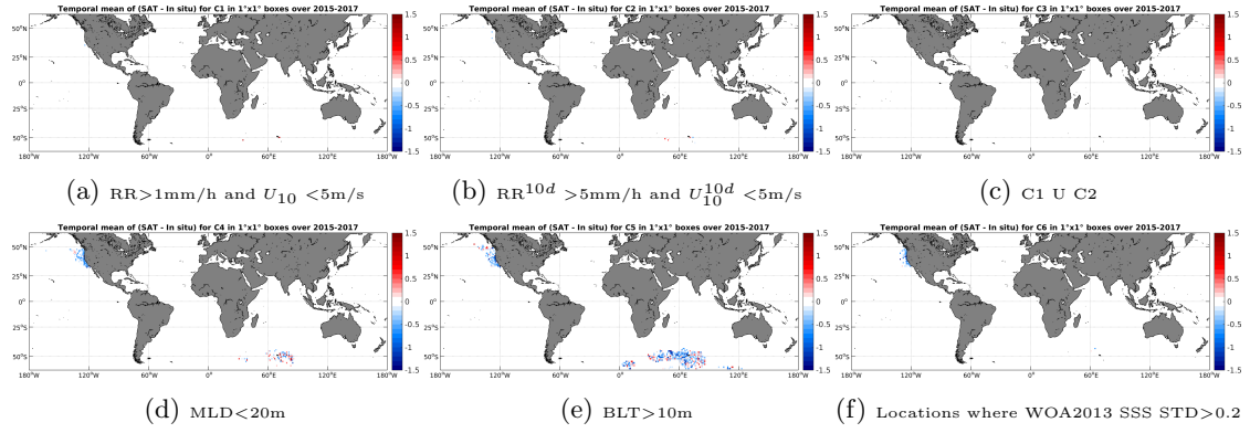
Figure 12: Temporal mean gridded over spatial boxes of size 1^\circ \times 1^\circ of \Delta SSS (SMAP-L3-RSS-V2-8DAY-RUNNING-40KM - Sea mammals) for 6 different subdatasets corresponding to: RR > 1\text{mm/h} and U_{10} < 5\text{m/s} (a), RR^{10d} > 5\text{mm/h} and U_{10}^{10d} < 5\text{m/s} (b), C1 U C2 (c), MLD < 20\text{m} (d), BLT > 10\text{m} (e), Locations where WOA2013 SSS STD > 0.2 (f).
