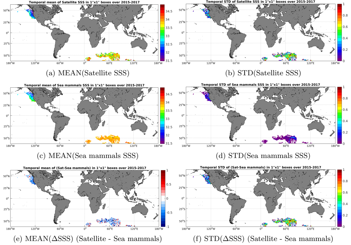
Figure 6: Temporal mean (left) and STD (right) of SSS from SMAP-L3-RSS-V2-8DAY-RUNNING-40KM (top), Sea mammals (middle), and of \Delta SSS (Satellite - Sea mammals). Only match-up pairs are used to generate these maps.
