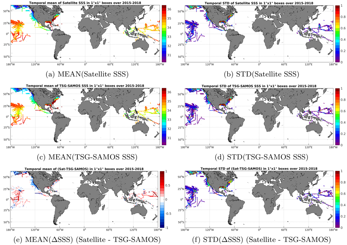
Figure 6: Temporal mean (left) and STD (right) of SSS from SMAP-L3-RSS-V2-8DAY-RUNNING-70KM (top), TSG-SAMOS (middle), and of \Delta SSS (Satellite - TSG-SAMOS). Only match-up pairs are used to generate these maps.
