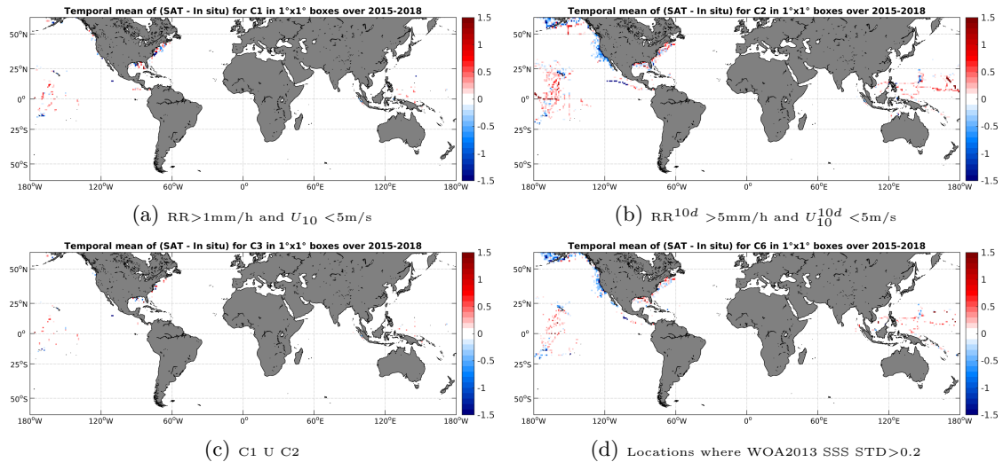
Figure 12: Temporal mean gridded over spatial boxes of size 1^\circ \times 1^\circ of \Delta SSS (SMAP-L3-RSS-V2-8DAY-RUNNING-70KM - TSG-SAMOS) for 4 different subdatasets corresponding to: RR > 1\text{mm/h} and U_{10} < 5\text{m/s} (a), RR^{10d} > 5\text{mm/h} and U_{10}^{10d} < 5\text{m/s} (b), C1 U C2 (c), Locations where WOA2013 SSS STD > 0.2 (d).
