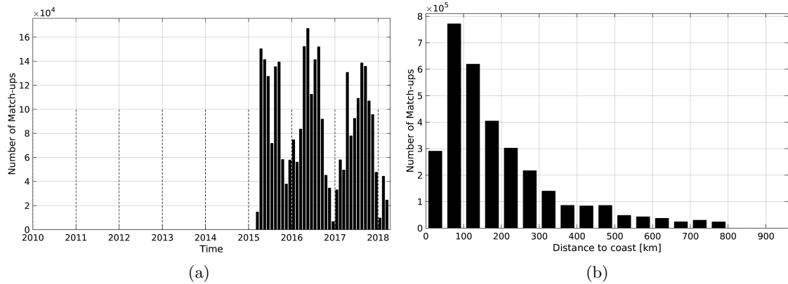
Figure 1: Number of match-ups between TSG-SAMOS and SMAP-L3-RSS-V2-8DAY-RUNNING-70KM SSS as a function of time (a) and as function of the distance to coast (b) over the SMOS coastal zone ( \leq 800 km) 60N-60S Pi-MEP region and for the full satellite product period.
