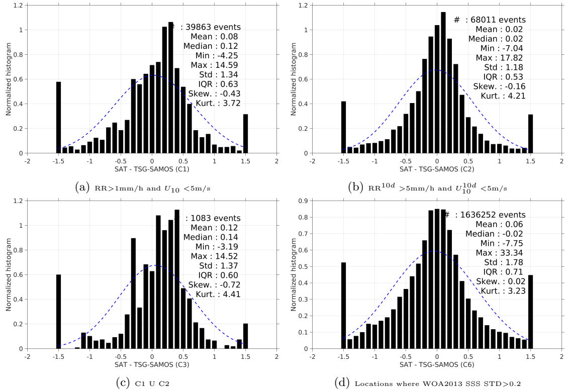
Figure 13: Normalized histogram of \Delta SSS (SMAP-L3-RSS-V2-8DAY-RUNNING-70KM - TSG-SAMOS) for 6 different subdatasets corresponding to: RR > 1\text{mm/h} and U_{10} < 5\text{m/s} (a), RR^{10d} > 5\text{mm/h} and U_{10}^{10d} < 5\text{m/s} (b), C1 U C2 (c), Locations where WOA2013 SSS STD > 0.2 (d).
