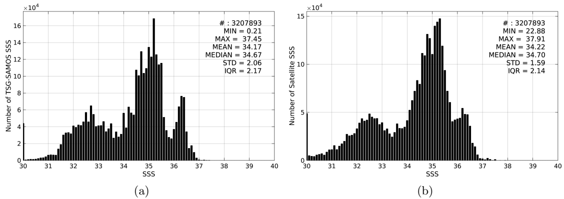
Figure 2: Histograms of SSS from TSG-SAMOS (a) and SMAP-L3-RSS-V2-8DAY-RUNNING-70KM (b) considering all match-up pairs per bins of 0.1 over the SMOS coastal zone ( \leq 800 km) 60N-60S Pi-MEP region and for the full satellite product period.
