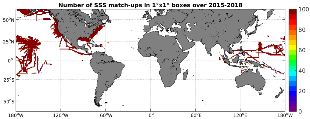
Figure 4: Number of SSS match-ups between TSG-SAMOS SSS and the SMAP-L3-RSS-V2-8DAY-RUNNING-70KM SSS product for the SMOS coastal zone ( \pm 800 km) 60N-60S Pi-MEP region over 1^\circ \times 1^\circ boxes and for the full satellite product period.
