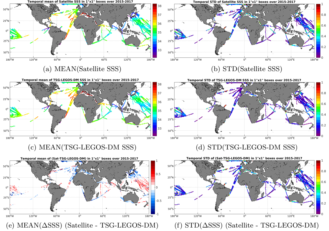
Figure 6: Temporal mean (left) and STD (right) of SSS from SMAP-L3-RSS-V2-8DAY-RUNNING-70KM (top), TSG-LEGOS-DM (middle), and of \Delta SSS (Satellite - TSG-LEGOS-DM). Only match-up pairs are used to generate these maps.
