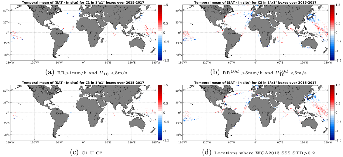
Figure 12: Temporal mean gridded over spatial boxes of size 1^\circ \times 1^\circ of \Delta SSS (SMAP-L3-RSS-V2-8DAY-RUNNING-70KM - TSG-LEGOS-DM) for 4 different subdatasets corresponding to: RR > 1mm/h and U_{10} < 5 m/s (a), RR^{10d} > 5 mm/h and U_{10}^{10d} < 5 m/s (b), C1 U C2 (c), Locations where WOA2013 SSS STD > 0.2 (d).
