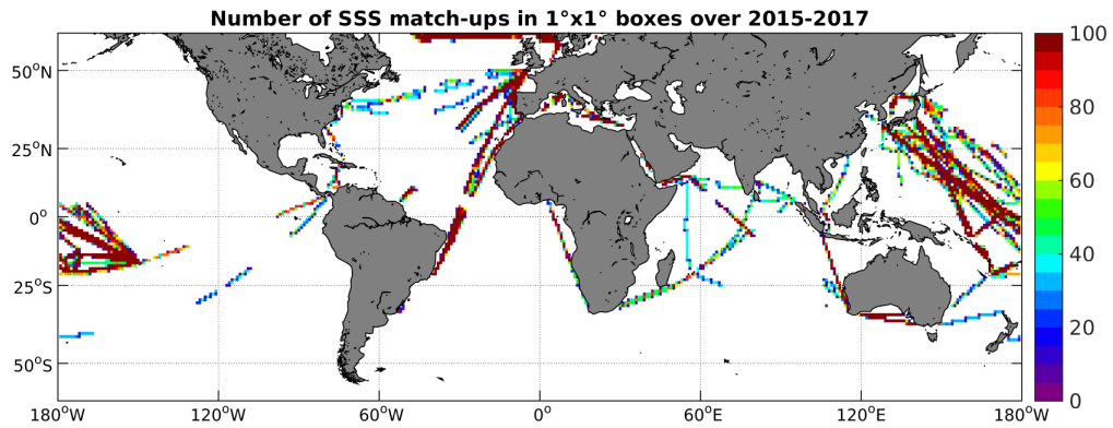
Figure 4: Number of SSS match-ups between TSG-LEGOS-DM SSS and the SMAP-L3-RSS-V2-8DAY-RUNNING-70KM SSS product for the SMOS coastal zone ( \pm 800\text{km} ) 60N-60S Pi-MEP region over 1^\circ \times 1^\circ boxes and for the full satellite product period.
