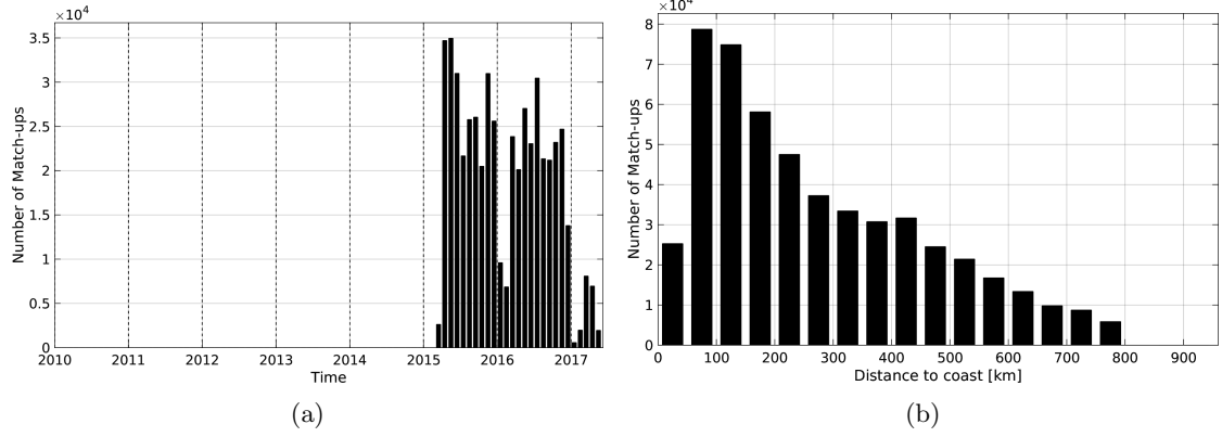
Figure 1: Number of match-ups between TSG-LEGOS-DM and SMAP-L3-RSS-V2-8DAY-RUNNING-70KM SSS as a function of time (a) and as function of the distance to coast (b) over the SMOS coastal zone ( \leq 800 km) 60N-60S Pi-MEP region and for the full satellite product period.
