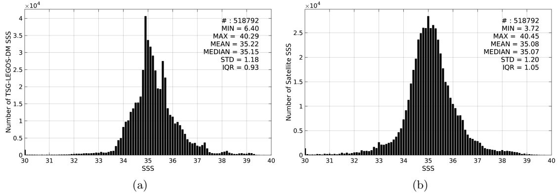
Figure 2: Histograms of SSS from TSG-LEGOS-DM (a) and SMAP-L3-RSS-V2-8DAY-RUNNING-70KM (b) considering all match-up pairs per bins of 0.1 over the SMOS coastal zone ( \leq 800 km) 60N-60S Pi-MEP region and for the full satellite product period.
