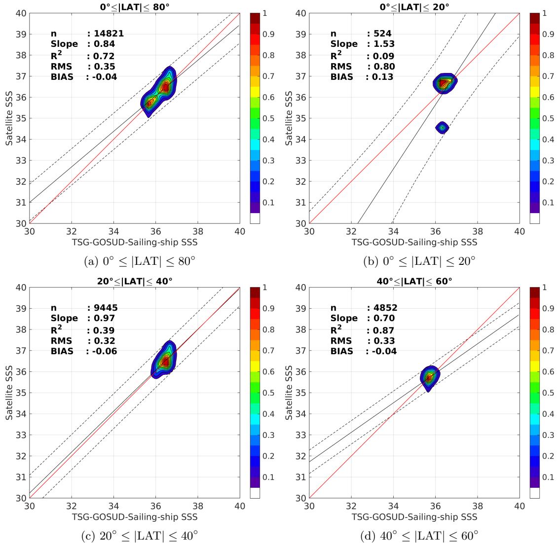
Figure 9: Contour maps of the concentration of SMAP-L3-RSS-V2-8DAY-RUNNING-70KM SSS (y-axis) versus TSG-GOSUD-Sailing-ship SSS (x-axis) at match-up pairs for different latitude bands. For each plot, the red line shows x=y . The black thin and dashed lines indicate a linear fit through the data cloud and the \pm 95\% confidence levels, respectively. The number match-up pairs n , the slope and R^2 coefficient of the linear fit, the root mean square (RMS) and the mean bias between satellite and in situ data are indicated for each latitude band in each plots.
