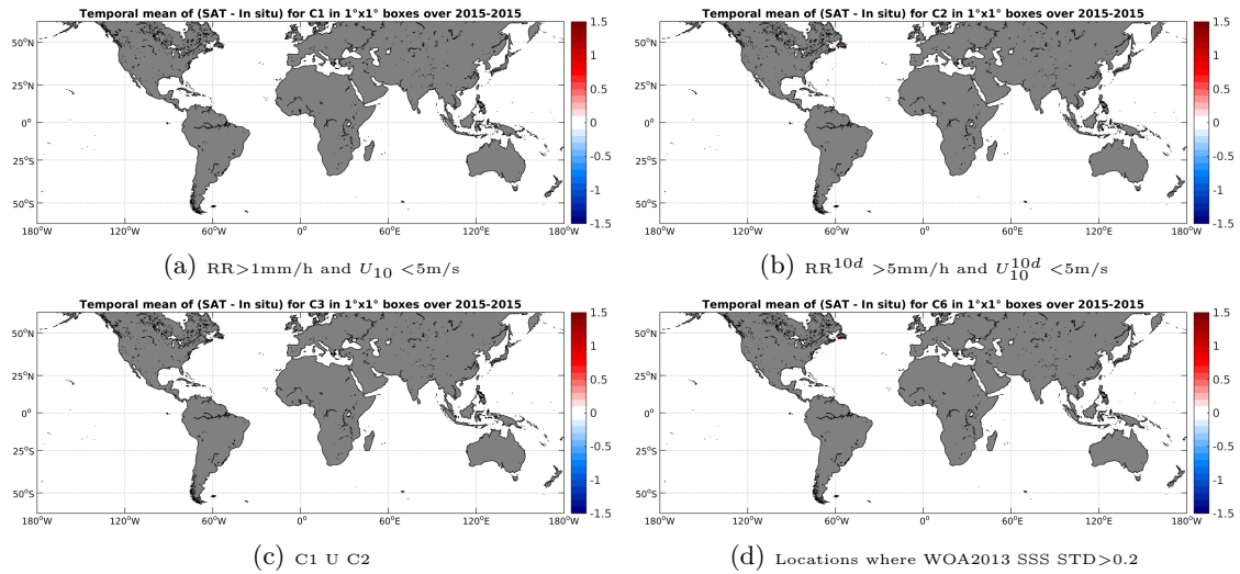
Figure 12: Temporal mean gridded over spatial boxes of size 1^\circ \times 1^\circ of \Delta SSS (SMAP-L3-RSS-V2-8DAY-RUNNING-70KM - TSG-GOSUD-Sailing-ship) for 4 different subdatasets corresponding to: RR > 1\text{mm/h} and U_{10} < 5\text{m/s} (a), RR^{10d} > 5\text{mm/h} and U_{10}^{10d} < 5\text{m/s} (b), C1 U C2 (c), Locations where WOA2013 SSS STD > 0.2 (d).
