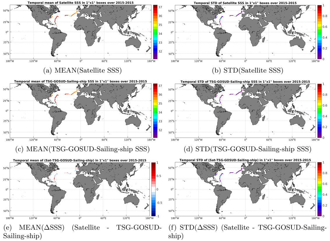
Figure 6: Temporal mean (left) and STD (right) of SSS from SMAP-L3-RSS-V2-8DAY-RUNNING-70KM (top), TSG-GOSUD-Sailing-ship (middle), and of \Delta SSS (Satellite - TSG-GOSUD-Sailing-ship). Only match-up pairs are used to generate these maps.
