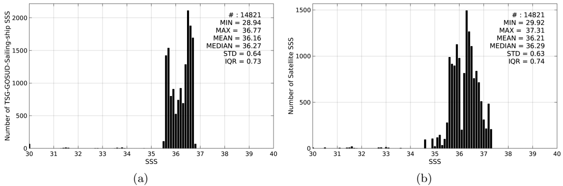
Figure 2: Histograms of SSS from TSG-GOSUD-Sailing-ship (a) and SMAP-L3-RSS-V2-8DAY-RUNNING-70KM (b) considering all match-up pairs per bins of 0.1 over the SMOS coastal zone ( \geq 800\text{km} ) 60N-60S Pi-MEP region and for the full satellite product period.
