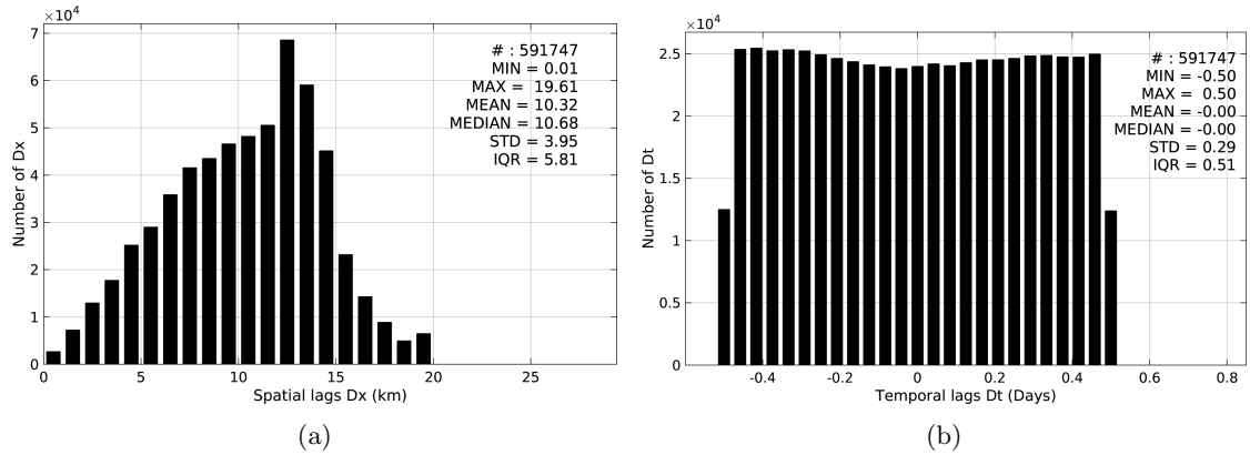
Figure 5: Histograms of the spatial (a) and temporal (b) lags between the time of the TSG-GOSUD-Research-vessel measurements and the date of the corresponding SMAP-L3-RSS-V2-8DAY-RUNNING-70KM SSS product.
