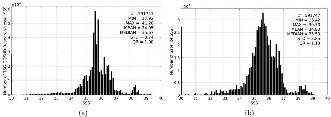
Figure 2: Histograms of SSS from TSG-GOSUD-Research-vessel (a) and SMAP-L3-RSS-V2-8DAY-RUNNING-70KM (b) considering all match-up pairs per bins of 0.1 over the SMOS coastal zone ( \approx 800 km) 60N-60S Pi-MEP region and for the full satellite product period.
