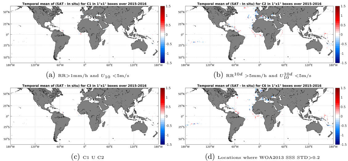
Figure 12: Temporal mean gridded over spatial boxes of size 1^\circ \times 1^\circ of \Delta SSS (SMAP-L3-RSS-V2-8DAY-RUNNING-70KM - TSG-GOSUD-Research-vessel) for 4 different subdatasets corresponding to: RR > 1\text{mm/h} and U_{10} < 5\text{m/s} (a), RR^{10d} > 5\text{mm/h} and U_{10}^{10d} < 5\text{m/s} (b), C1 U C2 (c), Locations where WOA2013 SSS STD > 0.2 (d).
