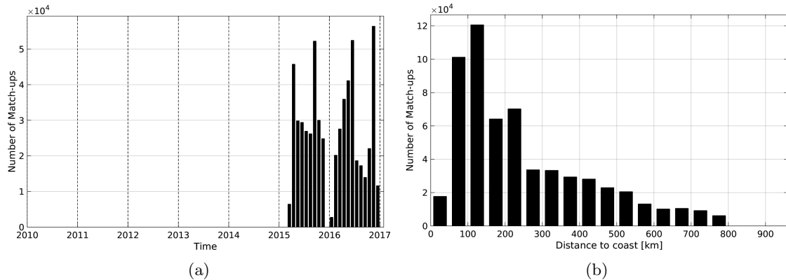
Figure 1: Number of match-ups between TSG-GOSUD-Research-vessel and SMAP-L3-RSS-V2-8DAY-RUNNING-70KM SSS as a function of time (a) and as function of the distance to coast (b) over the SMOS coastal zone ( \approx 800 km) 60N-60S Pi-MEP region and for the full satellite product period.
