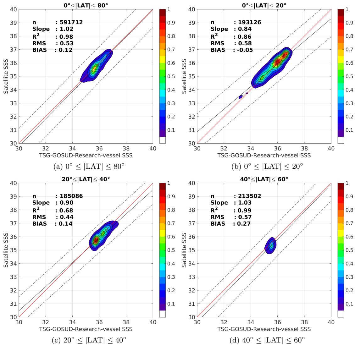
Figure 9: Contour maps of the concentration of SMAP-L3-RSS-V2-8DAY-RUNNING-70KM SSS (y-axis) versus TSG-GOSUD-Research-vessel SSS (x-axis) at match-up pairs for different latitude bands. For each plot, the red line shows x=y . The black thin and dashed lines indicate a linear fit through the data cloud and the \pm 95\% confidence levels, respectively. The number match-up pairs n , the slope and R^2 coefficient of the linear fit, the root mean square (RMS) and the mean bias between satellite and in situ data are indicated for each latitude band in each plots.
