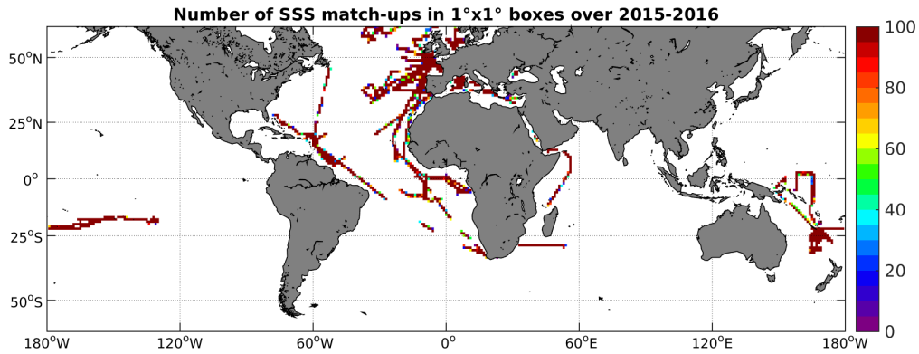
Figure 4: Number of SSS match-ups between TSG-GOSUD-Research-vessel SSS and the SMAP-L3-RSS-V2-8DAY-RUNNING-70KM SSS product for the SMOS coastal zone ( \pm 800\text{km} ) 60N-60S Pi-MEP region over 1^\circ \times 1^\circ boxes and for the full satellite product period.
