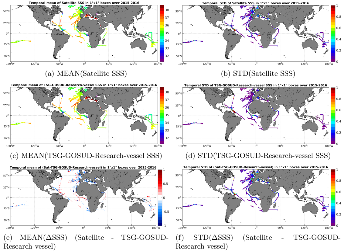
Figure 6: Temporal mean (left) and STD (right) of SSS from SMAP-L3-RSS-V2-8DAY-RUNNING-70KM (top), TSG-GOSUD-Research-vessel (middle), and of \Delta SSS (Satellite - TSG-GOSUD-Research-vessel). Only match-up pairs are used to generate these maps.
