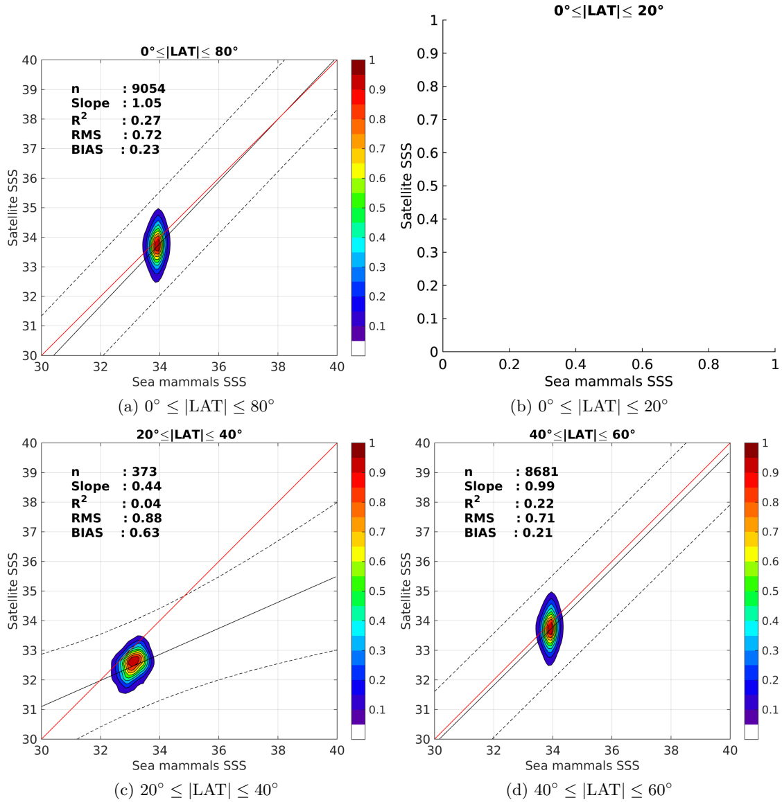
Figure 9: Contour maps of the concentration of SMAP-L3-RSS-V2-8DAY-RUNNING-70KM SSS (y-axis) versus Sea mammals SSS (x-axis) at match-up pairs for different latitude bands. For each plot, the red line shows x=y . The black thin and dashed lines indicate a linear fit through the data cloud and the \pm 95\% confidence levels, respectively. The number match-up pairs n , the slope and R^2 coefficient of the linear fit, the root mean square (RMS) and the mean bias between satellite and in situ data are indicated for each latitude band in each plots.
