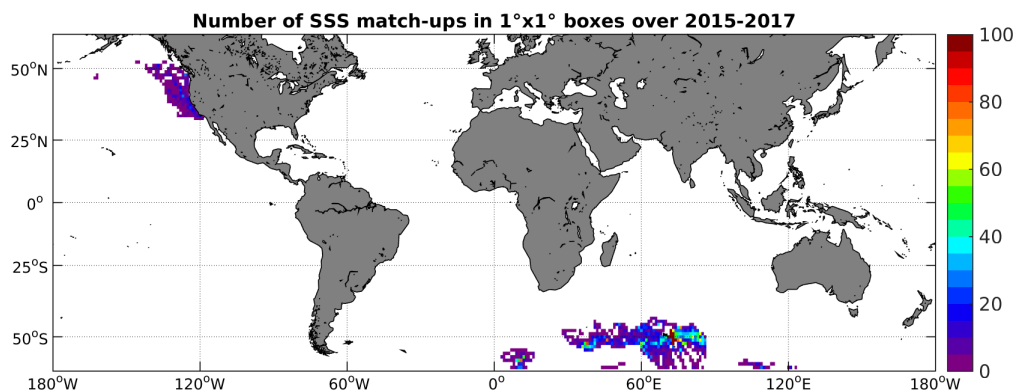
Figure 4: Number of SSS match-ups between Sea mammals SSS and the SMAP-L3-RSS-V2-8DAY-RUNNING-70KM SSS product for the SMOS coastal zone ( \pm 800\text{km} ) 60N-60S Pi-MEP region over 1^\circ \times 1^\circ boxes and for the full satellite product period.
