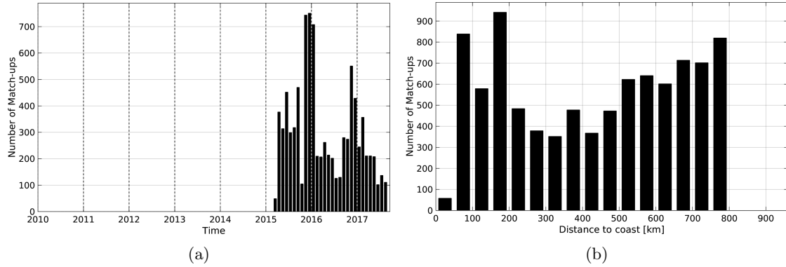
Figure 1: Number of match-ups between Sea mammals and SMAP-L3-RSS-V2-8DAY-RUNNING-70KM SSS as a function of time (a) and as function of the distance to coast (b) over the SMOS coastal zone ( \approx 800 km) 60N-60S Pi-MEP region and for the full satellite product period.
