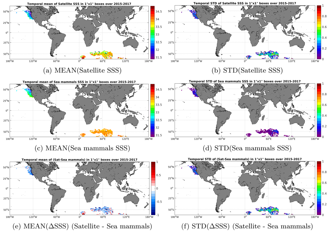
Figure 6: Temporal mean (left) and STD (right) of SSS from SMAP-L3-RSS-V2-8DAY-RUNNING-70KM (top), Sea mammals (middle), and of \Delta SSS (Satellite - Sea mammals). Only match-up pairs are used to generate these maps.
