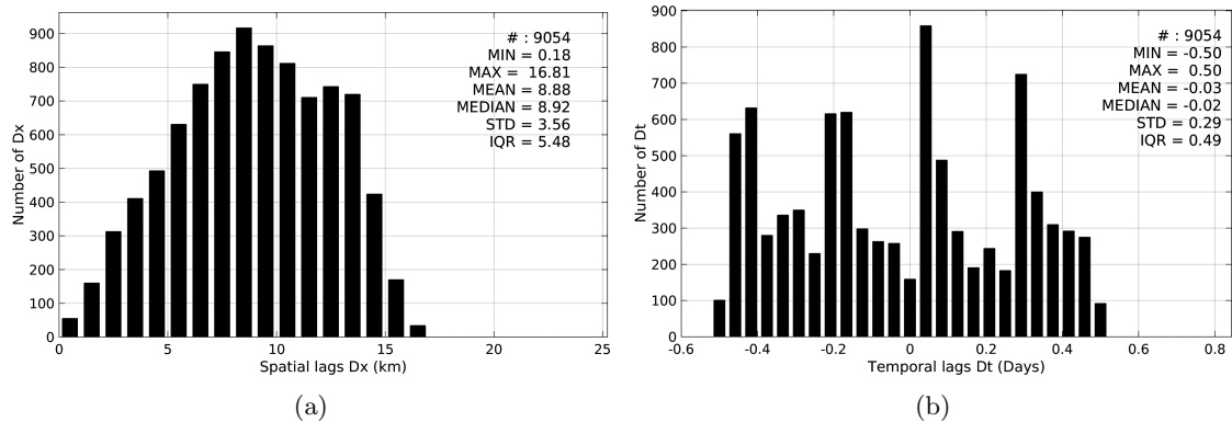
Figure 5: Histograms of the spatial (a) and temporal (b) lags between the time of the Sea mammals measurements and the date of the corresponding SMAP-L3-RSS-V2-8DAY-RUNNING-70KM SSS product.
