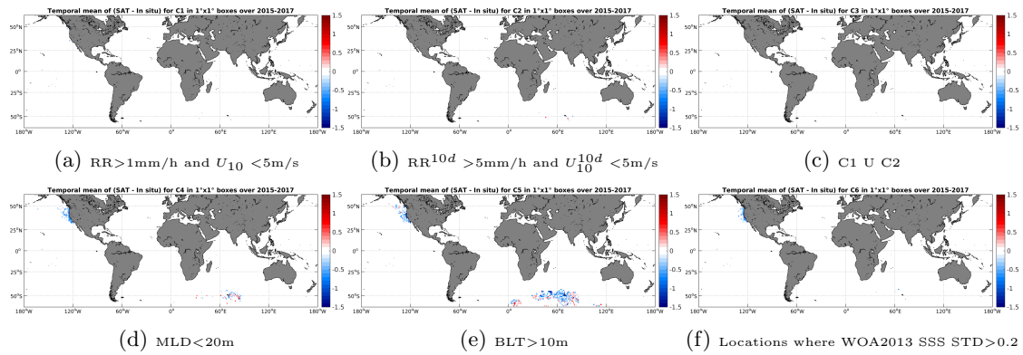
Figure 12: Temporal mean gridded over spatial boxes of size 1^\circ \times 1^\circ of \Delta SSS (SMAP-L3-RSS-V2-8DAY-RUNNING-70KM - Sea mammals) for 6 different subdatasets corresponding to:RR >1 mm/h and U_{10} < 5 m/s (a), RR^{10d} > 5 mm/h and U_{10}^{10d} < 5 m/s (b), C1 U C2 (c),MLD <20 m (d),BLT >10 m (e),Locations where WOA2013 SSS STD >0.2 (f).
