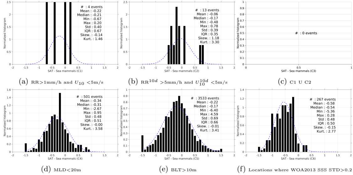
Figure 13: Normalized histogram of \Delta SSS (SMAP-L3-RSS-V2-8DAY-RUNNING-70KM - Sea mammals) for 6 different subdatasets corresponding to: RR>1mm/h and U_{10} < 5 m/s (a), RR^{10d} > 5 mm/h and U_{10}^{10d} < 5 m/s (b), C1 U C2 (c),MLD<20m (d),BLT>10m (e),Locations where WOA2013 SSS STD>0.2 (f).
