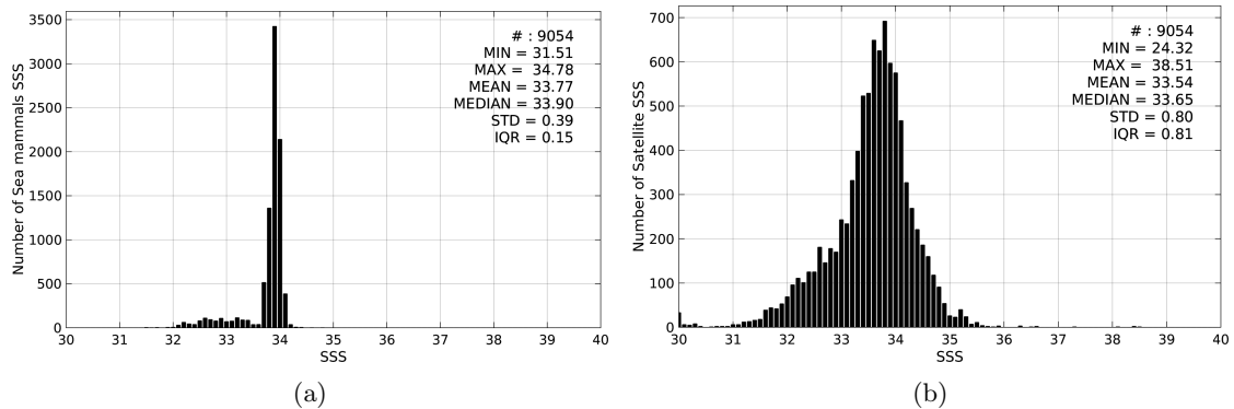
Figure 2: Histograms of SSS from Sea mammals (a) and SMAP-L3-RSS-V2-8DAY-RUNNING-70KM (b) considering all match-up pairs per bins of 0.1 over the SMOS coastal zone ( \approx 800 km) 60N-60S Pi-MEP region and for the full satellite product period.
