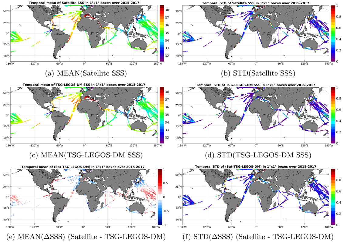
Figure 6: Temporal mean (left) and STD (right) of SSS from SMAP-L3-RSS-V2-MONTHLY-0.25DEG-40KM (top), TSG-LEGOS-DM (middle), and of \Delta SSS (Satellite - TSG-LEGOS-DM). Only match-up pairs are used to generate these maps.
