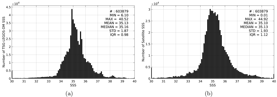
Figure 2: Histograms of SSS from TSG-LEGOS-DM (a) and SMAP-L3-RSS-V2-MONTHLY-0.25DEG-40KM (b) considering all match-up pairs per bins of 0.1 over the SMOS coastal zone ( \approx 800\text{km} ) 60N-60S Pi-MEP region and for the full satellite product period.
