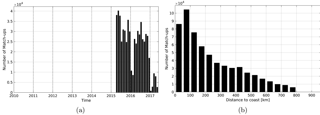
Figure 1: Number of match-ups between TSG-LEGOS-DM and SMAP-L3-RSS-V2-MONTHLY-0.25DEG-40KM SSS as a function of time (a) and as function of the distance to coast (b) over the SMOS coastal zone ( \approx 800\text{km} ) 60N-60S Pi-MEP region and for the full satellite product period.
