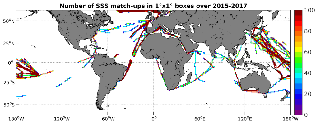
Figure 4: Number of SSS match-ups between TSG-LEGOS-DM SSS and the SMAP-L3-RSS-V2-MONTHLY-0.25DEG-40KM SSS product for the SMOS coastal zone ( \pm 800\text{km} ) 60N-60S Pi-MEP region over 1^\circ \times 1^\circ boxes and for the full satellite product period.
