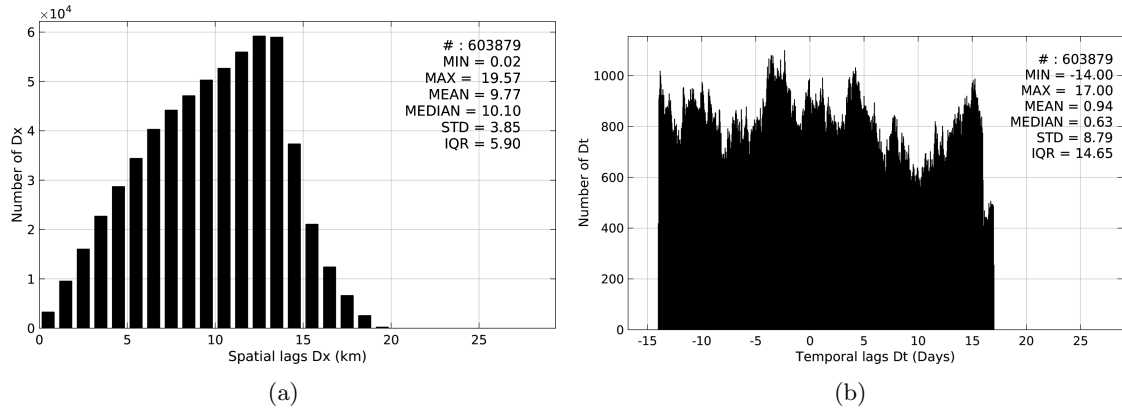
Figure 5: Histograms of the spatial (a) and temporal (b) lags between the time of the TSG-LEGOS-DM measurements and the date of the corresponding SMAP-L3-RSS-V2-MONTHLY-0.25DEG-40KM SSS product.
