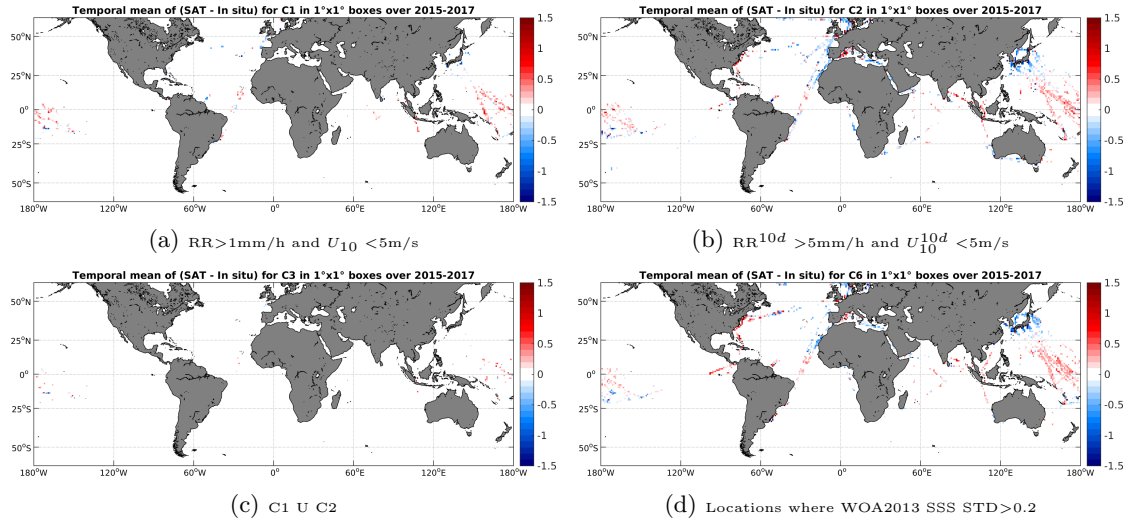
Figure 12: Temporal mean gridded over spatial boxes of size 1^\circ \times 1^\circ of \Delta SSS (SMAP-L3-RSS-V2-MONTHLY-0.25DEG-40KM - TSG-LEGOS-DM) for 4 different subdatasets corresponding to: RR > 1\text{mm/h} and U_{10} < 5\text{m/s} (a), RR^{10d} > 5\text{mm/h} and U_{10}^{10d} < 5\text{m/s} (b), C1 U C2 (c), Locations where WOA2013 SSS STD > 0.2 (d).
