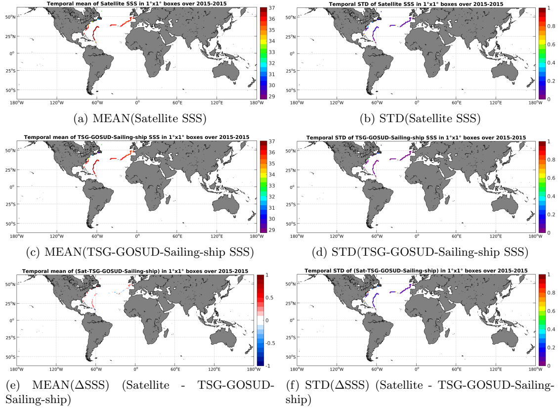
Figure 6: Temporal mean (left) and STD (right) of SSS from SMAP-L3-RSS-V2-MONTHLY-0.25DEG-40KM (top), TSG-GOSUD-Sailing-ship (middle), and of \Delta SSS (Satellite - TSG-GOSUD-Sailing-ship). Only match-up pairs are used to generate these maps.
