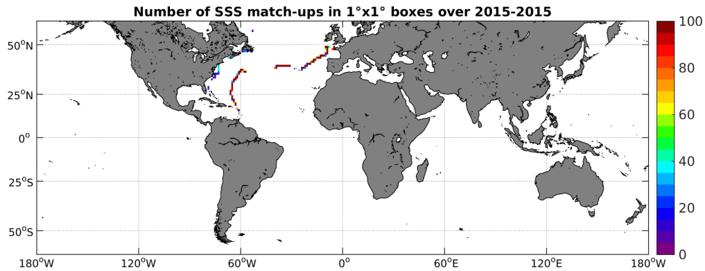
Figure 4: Number of SSS match-ups between TSG-GOSUD-Sailing-ship SSS and the SMAP-L3-RSS-V2-MONTHLY-0.25DEG-40KM SSS product for the SMOS coastal zone ( \pm 800\text{km} ) 60N-60S Pi-MEP region over 1^\circ \times 1^\circ boxes and for the full satellite product period.
