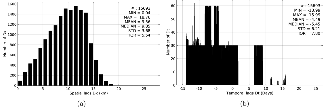
Figure 5: Histograms of the spatial (a) and temporal (b) lags between the time of the TSG-GOSUD-Sailing-ship measurements and the date of the corresponding SMAP-L3-RSS-V2-MONTHLY-0.25DEG-40KM SSS product.
