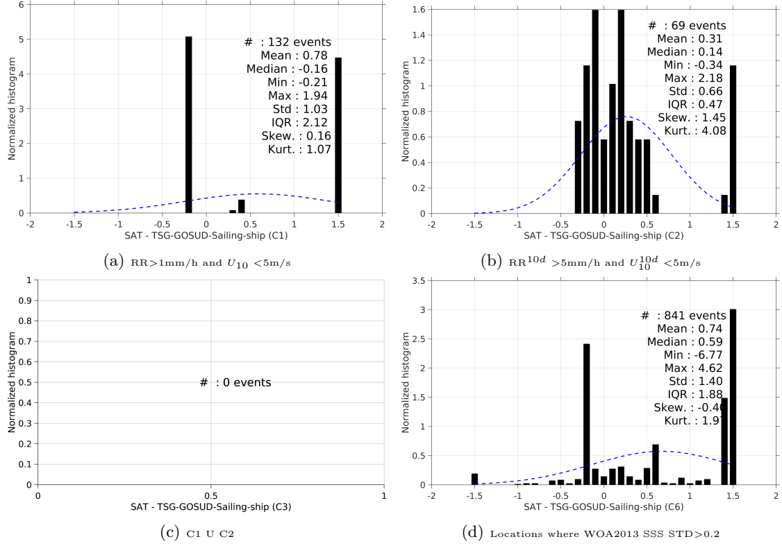
Figure 13: Normalized histogram of \Delta SSS (SMAP-L3-RSS-V2-MONTHLY-0.25DEG-40KM - TSG-GOSUD-Sailing-ship) for 6 different subdatasets corresponding to: RR > 1\text{mm/h} and U_{10} < 5\text{m/s} (a), RR^{10d} > 5\text{mm/h} and U_{10}^{10d} < 5\text{m/s} (b), C1 U C2 (c), Locations where WOA2013 SSS STD > 0.2 (d).
