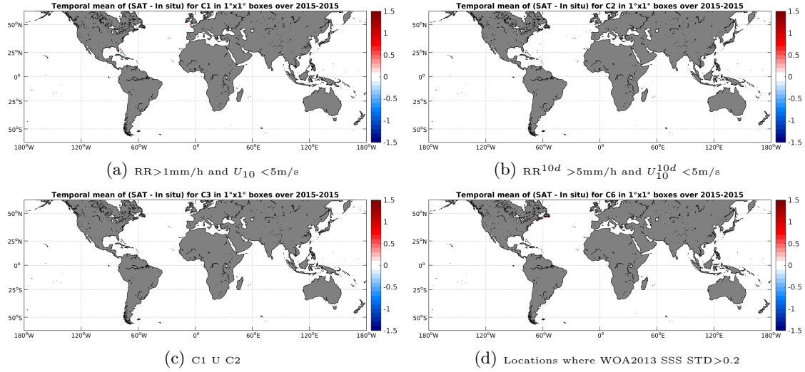
Figure 12: Temporal mean gridded over spatial boxes of size 1^\circ \times 1^\circ of \Delta SSS (SMAP-L3-RSS-V2-MONTHLY-0.25DEG-40KM - TSG-GOSUD-Sailing-ship) for 4 different subdatasets corresponding to: RR > 1\text{mm/h} and U_{10} < 5\text{m/s} (a), RR^{10d} > 5\text{mm/h} and U_{10}^{10d} < 5\text{m/s} (b), C1 U C2 (c), Locations where WOA2013 SSS STD > 0.2 (d).
