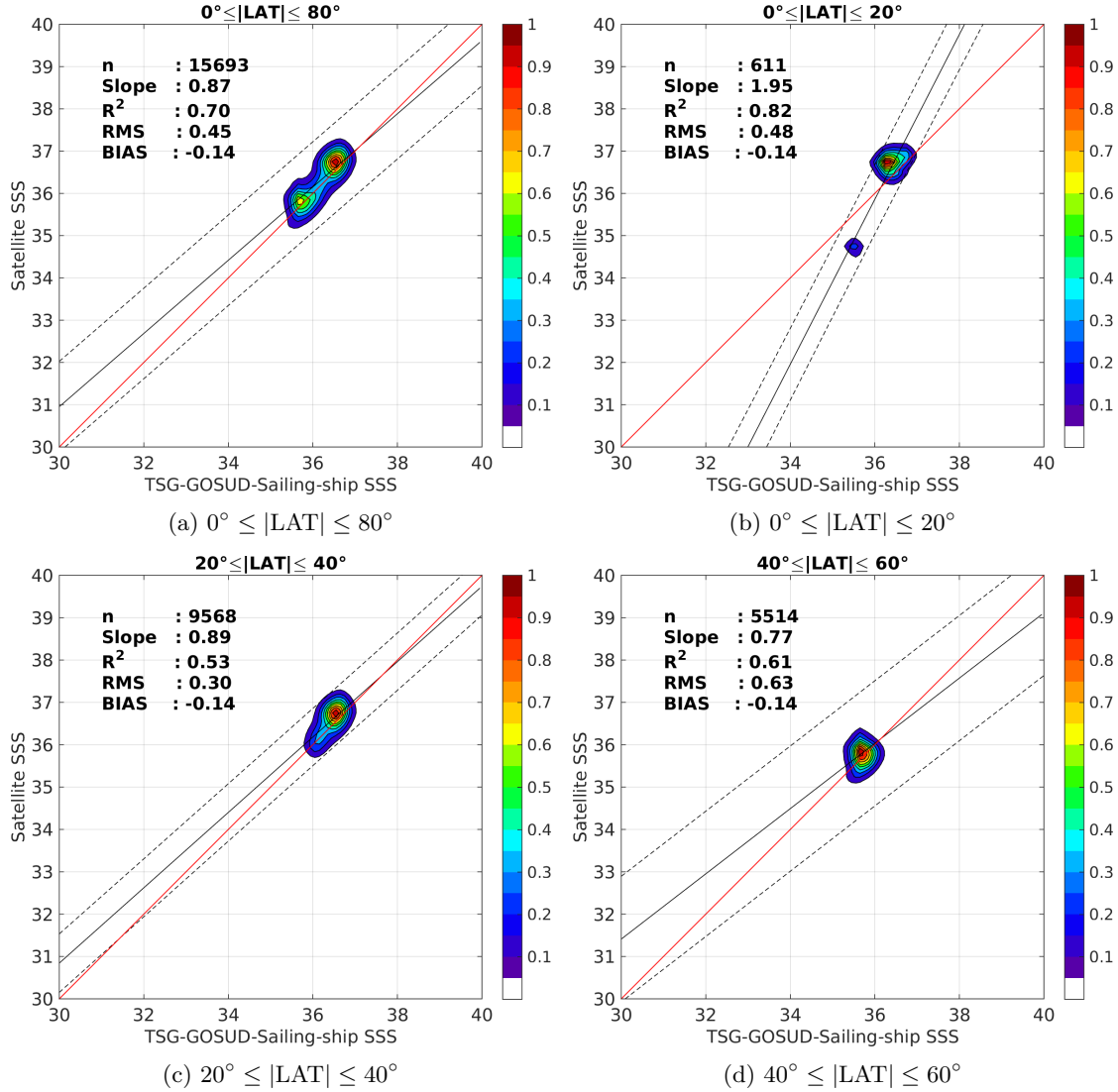
Figure 9: Contour maps of the concentration of SMAP-L3-RSS-V2-MONTHLY-0.25DEG-40KM SSS (y-axis) versus TSG-GOSUD-Sailing-ship SSS (x-axis) at match-up pairs for different latitude bands. For each plot, the red line shows x=y . The black thin and dashed lines indicate a linear fit through the data cloud and the \pm 95\% confidence levels, respectively. The number match-up pairs n , the slope and R^2 coefficient of the linear fit, the root mean square (RMS) and the mean bias between satellite and in situ data are indicated for each latitude band in each plots.
