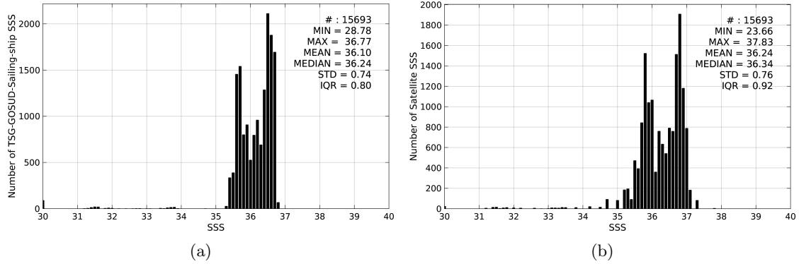
Figure 2: Histograms of SSS from TSG-GOSUD-Sailing-ship (a) and SMAP-L3-RSS-V2-MONTHLY-0.25DEG-40KM (b) considering all match-up pairs per bins of 0.1 over the SMOS coastal zone ( \geq 800 km) 60N-60S Pi-MEP region and for the full satellite product period.
