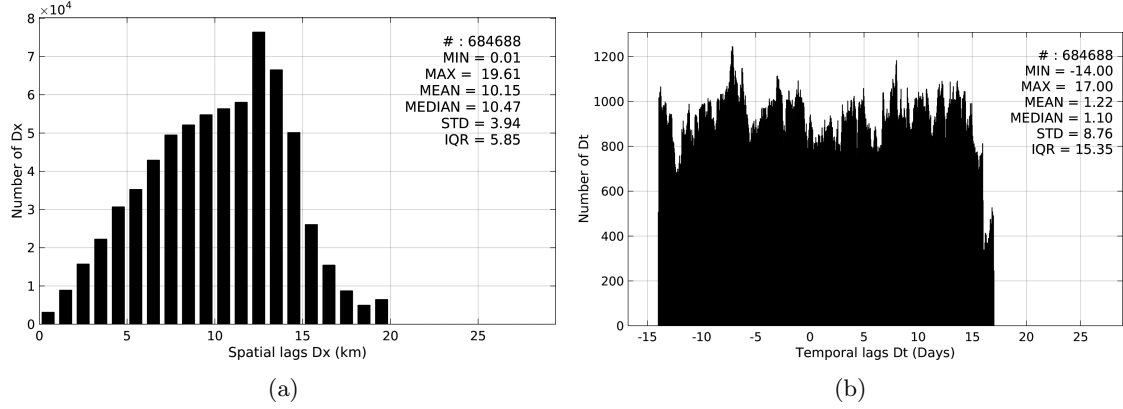
Figure 5: Histograms of the spatial (a) and temporal (b) lags between the time of the TSG-GOSUD-Research-vessel measurements and the date of the corresponding SMAP-L3-RSS-V2-MONTHLY-0.25DEG-40KM SSS product.
