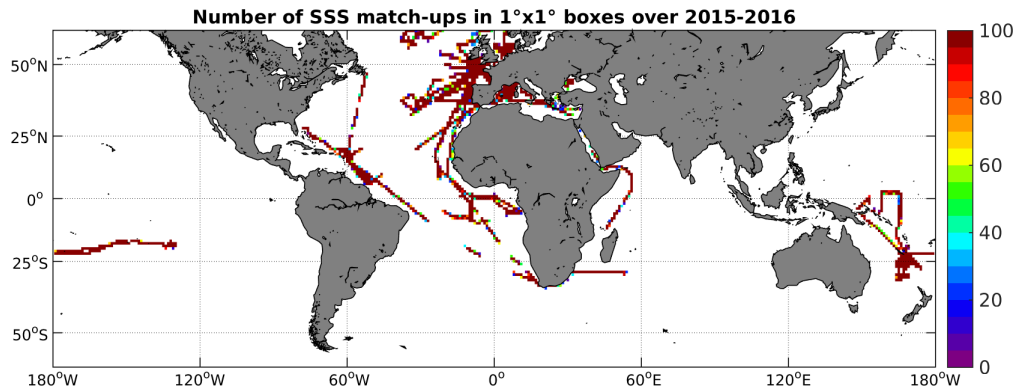
Figure 4: Number of SSS match-ups between TSG-GOSUD-Research-vessel SSS and the SMAP-L3-RSS-V2-MONTHLY-0.25DEG-40KM SSS product for the SMOS coastal zone ( \geq 800\text{km} ) 60^\circ\text{N} - 60^\circ\text{S} Pi-MEP region over 1^\circ \times 1^\circ boxes and for the full satellite product period.
