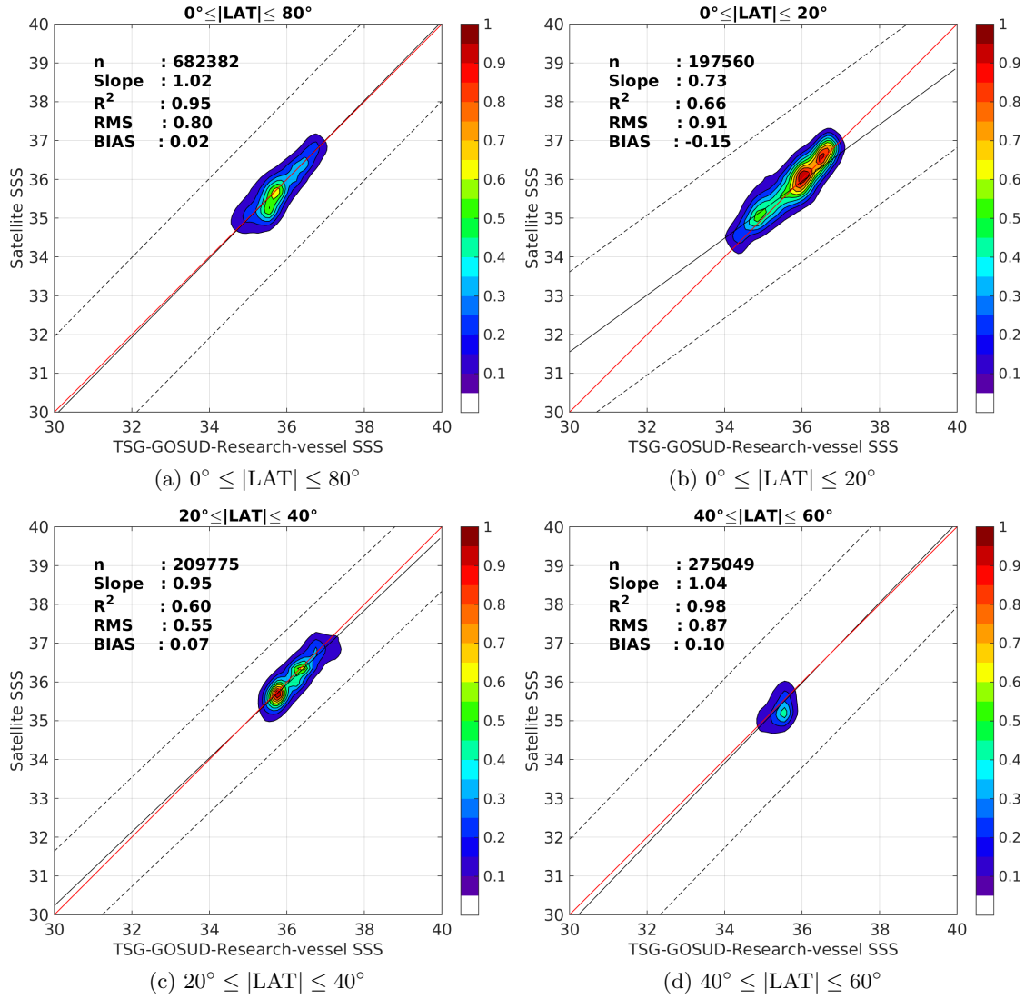
Figure 9: Contour maps of the concentration of SMAP-L3-RSS-V2-MONTHLY-0.25DEG-40KM SSS (y-axis) versus TSG-GOSUD-Research-vessel SSS (x-axis) at match-up pairs for different latitude bands. For each plot, the red line shows x=y . The black thin and dashed lines indicate a linear fit through the data cloud and the \pm 95\% confidence levels, respectively. The number match-up pairs n , the slope and R^2 coefficient of the linear fit, the root mean square (RMS) and the mean bias between satellite and in situ data are indicated for each latitude band in each plots.
