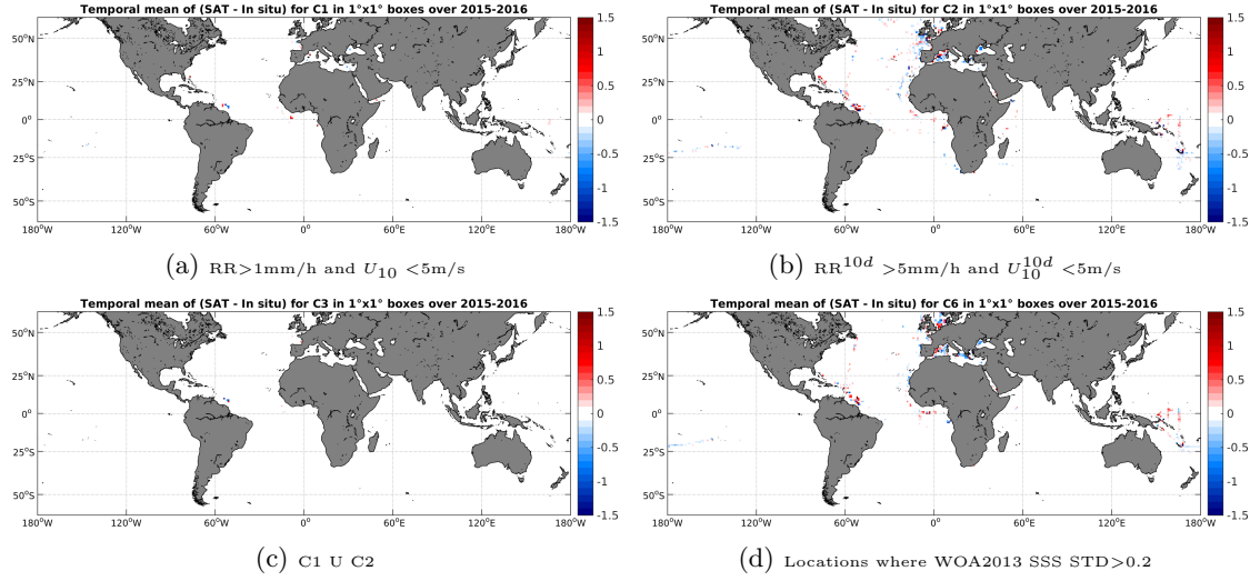
Figure 12: Temporal mean gridded over spatial boxes of size 1^\circ \times 1^\circ of \Delta SSS (SMAP-L3-RSS-V2-MONTHLY-0.25DEG-40KM - TSG-GOSUD-Research-vessel) for 4 different subdatasets corresponding to: RR > 1mm/h and U_{10} < 5 m/s (a), RR^{10d} > 5 mm/h and U_{10}^{10d} < 5 m/s (b), C1 U C2 (c), Locations where WOA2013 SSS STD > 0.2 (d).
