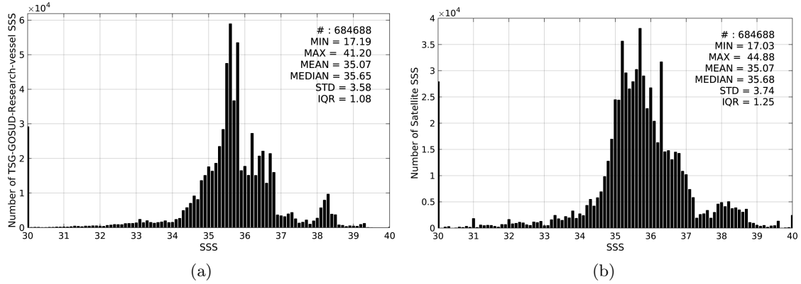
Figure 2: Histograms of SSS from TSG-GOSUD-Research-vessel (a) and SMAP-L3-RSS-V2-MONTHLY-0.25DEG-40KM (b) considering all match-up pairs per bins of 0.1 over the SMOS coastal zone ( \pm 800\text{km} ) 60N-60S Pi-MEP region and for the full satellite product period.
