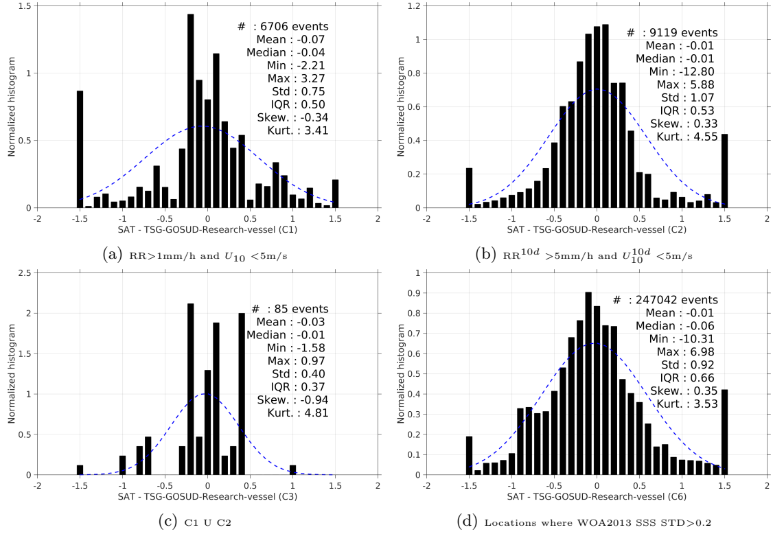
Figure 13: Normalized histogram of \Delta SSS (SMAP-L3-RSS-V2-MONTHLY-0.25DEG-40KM - TSG-GOSUD-Research-vessel) for 6 different subdatasets corresponding to: RR > 1\text{mm/h} and U_{10} < 5\text{m/s} (a), RR^{10d} > 5\text{mm/h} and U_{10}^{10d} < 5\text{m/s} (b), C1 \cup C2 (c), Locations where WOA2013 SSS STD > 0.2 (d).
