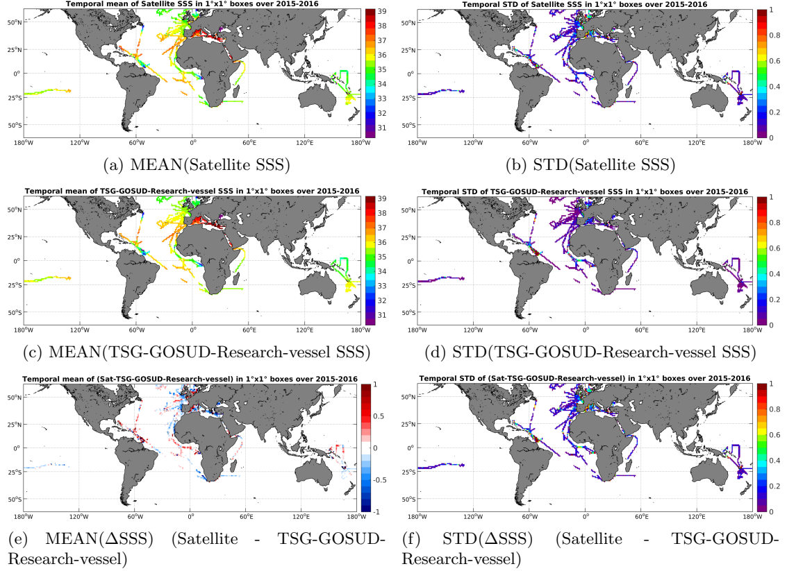
Figure 6: Temporal mean (left) and STD (right) of SSS from SMAP-L3-RSS-V2-MONTHLY-0.25DEG-40KM (top), TSG-GOSUD-Research-vessel (middle), and of \Delta SSS (Satellite - TSG-GOSUD-Research-vessel). Only match-up pairs are used to generate these maps.
