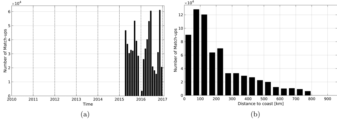
Figure 1: Number of match-ups between TSG-GOSUD-Research-vessel and SMAP-L3-RSS-V2-MONTHLY-0.25DEG-40KM SSS as a function of time (a) and as function of the distance to coast (b) over the SMOS coastal zone ( \pm 800\text{km} ) 60N-60S Pi-MEP region and for the full satellite product period.
