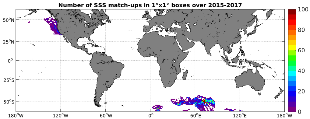
Figure 4: Number of SSS match-ups between Sea mammals SSS and the SMAP-L3-RSS-V2-MONTHLY-0.25DEG-40KM SSS product for the SMOS coastal zone ( \pm 800\text{km} ) 60N-60S Pi-MEP region over 1^\circ \times 1^\circ boxes and for the full satellite product period.
