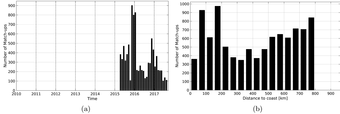
Figure 1: Number of match-ups between Sea mammals and SMAP-L3-RSS-V2-MONTHLY-0.25DEG-40KM SSS as a function of time (a) and as function of the distance to coast (b) over the SMOS coastal zone ( \pm 800\text{km} ) 60N-60S Pi-MEP region and for the full satellite product period.
