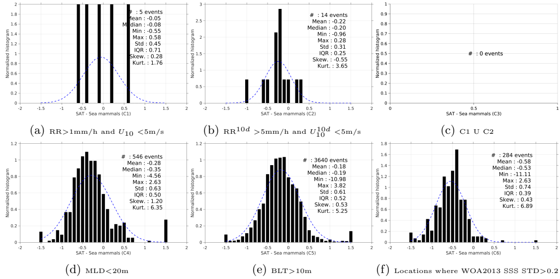
Figure 13: Normalized histogram of \Delta SSS (SMAP-L3-RSS-V2-MONTHLY-0.25DEG-40KM - Sea mammals) for 6 different subdatasets corresponding to: RR>1mm/h and U_{10} < 5\text{m/s} (a), RR^{10d} > 5\text{mm/h} and U_{10}^{10d} < 5\text{m/s} (b), C1 U C2 (c), MLD<20m (d), BLT>10m (e), Locations where WOA2013 SSS STD>0.2 (f).
