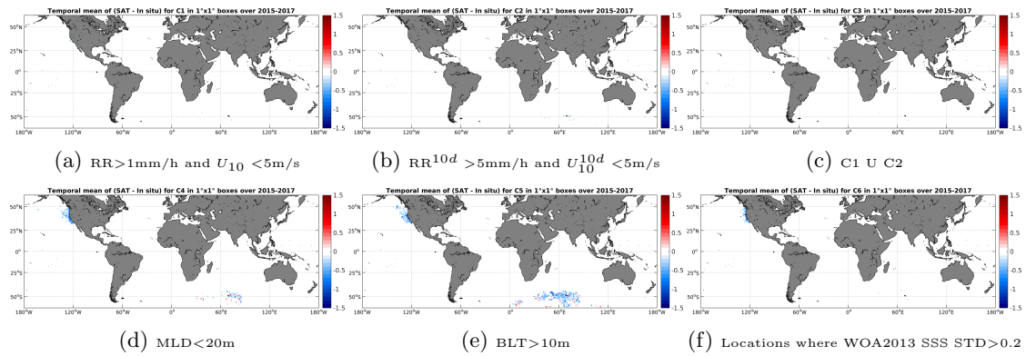
Figure 12: Temporal mean gridded over spatial boxes of size 1^\circ \times 1^\circ of \Delta SSS (SMAP-L3-RSS-V2-MONTHLY-0.25DEG-40KM - Sea mammals) for 6 different subdatasets corresponding to: RR > 1 mm/h and U_{10} < 5 m/s (a), RR^{10d} > 5 mm/h and U_{10}^{10d} < 5 m/s (b), C1 U C2 (c), MLD < 20m (d), BLT > 10m (e), Locations where WOA2013 SSS STD > 0.2 (f).
