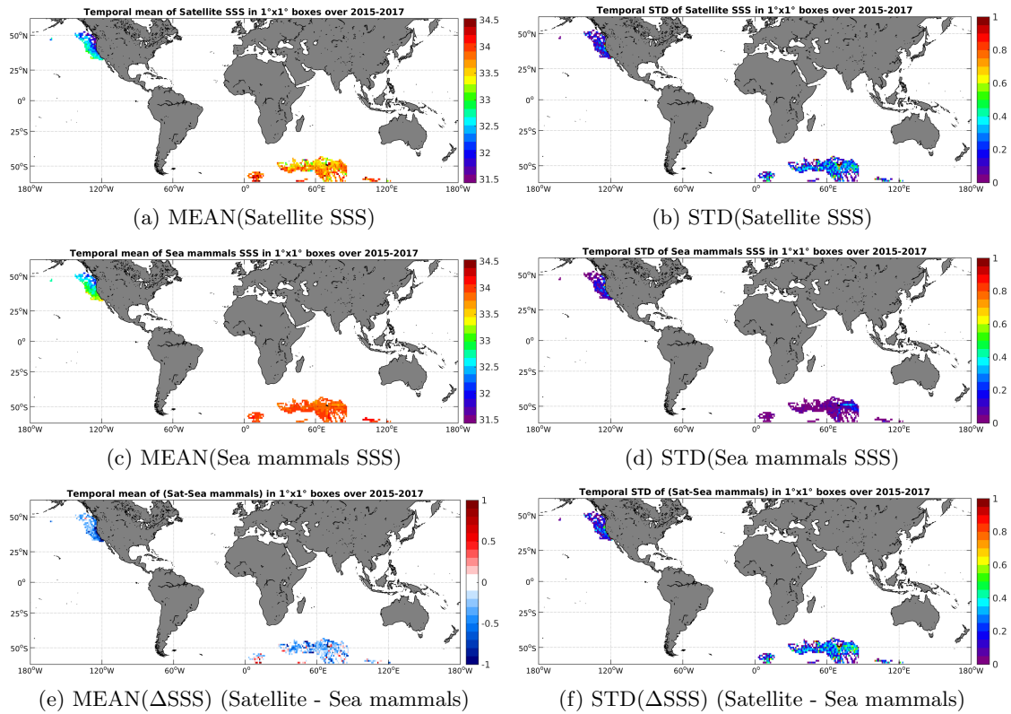
Figure 6: Temporal mean (left) and STD (right) of SSS from SMAP-L3-RSS-V2-MONTHLY-0.25DEG-40KM (top), Sea mammals (middle), and of \Delta SSS (Satellite - Sea mammals). Only match-up pairs are used to generate these maps.
