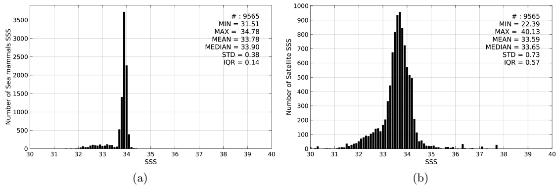
Figure 2: Histograms of SSS from Sea mammals (a) and SMAP-L3-RSS-V2-MONTHLY-0.25DEG-40KM (b) considering all match-up pairs per bins of 0.1 over the SMOS coastal zone ( \pm 800\text{km} ) 60N-60S Pi-MEP region and for the full satellite product period.
