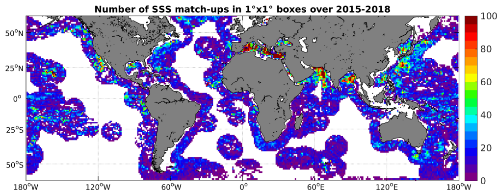
Figure 4: Number of SSS match-ups between Argo SSS and the SMAP-L3-RSS-V2-MONTHLY-0.25DEG-40KM SSS product for the SMOS coastal zone ( \approx 800\text{km} ) 60N-60S Pi-MEP region over 1^\circ \times 1^\circ boxes and for the full satellite product period.
