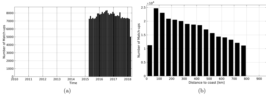
Figure 1: Number of match-ups between Argo and SMAP-L3-RSS-V2-MONTHLY-0.25DEG-40KM SSS as a function of time (a) and as function of the distance to coast (b) over the SMOS coastal zone ( \leq 800 km) 60N-60S Pi-MEP region and for the full satellite product period.
