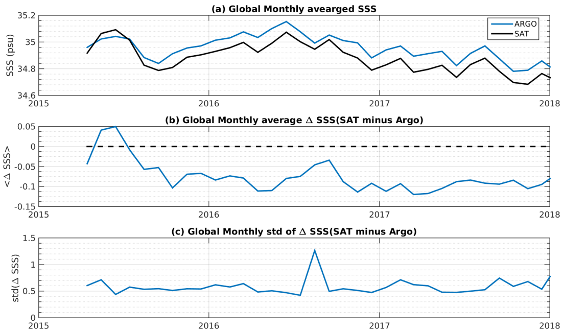
Figure 7: Time series of the monthly averaged mean SSS (top), mean \Delta SSS (Satellite - Argo) and STD of \Delta SSS (Satellite - Argo) over the SMOS coastal zone ( \geq 800 km) 60N-60S Pi-MEP region considering all match-ups collected by the Pi-MEP platform.
