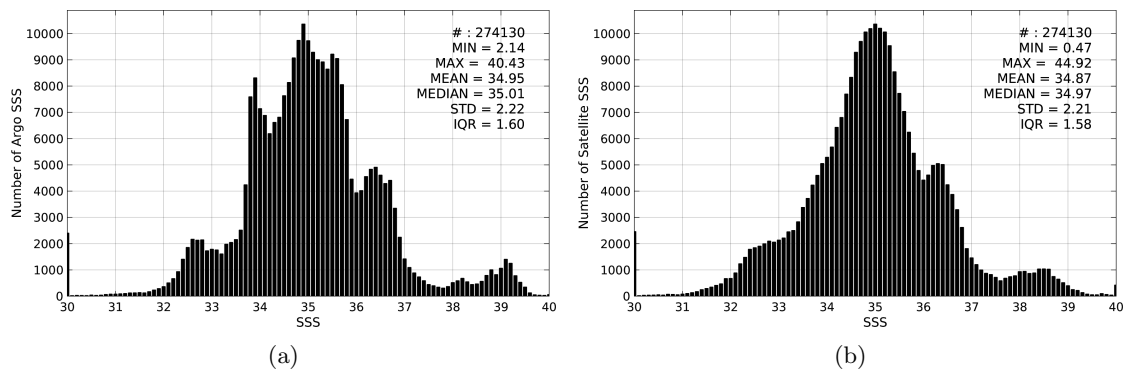
Figure 2: Histograms of SSS from Argo (a) and SMAP-L3-RSS-V2-MONTHLY-0.25DEG-40KM (b) considering all match-up pairs per bins of 0.1 over the SMOS coastal zone ( \leq 800 km) 60N-60S Pi-MEP region and for the full satellite product period.
