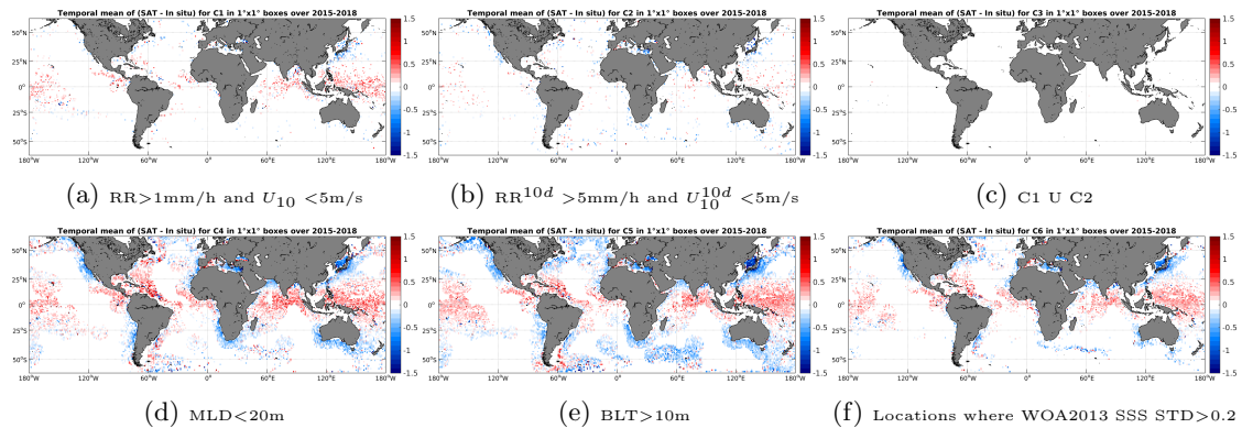
Figure 12: Temporal mean gridded over spatial boxes of size 1^\circ \times 1^\circ of \Delta SSS (SMAP-L3-RSS-V2-MONTHLY-0.25DEG-40KM - Argo) for 6 different subdatasets corresponding to: RR > 1 mm/h and U_{10} < 5 m/s (a), RR^{10d} > 5 mm/h and U_{10}^{10d} < 5 m/s (b), C1 U C2 (c), MLD < 20 m (d), BLT > 10 m (e), Locations where WOA2013 SSS STD > 0.2 (f).
