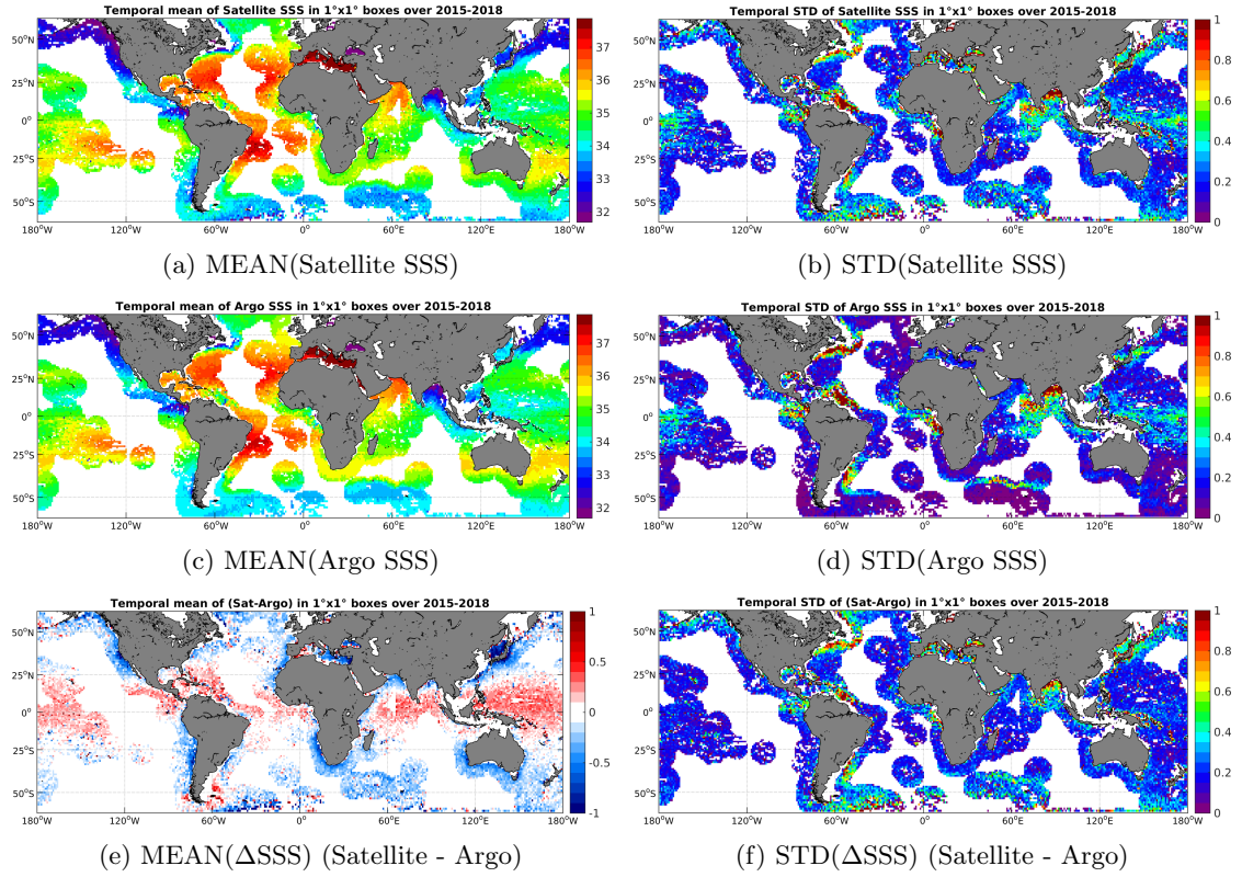
Figure 6: Temporal mean (left) and STD (right) of SSS from SMAP-L3-RSS-V2-MONTHLY-0.25DEG-40KM (top), Argo (middle), and of \Delta SSS (Satellite - Argo). Only match-up pairs are used to generate these maps.
