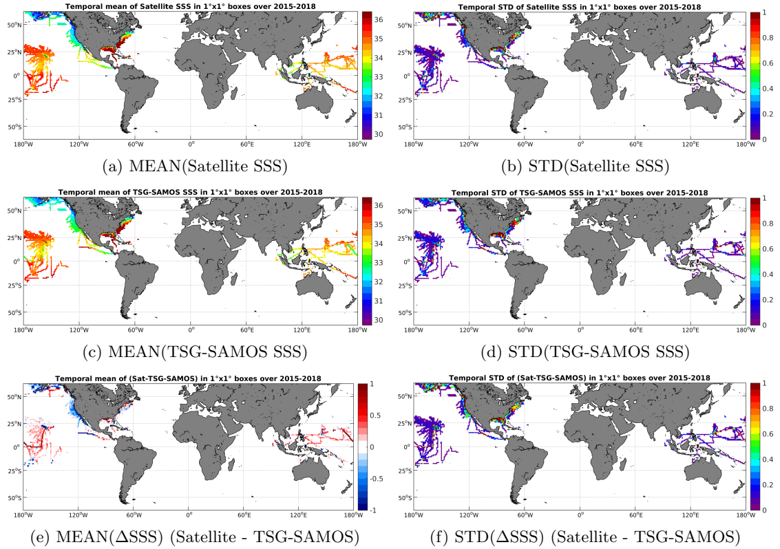
Figure 6: Temporal mean (left) and STD (right) of SSS from SMAP-L3-RSS-V2-MONTHLY-70KM (top), TSG-SAMOS (middle), and of \Delta SSS (Satellite - TSG-SAMOS). Only match-up pairs are used to generate these maps.
