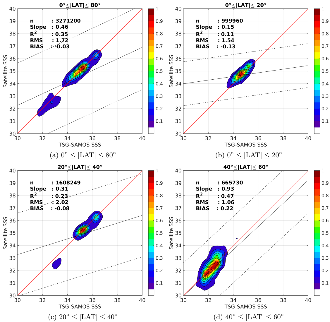
Figure 9: Contour maps of the concentration of SMAP-L3-RSS-V2-MONTHLY-70KM SSS (y-axis) versus TSG-SAMOS SSS (x-axis) at match-up pairs for different latitude bands. For each plot, the red line shows x=y . The black thin and dashed lines indicate a linear fit through the data cloud and the \pm 95\% confidence levels, respectively. The number match-up pairs n , the slope and R^2 coefficient of the linear fit, the root mean square (RMS) and the mean bias between satellite and in situ data are indicated for each latitude band in each plots.
