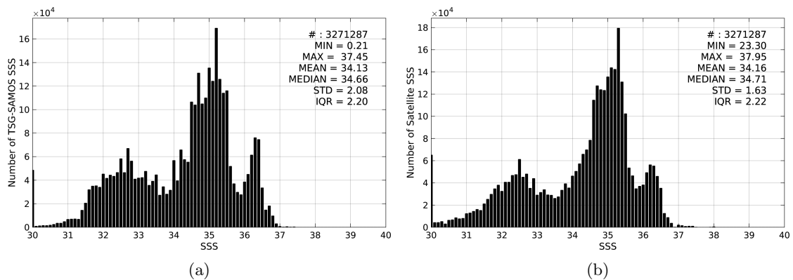
Figure 2: Histograms of SSS from TSG-SAMOS (a) and SMAP-L3-RSS-V2-MONTHLY-70KM (b) considering all match-up pairs per bins of 0.1 over the SMOS coastal zone ( \approx 800\text{km} ) 60N-60S Pi-MEP region and for the full satellite product period.
