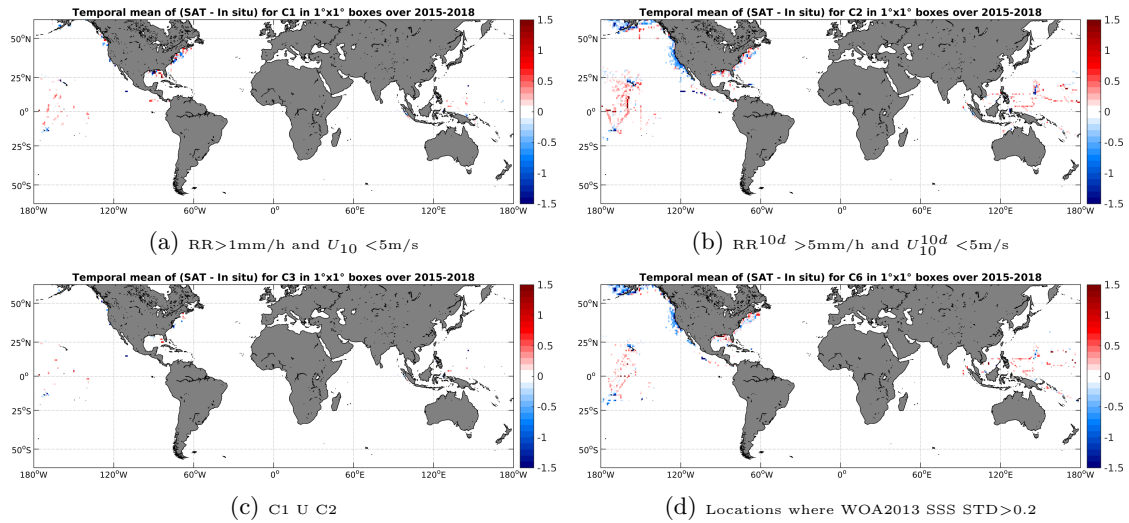
Figure 12: Temporal mean gridded over spatial boxes of size 1^\circ \times 1^\circ of \Delta SSS (SMAP-L3-RSS-V2-MONTHLY-70KM - TSG-SAMOS) for 4 different subdatasets corresponding to: RR > 1\text{mm/h} and U_{10} < 5\text{m/s} (a), RR^{10d} > 5\text{mm/h} and U_{10}^{10d} < 5\text{m/s} (b), C1 U C2 (c), Locations where WOA2013 SSS STD > 0.2 (d).
