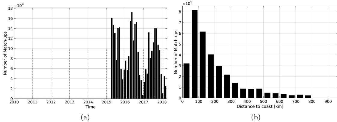
Figure 1: Number of match-ups between TSG-SAMOS and SMAP-L3-RSS-V2-MONTHLY-70KM SSS as a function of time (a) and as function of the distance to coast (b) over the SMOS coastal zone ( \approx 800\text{km} ) 60N-60S Pi-MEP region and for the full satellite product period.
