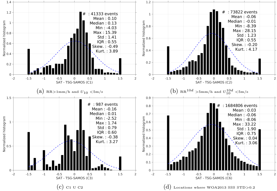
Figure 13: Normalized histogram of \Delta\text{SSS} (SMAP-L3-RSS-V2-MONTHLY-70KM - TSG-SAMOS) for 6 different subdatasets corresponding to: RR>1mm/h and U_{10} < 5\text{m/s} (a), RR^{10d} > 5\text{mm/h} and U_{10}^{10d} < 5\text{m/s} (b), C1 U C2 (c), Locations where WOA2013 SSS STD>0.2 (d).
