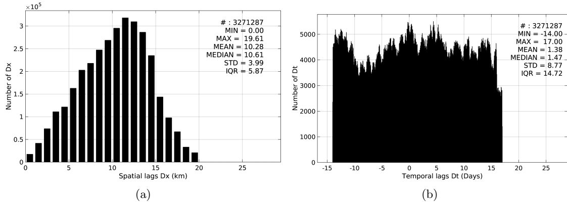
Figure 5: Histograms of the spatial (a) and temporal (b) lags between the time of the TSG-SAMOS measurements and the date of the corresponding SMAP-L3-RSS-V2-MONTHLY-70KM SSS product.
