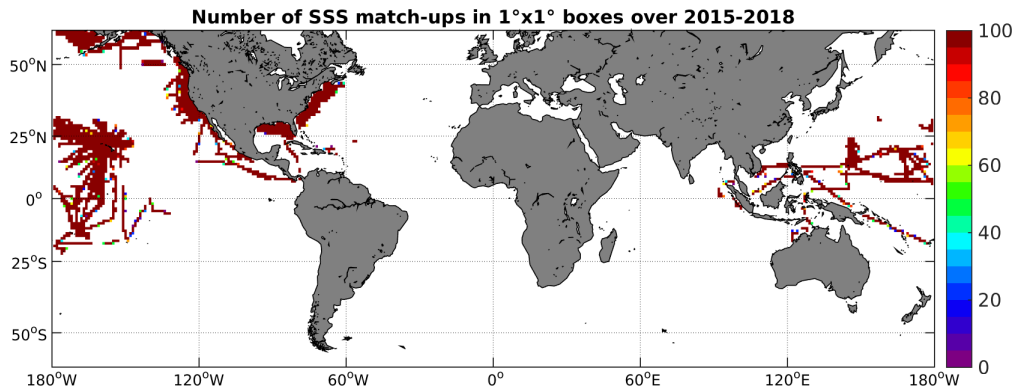
Figure 4: Number of SSS match-ups between TSG-SAMOS SSS and the SMAP-L3-RSS-V2-MONTHLY-70KM SSS product for the SMOS coastal zone ( \approx 800\text{km} ) 60N-60S Pi-MEP region over 1^\circ \times 1^\circ boxes and for the full satellite product period.
