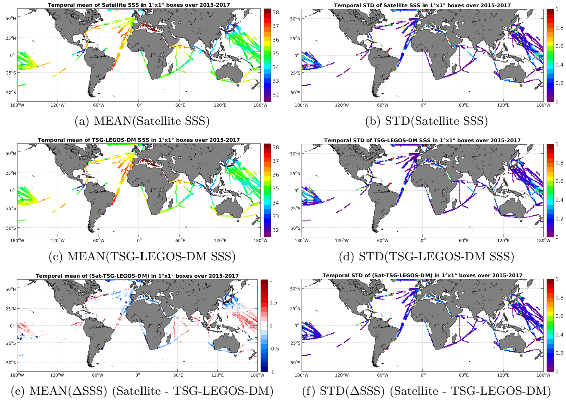
Figure 6: Temporal mean (left) and STD (right) of SSS from SMAP-L3-RSS-V2-MONTHLY-70KM (top), TSG-LEGOS-DM (middle), and of \Delta SSS (Satellite - TSG-LEGOS-DM). Only match-up pairs are used to generate these maps.
