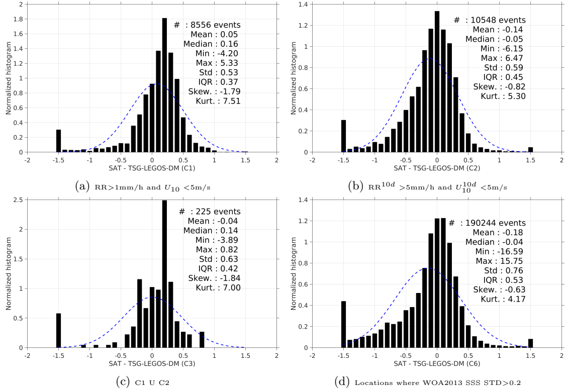
Figure 13: Normalized histogram of \Delta\text{SSS} (SMAP-L3-RSS-V2-MONTHLY-70KM - TSG-LEGOS-DM) for 6 different subdatasets corresponding to: RR > 1mm/h and U_{10} < 5\text{m/s} (a), \text{RR}^{10d} > 5\text{mm/h} and U_{10}^{10d} < 5\text{m/s} (b), C1 U C2 (c), Locations where WOA2013 SSS STD > 0.2 (d).
