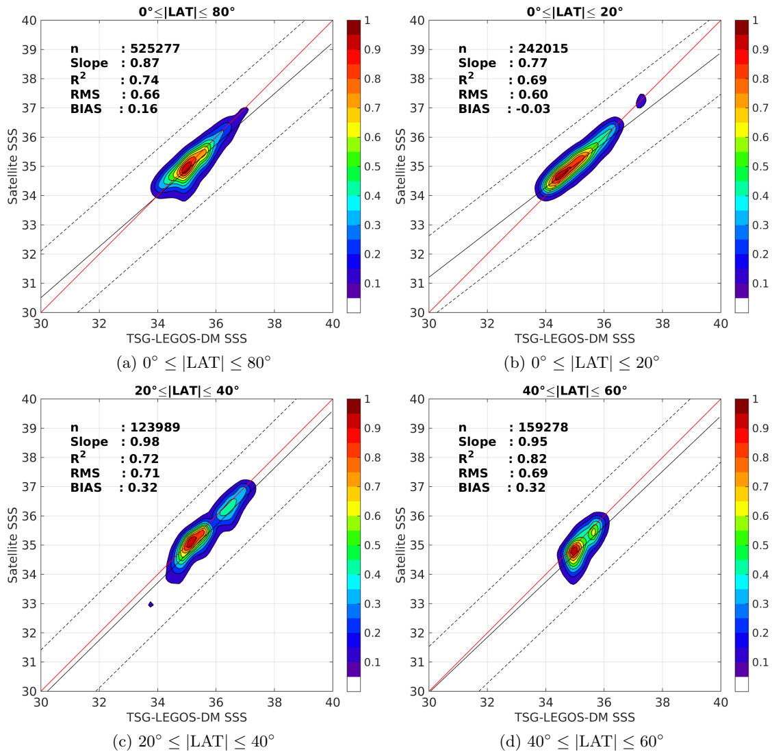
Figure 9: Contour maps of the concentration of SMAP-L3-RSS-V2-MONTHLY-70KM SSS (y-axis) versus TSG-LEGOS-DM SSS (x-axis) at match-up pairs for different latitude bands. For each plot, the red line shows x=y . The black thin and dashed lines indicate a linear fit through the data cloud and the \pm 95\% confidence levels, respectively. The number match-up pairs n , the slope and R^2 coefficient of the linear fit, the root mean square (RMS) and the mean bias between satellite and in situ data are indicated for each latitude band in each plots.
