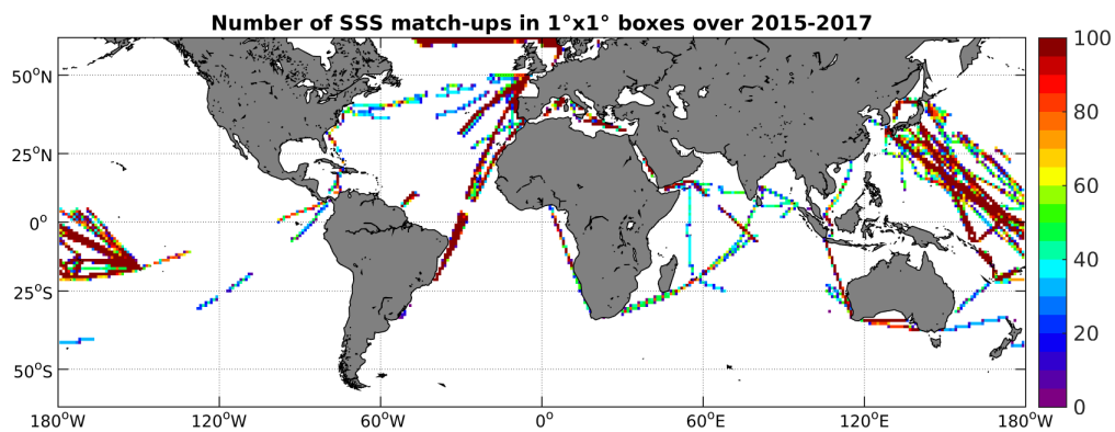
Figure 4: Number of SSS match-ups between TSG-LEGOS-DM SSS and the SMAP-L3-RSS-V2-MONTHLY-70KM SSS product for the SMOS coastal zone ( \approx 800\text{km} ) 60N-60S Pi-MEP region over 1^\circ \times 1^\circ boxes and for the full satellite product period.
