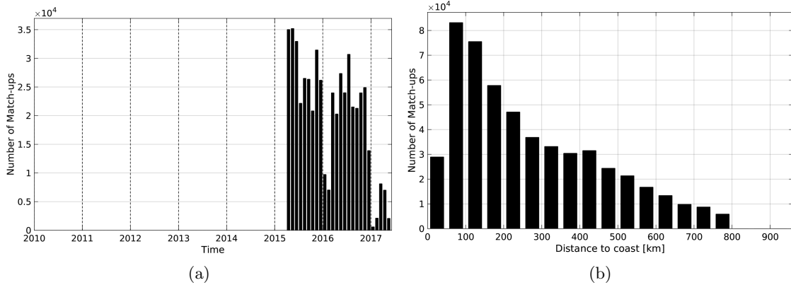
Figure 1: Number of match-ups between TSG-LEGOS-DM and SMAP-L3-RSS-V2-MONTHLY-70KM SSS as a function of time (a) and as function of the distance to coast (b) over the SMOS coastal zone ( \approx 800 km) 60N-60S Pi-MEP region and for the full satellite product period.
