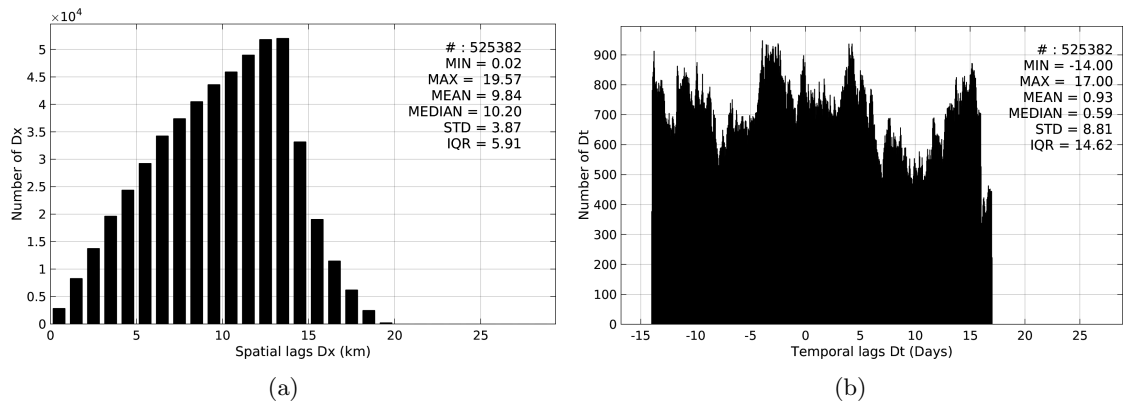
Figure 5: Histograms of the spatial (a) and temporal (b) lags between the time of the TSG-LEGOS-DM measurements and the date of the corresponding SMAP-L3-RSS-V2-MONTHLY-70KM SSS product.
