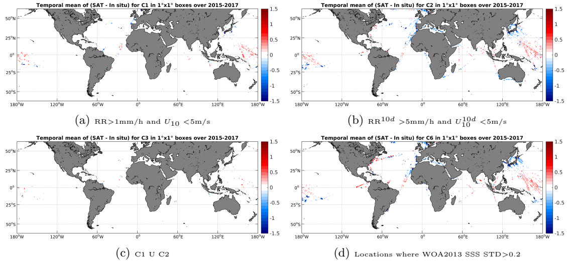
Figure 12: Temporal mean gridded over spatial boxes of size 1^\circ \times 1^\circ of \Delta SSS (SMAP-L3-RSS-V2-MONTHLY-70KM - TSG-LEGOS-DM) for 4 different subdatasets corresponding to: RR > 1\text{mm/h} and U_{10} < 5\text{m/s} (a), RR^{10d} > 5\text{mm/h} and U_{10}^{10d} < 5\text{m/s} (b), C1 U C2 (c), Locations where WOA2013 SSS STD > 0.2 (d).
