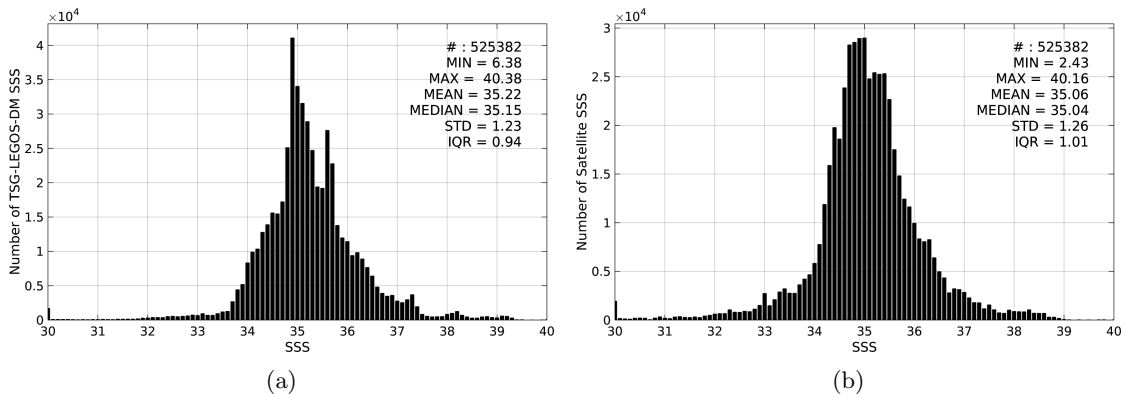
Figure 2: Histograms of SSS from TSG-LEGOS-DM (a) and SMAP-L3-RSS-V2-MONTHLY-70KM (b) considering all match-up pairs per bins of 0.1 over the SMOS coastal zone ( \approx 800 km) 60N-60S Pi-MEP region and for the full satellite product period.
