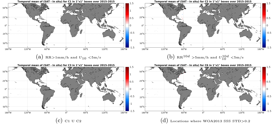
Figure 12: Temporal mean gridded over spatial boxes of size 1^\circ \times 1^\circ of \Delta SSS (SMAP-L3-RSS-V2-MONTHLY-70KM - TSG-GOSUD-Sailing-ship) for 4 different subdatasets corresponding to: RR > 1mm/h and U_{10} < 5 m/s (a), RR^{10d} > 5 mm/h and U_{10}^{10d} < 5 m/s (b), C1 U C2 (c), Locations where WOA2013 SSS STD > 0.2 (d).
