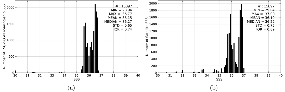
Figure 2: Histograms of SSS from TSG-GOSUD-Sailing-ship (a) and SMAP-L3-RSS-V2-MONTHLY-70KM (b) considering all match-up pairs per bins of 0.1 over the SMOS coastal zone ( \geq 800 km) 60N-60S Pi-MEP region and for the full satellite product period.
