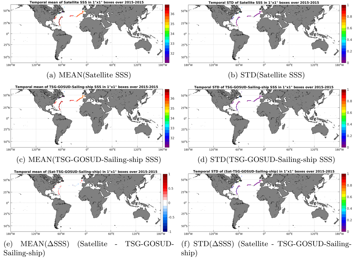
Figure 6: Temporal mean (left) and STD (right) of SSS from SMAP-L3-RSS-V2-MONTHLY-70KM (top), TSG-GOSUD-Sailing-ship (middle), and of \Delta SSS (Satellite - TSG-GOSUD-Sailing-ship). Only match-up pairs are used to generate these maps.
