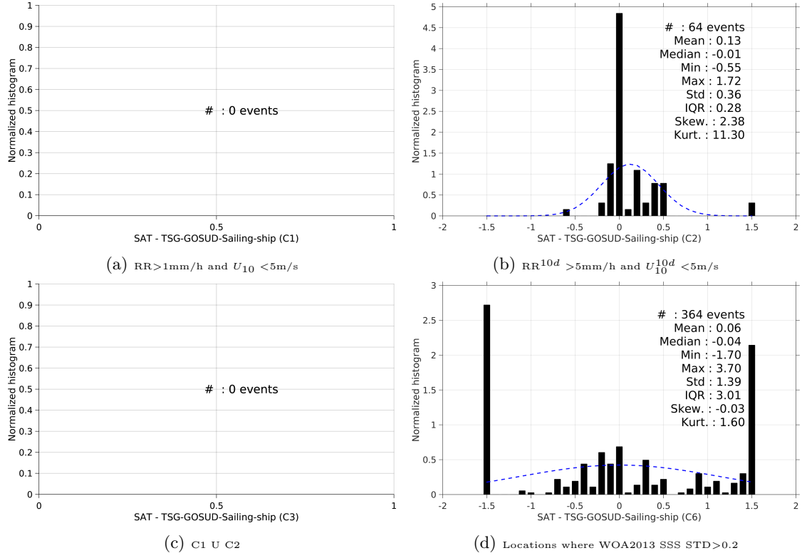
Figure 13: Normalized histogram of \Delta SSS (SMAP-L3-RSS-V2-MONTHLY-70KM - TSG-GOSUD-Sailing-ship) for 6 different subdatasets corresponding to: RR > 1\text{mm/h} and U_{10} < 5\text{m/s} (a), RR^{10d} > 5\text{mm/h} and U_{10}^{10d} < 5\text{m/s} (b), C1 \cup C2 (c), Locations where WOA2013 SSS STD > 0.2 (d).
