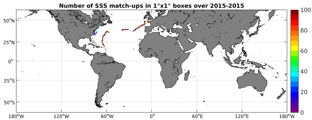
Figure 4: Number of SSS match-ups between TSG-GOSUD-Sailing-ship SSS and the SMAP-L3-RSS-V2-MONTHLY-70KM SSS product for the SMOS coastal zone ( \pm 800\text{km} ) 60N-60S Pi-MEP region over 1^\circ \times 1^\circ boxes and for the full satellite product period.
