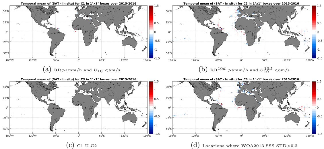
Figure 12: Temporal mean gridded over spatial boxes of size 1^\circ \times 1^\circ of \Delta SSS (SMAP-L3-RSS-V2-MONTHLY-70KM - TSG-GOSUD-Research-vessel) for 4 different subdatasets corresponding to: RR > 1\text{mm/h} and U_{10} < 5\text{m/s} (a), RR^{10d} > 5\text{mm/h} and U_{10}^{10d} < 5\text{m/s} (b), C1 U C2 (c), Locations where WOA2013 SSS STD > 0.2 (d).
