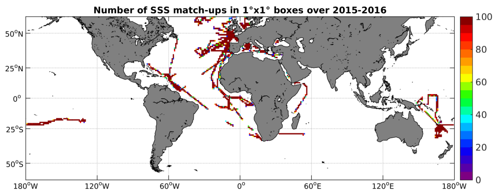
Figure 4: Number of SSS match-ups between TSG-GOSUD-Research-vessel SSS and the SMAP-L3-RSS-V2-MONTHLY-70KM SSS product for the SMOS coastal zone ( \pm 800 km) 60N-60S Pi-MEP region over 1^\circ \times 1^\circ boxes and for the full satellite product period.
