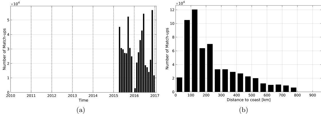
Figure 1: Number of match-ups between TSG-GOSUD-Research-vessel and SMAP-L3-RSS-V2-MONTHLY-70KM SSS as a function of time (a) and as function of the distance to coast (b) over the SMOS coastal zone ( \approx 800 km) 60N-60S Pi-MEP region and for the full satellite product period.
