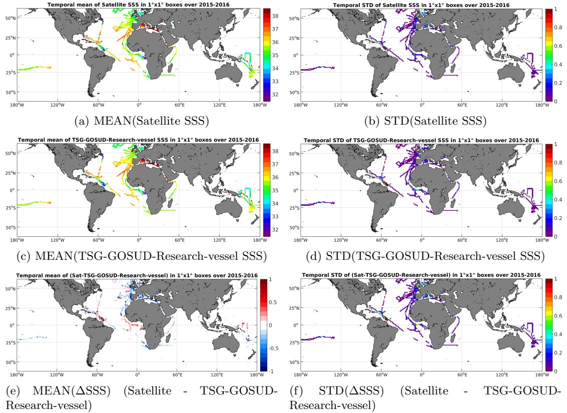
Figure 6: Temporal mean (left) and STD (right) of SSS from SMAP-L3-RSS-V2-MONTHLY-70KM (top), TSG-GOSUD-Research-vessel (middle), and of \Delta SSS (Satellite - TSG-GOSUD-Research-vessel). Only match-up pairs are used to generate these maps.
