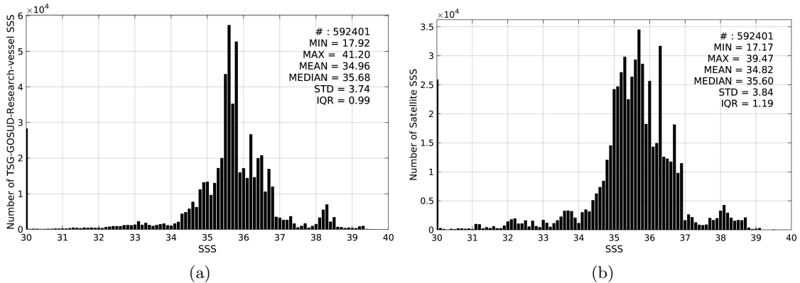
Figure 2: Histograms of SSS from TSG-GOSUD-Research-vessel (a) and SMAP-L3-RSS-V2-MONTHLY-70KM (b) considering all match-up pairs per bins of 0.1 over the SMOS coastal zone ( \approx 800 km) 60N-60S Pi-MEP region and for the full satellite product period.
