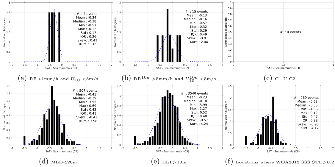
Figure 13: Normalized histogram of \Delta SSS (SMAP-L3-RSS-V2-MONTHLY-70KM - Sea mammals) for 6 different subdatasets corresponding to: RR > 1\text{mm/h} and U_{10} < 5\text{m/s} (a), RR^{10d} > 5\text{mm/h} and U_{10}^{10d} < 5\text{m/s} (b), C1 U C2 (c), MLD < 20\text{m} (d), BLT > 10\text{m} (e), Locations where WOA2013 SSS STD > 0.2 (f).
