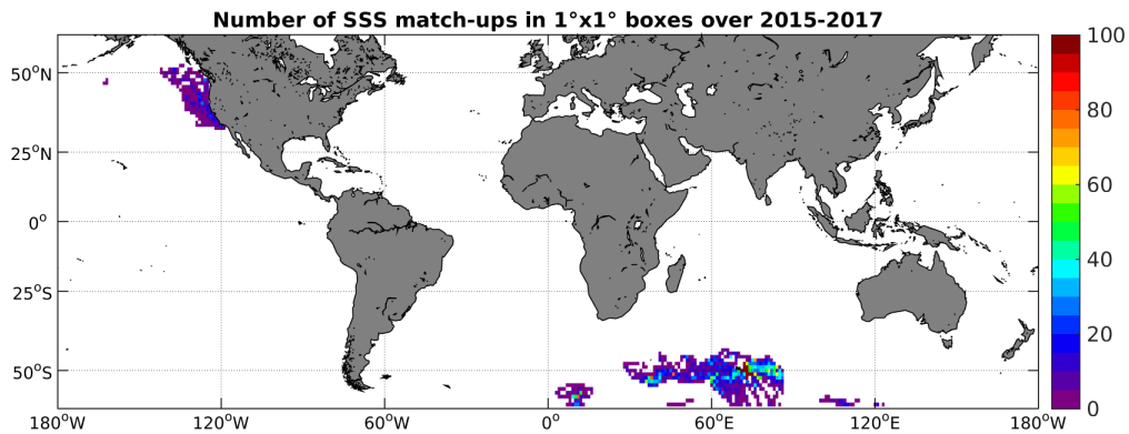
Figure 4: Number of SSS match-ups between Sea mammals SSS and the SMAP-L3-RSS-V2-MONTHLY-70KM SSS product for the SMOS coastal zone ( \approx 800\text{km} ) 60N-60S Pi-MEP region over 1^\circ \times 1^\circ boxes and for the full satellite product period.
