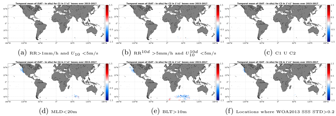
Figure 12: Temporal mean gridded over spatial boxes of size 1^\circ \times 1^\circ of \Delta SSS (SMAP-L3-RSS-V2-MONTHLY-70KM - Sea mammals) for 6 different subdatasets corresponding to:RR>1mm/h and U_{10} < 5 m/s (a), RR^{10d} > 5 mm/h and U_{10}^{10d} < 5 m/s (b), C1 U C2 (c),MLD<20m (d),BLT>10m (e),Locations where WOA2013 SSS STD>0.2 (f).
