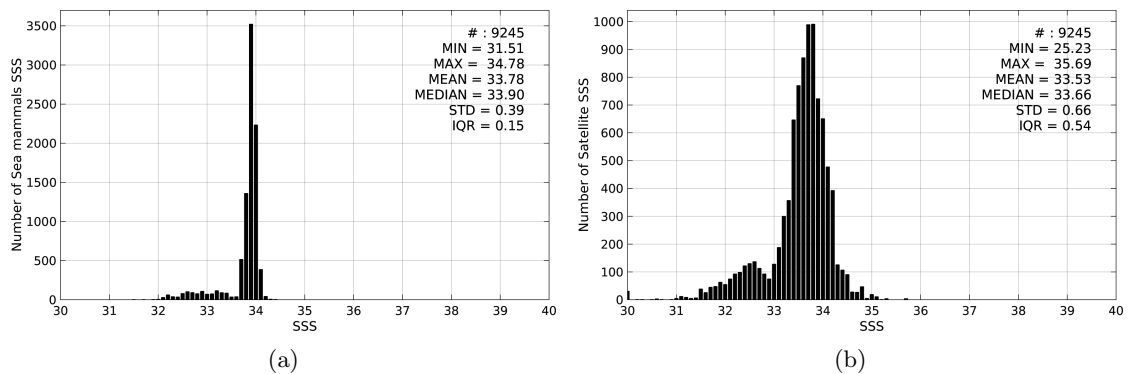
Figure 2: Histograms of SSS from Sea mammals (a) and SMAP-L3-RSS-V2-MONTHLY-70KM (b) considering all match-up pairs per bins of 0.1 over the SMOS coastal zone ( \geq 800\text{km} ) 60N-60S Pi-MEP region and for the full satellite product period.
