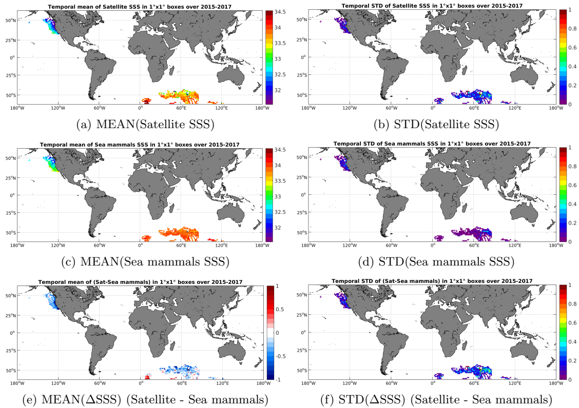
Figure 6: Temporal mean (left) and STD (right) of SSS from SMAP-L3-RSS-V2-MONTHLY-70KM (top), Sea mammals (middle), and of \Delta SSS (Satellite - Sea mammals). Only match-up pairs are used to generate these maps.
