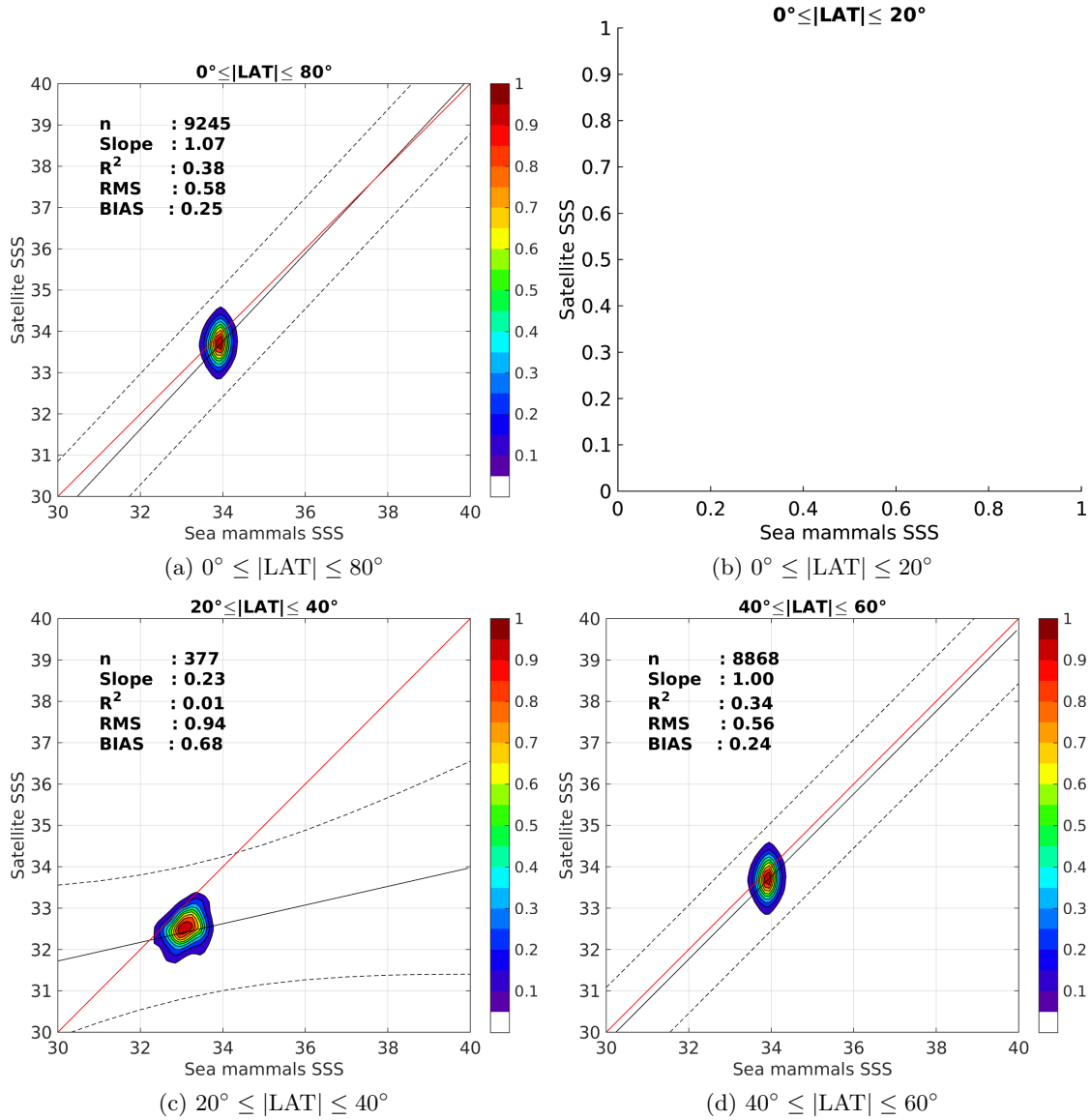
Figure 9: Contour maps of the concentration of SMAP-L3-RSS-V2-MONTHLY-70KM SSS (y-axis) versus Sea mammals SSS (x-axis) at match-up pairs for different latitude bands. For each plot, the red line shows x=y . The black thin and dashed lines indicate a linear fit through the data cloud and the \pm 95\% confidence levels, respectively. The number match-up pairs n , the slope and R^2 coefficient of the linear fit, the root mean square (RMS) and the mean bias between satellite and in situ data are indicated for each latitude band in each plots.
