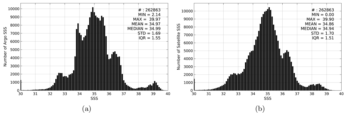
Figure 2: Histograms of SSS from Argo (a) and SMAP-L3-RSS-V2-MONTHLY-70KM (b) considering all match-up pairs per bins of 0.1 over the SMOS coastal zone ( \geq 800 km) 60N-60S Pi-MEP region and for the full satellite product period.
