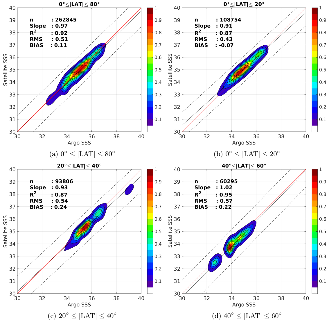
Figure 9: Contour maps of the concentration of SMAP-L3-RSS-V2-MONTHLY-70KM SSS (y-axis) versus Argo SSS (x-axis) at match-up pairs for different latitude bands. For each plot, the red line shows x=y . The black thin and dashed lines indicate a linear fit through the data cloud and the \pm 95\% confidence levels, respectively. The number match-up pairs n , the slope and R^2 coefficient of the linear fit, the root mean square (RMS) and the mean bias between satellite and in situ data are indicated for each latitude band in each plots.
