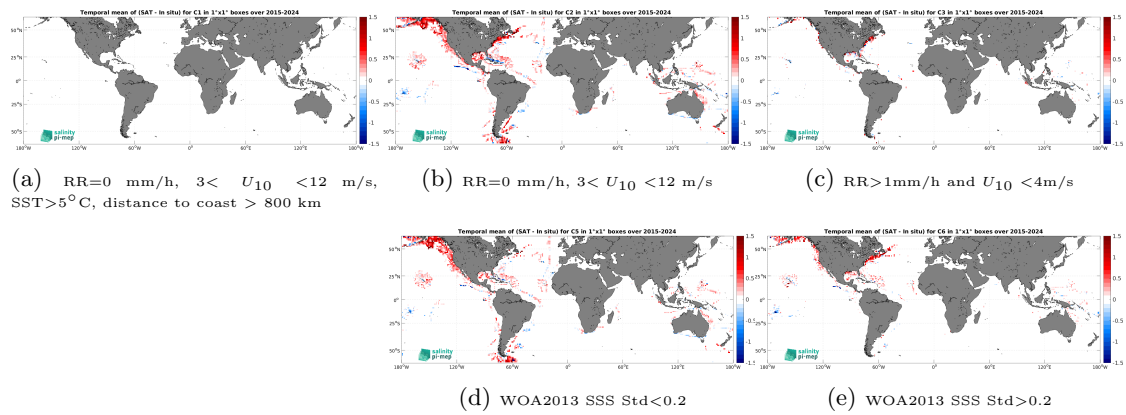
Figure 14: Temporal mean gridded over spatial boxes of size 1^\circ \times 1^\circ of \Delta SSS (SMAP SSS L3 v5.0 - 8-Day running (JPL) - TSG (SAMOS)) for 5 different subdatasets corresponding to:RR=0 mm/h, 3 < U_{10} < 12 m/s, SST>5°C, distance to coast > 800 km (a), RR=0 mm/h, 3 < U_{10} < 12 m/s (b), RR>1mm/h and U_{10} < 4 m/s (c), WOA2013 SSS Std<0.2 (d), WOA2013 SSS Std>0.2 (e).
