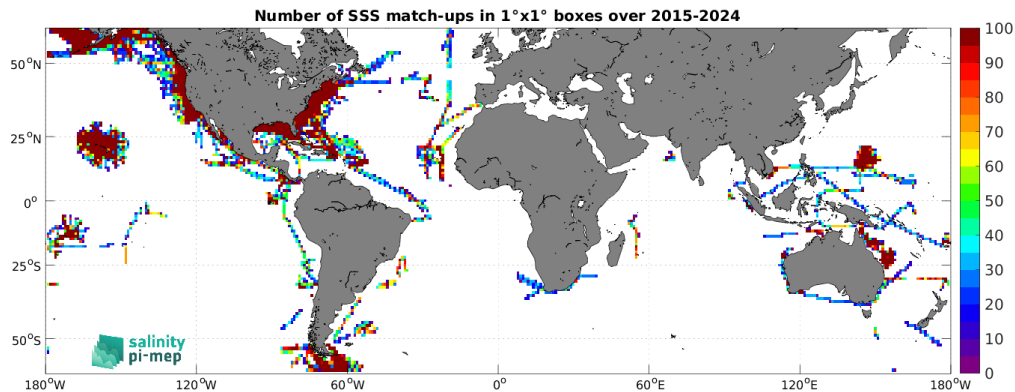
Figure 5: Number of SSS match-ups between TSG (SAMOS) SSS and the SMAP SSS L3 v5.0 - 8-Day running (JPL) SSS product for the SMOS coastal zone (<800km) 60N-60S Pi-MEP region over 1^\circ \times 1^\circ boxes and for the full satellite product period.
