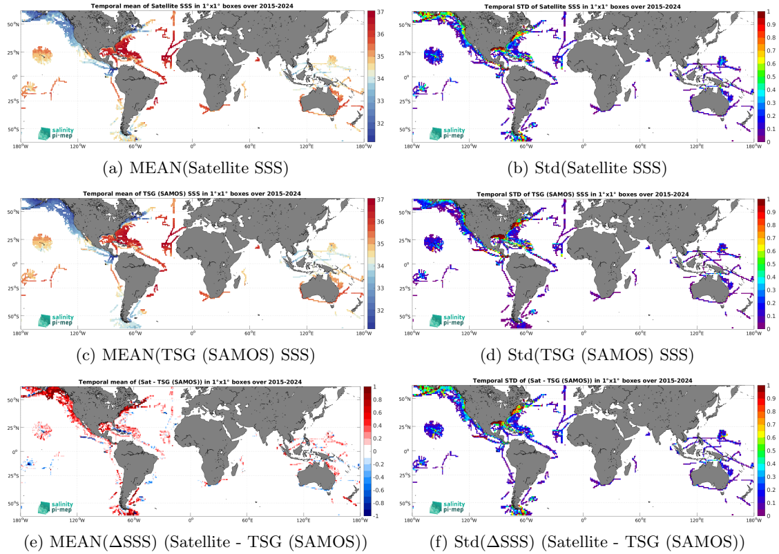
Figure 7: Temporal mean (left) and Std (right) of SSS from SMAP SSS L3 v5.0 - 8-Day running (JPL) (top), TSG (SAMOS) (middle), and of \Delta SSS (Satellite - TSG (SAMOS)). Only match-up pairs are used to generate these maps.
