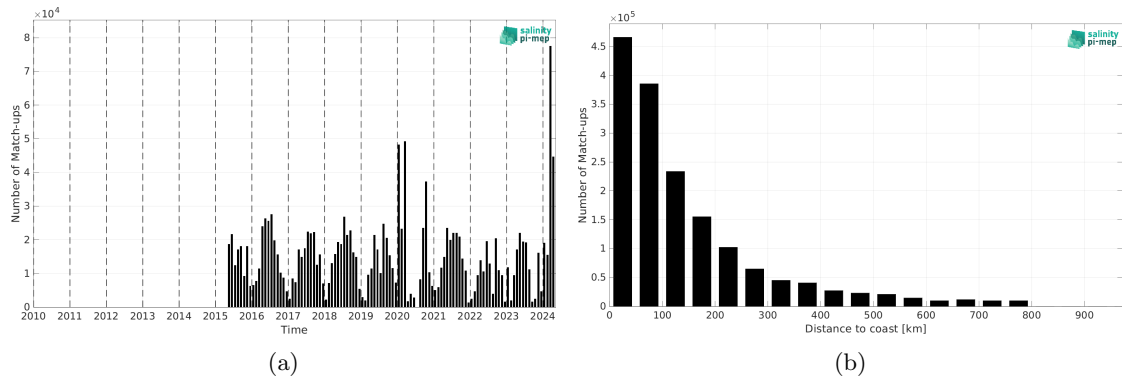
Figure 2: Number of match-ups between TSG (SAMOS) and SMAP SSS L3 v5.0 - 8-Day running (JPL) SSS as a function of time (a) and as function of the distance to coast (b) over the SMOS coastal zone (<800km) 60N-60S Pi-MEP region and for the full satellite product period.
