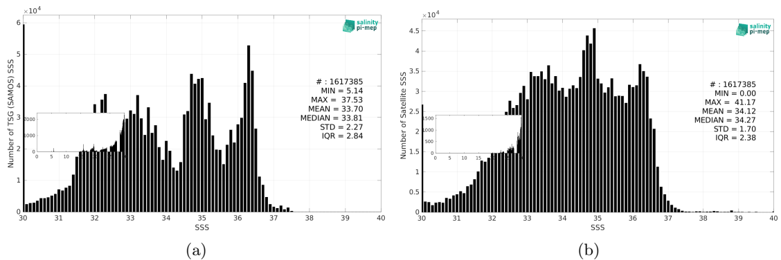
Figure 3: Histograms of SSS from TSG (SAMOS) (a) and SMAP SSS L3 v5.0 - 8-Day running (JPL) (b) considering all match-up pairs per bins of 0.1 over the SMOS coastal zone (<800km) 60N-60S Pi-MEP region and for the full satellite product period.
