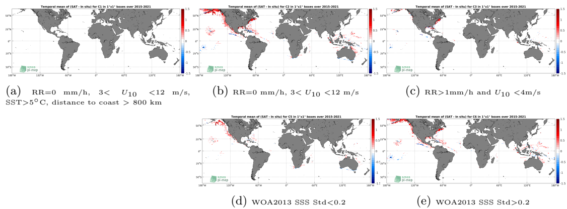
Figure 12: Temporal mean gridded over spatial boxes of size 1^\circ \times 1^\circ of \Delta\text{SSS} (SMAP SSS L3 v5.0 - 8-Day running (JPL) - TSG (SAMOS)) for 5 different subdatasets corresponding to:RR=0 mm/h, 3 < U_{10} < 12 m/s, SST >5^\circ\text{C} , distance to coast > 800 km (a), RR=0 mm/h, 3 < U_{10} < 12 m/s (b), RR >1 mm/h and U_{10} < 4 m/s (c), WOA2013 SSS Std <0.2 (d), WOA2013 SSS Std >0.2 (e).
