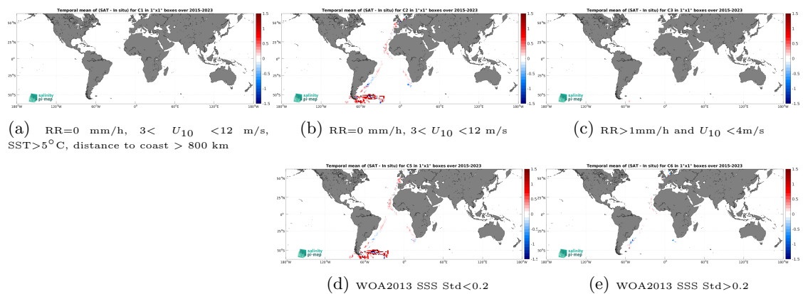
Figure 14: Temporal mean gridded over spatial boxes of size 1^\circ \times 1^\circ of \Delta SSS (SMAP SSS L3 v5.0 - 8-Day running (JPL) - TSG (Polarstern)) for 5 different subdatasets corresponding to:RR=0 mm/h, 3 < U_{10} < 12 m/s, SST >5^\circ\text{C} , distance to coast > 800 km (a), RR=0 mm/h, 3 < U_{10} < 12 m/s (b), RR >1 mm/h and U_{10} < 4 m/s (c), WOA2013 SSS Std <0.2 (d), WOA2013 SSS Std >0.2 (e).
