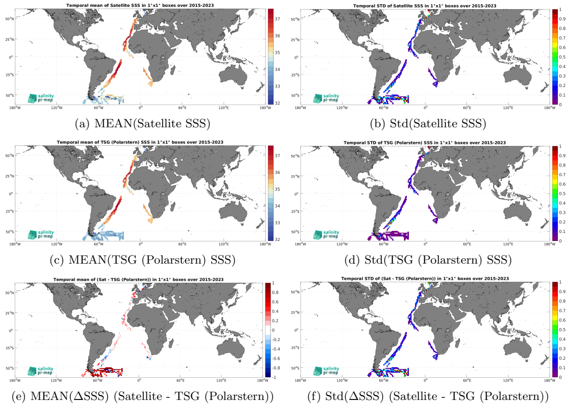
Figure 7: Temporal mean (left) and Std (right) of SSS from SMAP SSS L3 v5.0 - 8-Day running (JPL) (top), TSG (Polarstern) (middle), and of \Delta SSS (Satellite - TSG (Polarstern)). Only match-up pairs are used to generate these maps.
