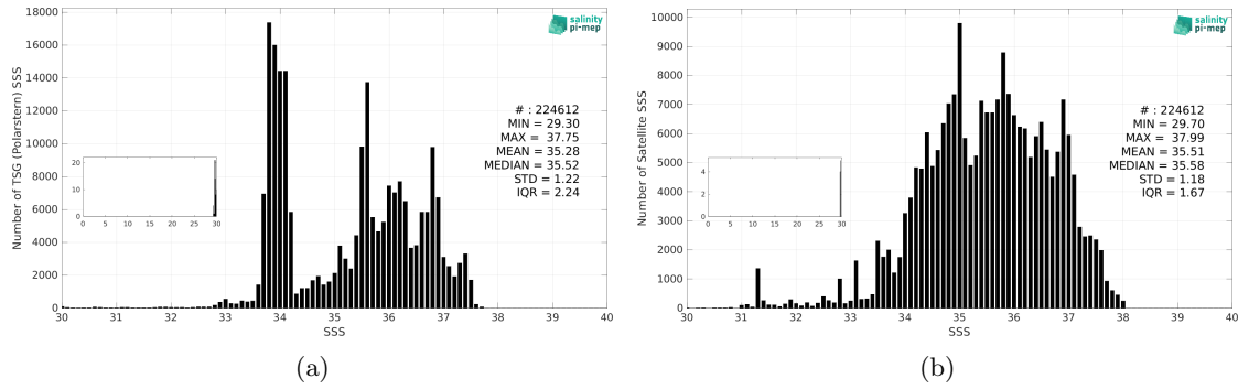
Figure 3: Histograms of SSS from TSG (Polarstern) (a) and SMAP SSS L3 v5.0 - 8-Day running (JPL) (b) considering all match-up pairs per bins of 0.1 over the SMOS coastal zone (<800km) 60N-60S Pi-MEP region and for the full satellite product period.
