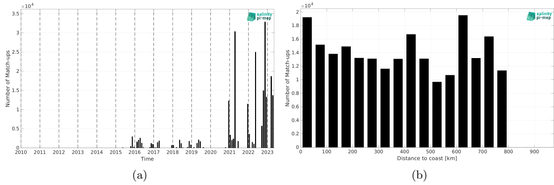
Figure 2: Number of match-ups between TSG (Polarstern) and SMAP SSS L3 v5.0 - 8-Day running (JPL) SSS as a function of time (a) and as function of the distance to coast (b) over the SMOS coastal zone (<800km) 60N-60S Pi-MEP region and for the full satellite product period.
