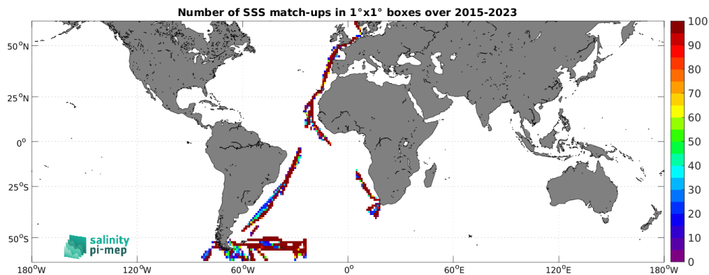
Figure 5: Number of SSS match-ups between TSG (Polarstern) SSS and the SMAP SSS L3 v5.0 - 8-Day running (JPL) SSS product for the SMOS coastal zone (<800km) 60N-60S Pi-MEP region over 1^\circ \times 1^\circ boxes and for the full satellite product period.
