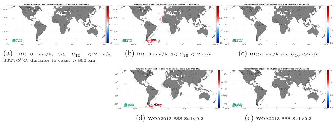
Figure 14: Temporal mean gridded over spatial boxes of size 1^\circ \times 1^\circ of \Delta\text{SSS} (SMAP SSS L3 v5.0 - 8-Day running (JPL) - TSG (Polarstern)) for 5 different subdatasets corresponding to: RR=0 mm/h, 3 < U_{10} < 12 m/s, SST > 5°C, distance to coast > 800 km (a), RR=0 mm/h, 3 < U_{10} < 12 m/s (b), RR > 1mm/h and U_{10} < 4 m/s (c), WOA2013 SSS Std < 0.2 (d), WOA2013 SSS Std > 0.2 (e).
