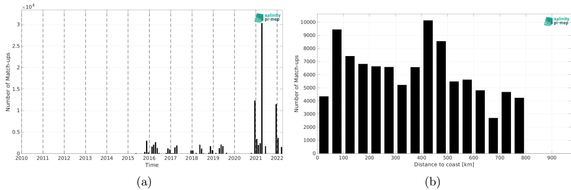
Figure 1: Number of match-ups between TSG (Polarstern) and SMAP SSS L3 v5.0 - 8-Day running (JPL) SSS as a function of time (a) and as function of the distance to coast (b) over the SMOS coastal zone (<800km) 60N-60S Pi-MEP region and for the full satellite product period.
