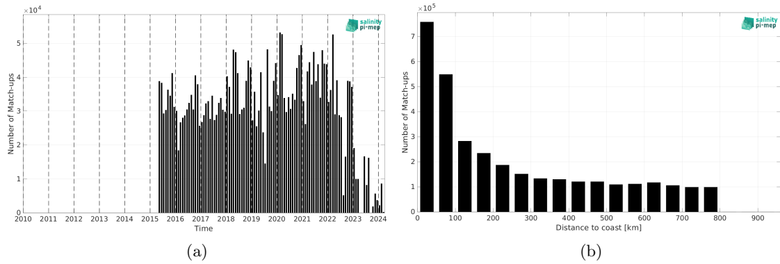
Figure 2: Number of match-ups between TSG (LEGOS-DM) and SMAP SSS L3 v5.0 - 8-Day running (JPL) SSS as a function of time (a) and as function of the distance to coast (b) over the SMOS coastal zone (<800km) 60N-60S Pi-MEP region and for the full satellite product period.
