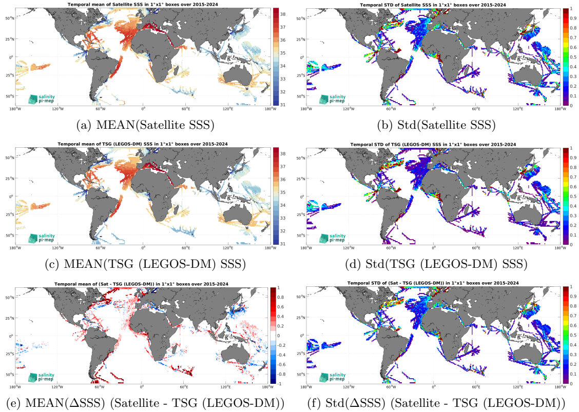
Figure 7: Temporal mean (left) and Std (right) of SSS from SMAP SSS L3 v5.0 - 8-Day running (JPL) (top), TSG (LEGOS-DM) (middle), and of \Delta SSS (Satellite - TSG (LEGOS-DM)). Only match-up pairs are used to generate these maps.
