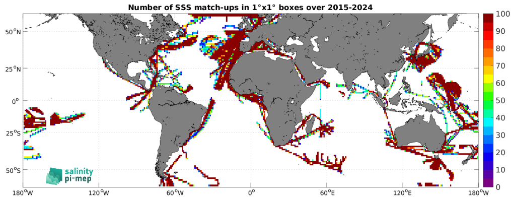
Figure 5: Number of SSS match-ups between TSG (LEGOS-DM) SSS and the SMAP SSS L3 v5.0 - 8-Day running (JPL) SSS product for the SMOS coastal zone (<800km) 60N-60S Pi-MEP region over 1°x1° boxes and for the full satellite product period.
