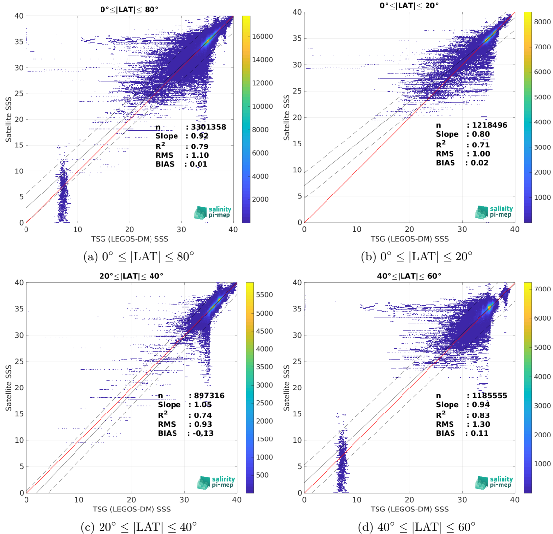
Figure 10: Contour maps of the concentration of SMAP SSS L3 v5.0 - 8-Day running (JPL) SSS (y-axis) versus TSG (LEGOS-DM) SSS (x-axis) at match-up pairs for different latitude bands. For each plot, the red line shows x=y . The black thin and dashed lines indicate a linear fit through the data cloud and the \pm 95\% confidence levels, respectively. The number match-up pairs n , the slope and R^2 coefficient of the linear fit, the root mean square (RMS) and the mean bias between satellite and in situ data are indicated for each latitude band in each plot.
