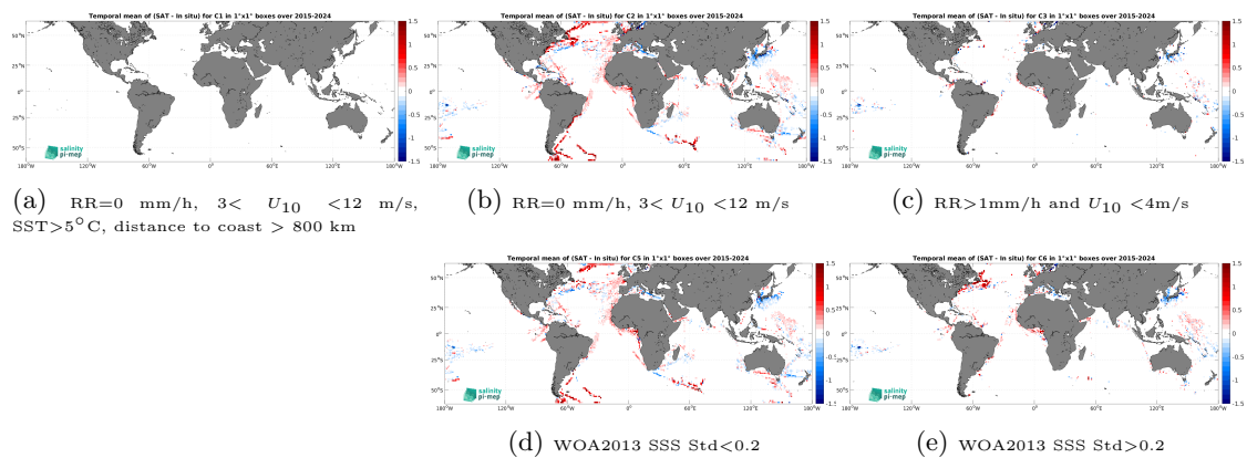
Figure 14: Temporal mean gridded over spatial boxes of size 1^\circ \times 1^\circ of \Delta\text{SSS} (SMAP SSS L3 v5.0 - 8-Day running (JPL) - TSG (LEGOS-DM)) for 5 different subdatasets corresponding to:RR=0 mm/h, 3 < U_{10} < 12 m/s, SST > 5^\circ\text{C} , distance to coast > 800 km (a), RR=0 mm/h, 3 < U_{10} < 12 m/s (b), RR > 1 mm/h and U_{10} < 4 m/s (c), WOA2013 SSS Std < 0.2 (d), WOA2013 SSS Std > 0.2 (e).
