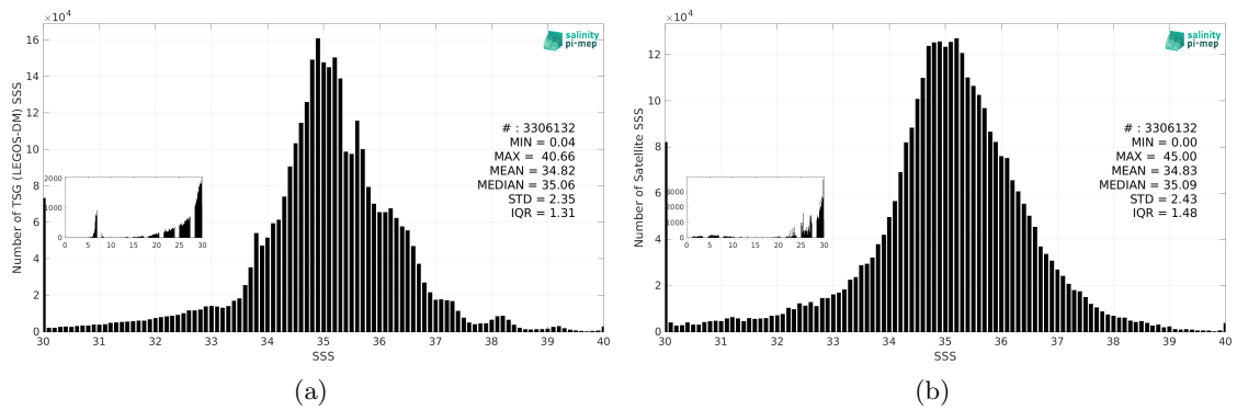
Figure 3: Histograms of SSS from TSG (LEGOS-DM) (a) and SMAP SSS L3 v5.0 - 8-Day running (JPL) (b) considering all match-up pairs per bins of 0.1 over the SMOS coastal zone (<800km) 60N-60S Pi-MEP region and for the full satellite product period.
