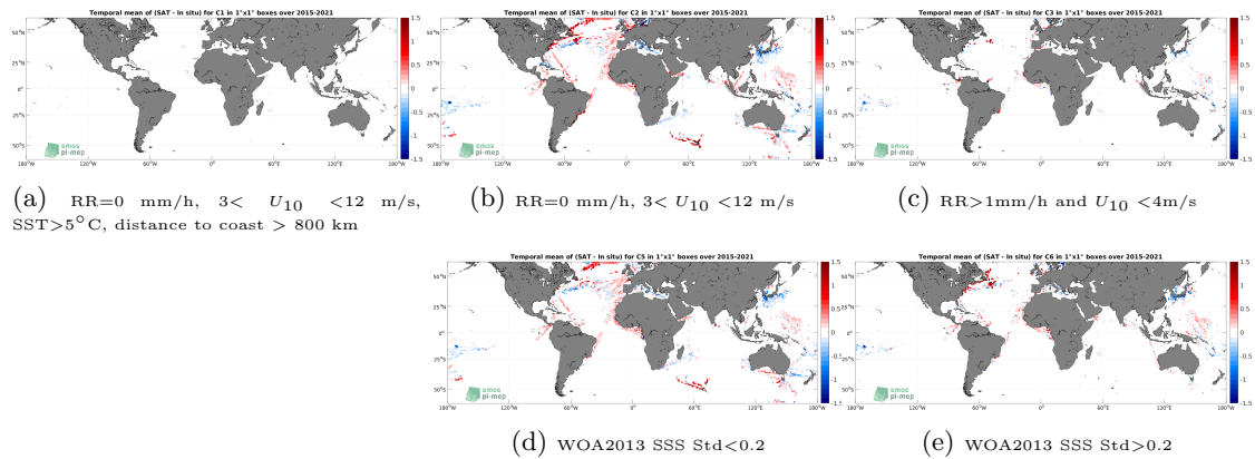
Figure 12: Temporal mean gridded over spatial boxes of size 1^\circ \times 1^\circ of \Delta SSS (SMAP SSS L3 v5.0 - 8-Day running (JPL) - TSG (LEGOS-DM)) for 5 different subdatasets corresponding to:RR=0 mm/h, 3 < U_{10} < 12 m/s, SST >5^\circ\text{C} , distance to coast > 800 km (a), RR=0 mm/h, 3 < U_{10} < 12 m/s (b), RR >1 mm/h and U_{10} < 4 m/s (c), WOA2013 SSS Std <0.2 (d), WOA2013 SSS Std >0.2 (e).
