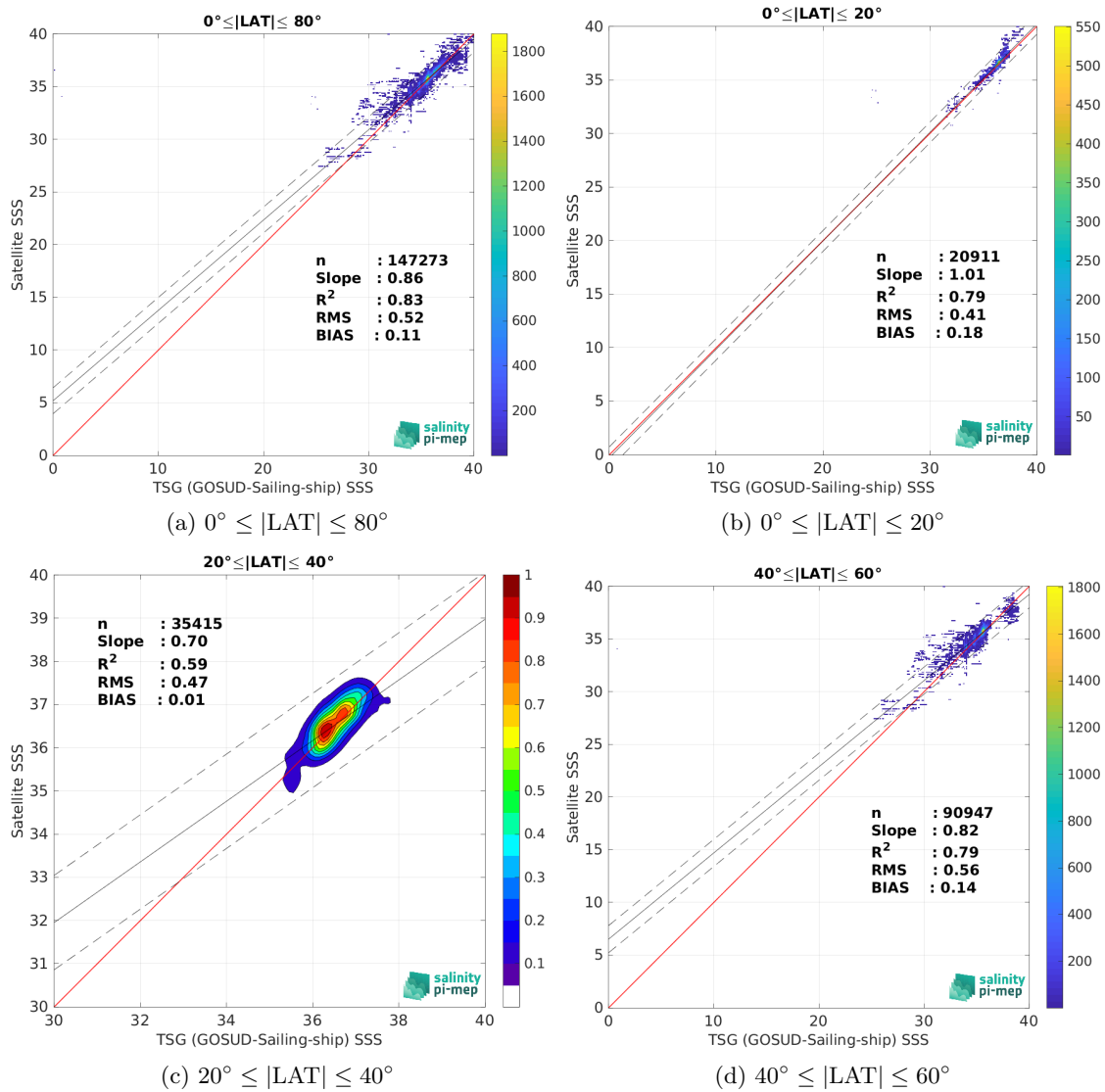
Figure 10: Contour maps of the concentration of SMAP SSS L3 v5.0 - 8-Day running (JPL) SSS (y-axis) versus TSG (GOSUD-Sailing-ship) SSS (x-axis) at match-up pairs for different latitude bands. For each plot, the red line shows x=y . The black thin and dashed lines indicate a linear fit through the data cloud and the \pm 95\% confidence levels, respectively. The number match-up pairs n , the slope and R^2 coefficient of the linear fit, the root mean square (RMS) and the mean bias between satellite and in situ data are indicated for each latitude band in each plots.
