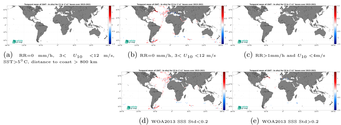
Figure 14: Temporal mean gridded over spatial boxes of size 1^\circ \times 1^\circ of \Delta\text{SSS} (SMAP SSS L3 v5.0 - 8-Day running (JPL) - TSG (GOSUD-Sailing-ship)) for 5 different subdatasets corresponding to:RR=0 mm/h, 3 < U_{10} < 12 m/s, SST > 5^\circ\text{C} , distance to coast > 800 km (a), RR=0 mm/h, 3 < U_{10} < 12 m/s (b), RR > 1 mm/h and U_{10} < 4 m/s (c), WOA2013 SSS Std < 0.2 (d), WOA2013 SSS Std > 0.2 (e).
