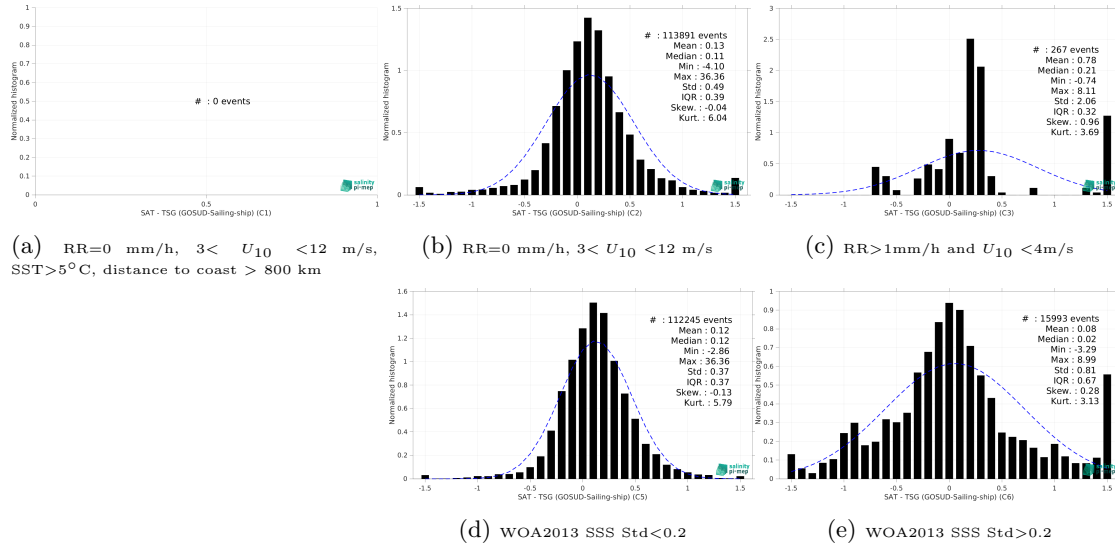
Figure 15: Normalized histogram of \Delta SSS (SMAP SSS L3 v5.0 - 8-Day running (JPL) - TSG (GOSUD-Sailing-ship)) for 5 different subdatasets corresponding to: RR=0 mm/h, 3 < U_{10} < 12 m/s, SST>5°C, distance to coast > 800 km (a), RR=0 mm/h, 3 < U_{10} < 12 m/s (b), RR>1mm/h and U_{10} < 4 m/s (c), WOA2013 SSS Std<0.2 (d), WOA2013 SSS Std>0.2 (e).
