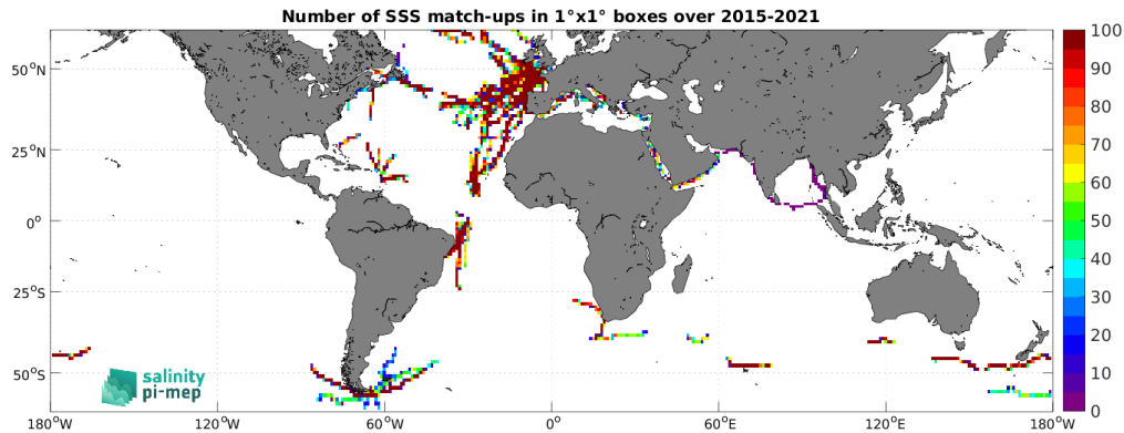
Figure 5: Number of SSS match-ups between TSG (GOSUD-Sailing-ship) SSS and the SMAP SSS L3 v5.0 - 8-Day running (JPL) SSS product for the SMOS coastal zone (<800km) 60N-60S Pi-MEP region over 1^\circ \times 1^\circ boxes and for the full satellite product period.
