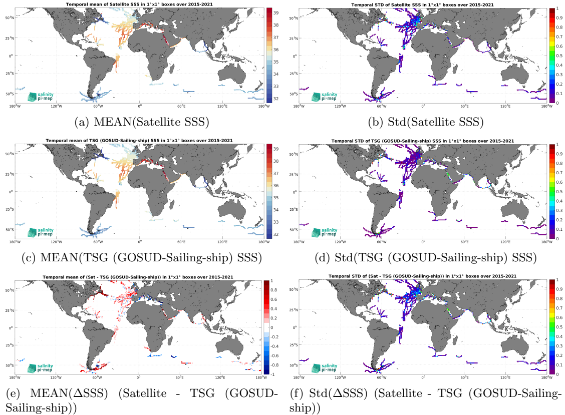
Figure 7: Temporal mean (left) and Std (right) of SSS from SMAP SSS L3 v5.0 - 8-Day running (JPL) (top), TSG (GOSUD-Sailing-ship) (middle), and of \Delta SSS (Satellite - TSG (GOSUD-Sailing-ship)). Only match-up pairs are used to generate these maps.
