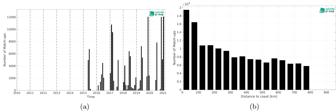
Figure 2: Number of match-ups between TSG (GOSUD-Sailing-ship) and SMAP SSS L3 v5.0 - 8-Day running (JPL) SSS as a function of time (a) and as function of the distance to coast (b) over the SMOS coastal zone (<800km) 60N-60S Pi-MEP region and for the full satellite product period.
