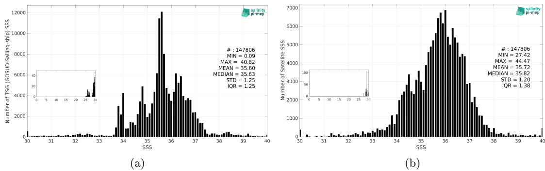
Figure 3: Histograms of SSS from TSG (GOSUD-Sailing-ship) (a) and SMAP SSS L3 v5.0 - 8-Day running (JPL) (b) considering all match-up pairs per bins of 0.1 over the SMOS coastal zone (<800km) 60N-60S Pi-MEP region and for the full satellite product period.
