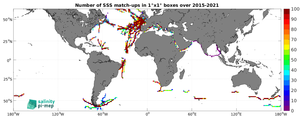
Figure 5: Number of SSS match-ups between TSG (GOSUD-Sailing-ship) SSS and the SMAP SSS L3 v5.0 - 8-Day running (JPL) SSS product for the SMOS coastal zone ( <800\text{km} ) 60N-60S Pi-MEP region over 1^\circ \times 1^\circ boxes and for the full satellite product period.
