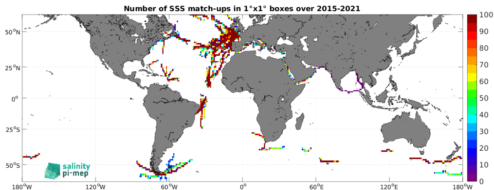
Figure 4: Number of SSS match-ups between TSG (GOSUD-Sailing-ship) SSS and the SMAP SSS L3 v5.0 - 8-Day running (JPL) SSS product for the SMOS coastal zone ( <800\text{km} ) 60N-60S Pi-MEP region over 1^\circ \times 1^\circ boxes and for the full satellite product period.
