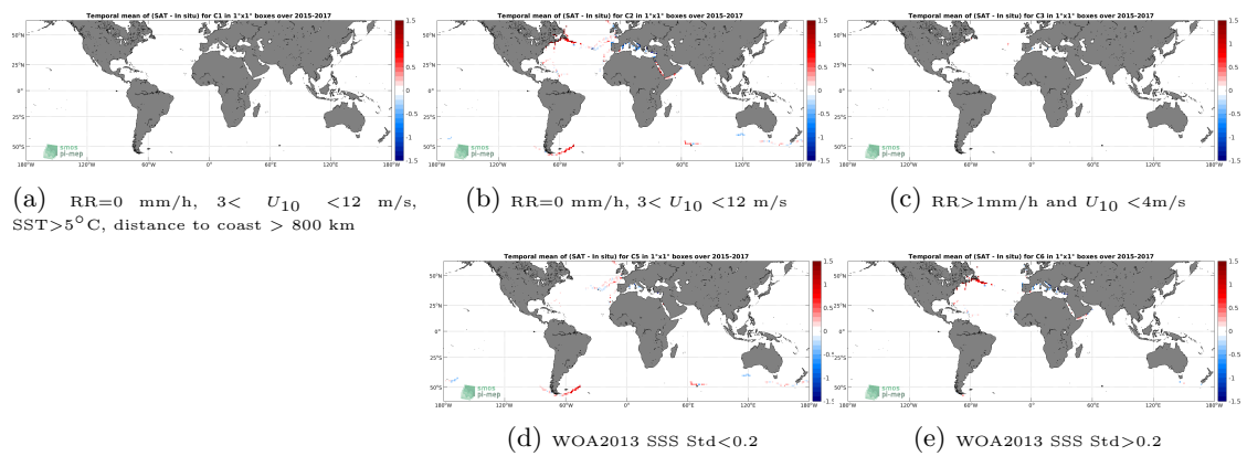
Figure 12: Temporal mean gridded over spatial boxes of size 1^\circ \times 1^\circ of \Delta\text{SSS} (SMAP SSS L3 v5.0 - 8-Day running (JPL) - TSG (GOSUD-Sailing-ship)) for 5 different subdatasets corresponding to:RR=0 mm/h, 3 < U_{10} < 12 m/s, SST>5°C, distance to coast > 800 km (a), RR=0 mm/h, 3 < U_{10} < 12 m/s (b), RR>1mm/h and U_{10} < 4 m/s (c), WOA2013 SSS Std<0.2 (d), WOA2013 SSS Std>0.2 (e).
