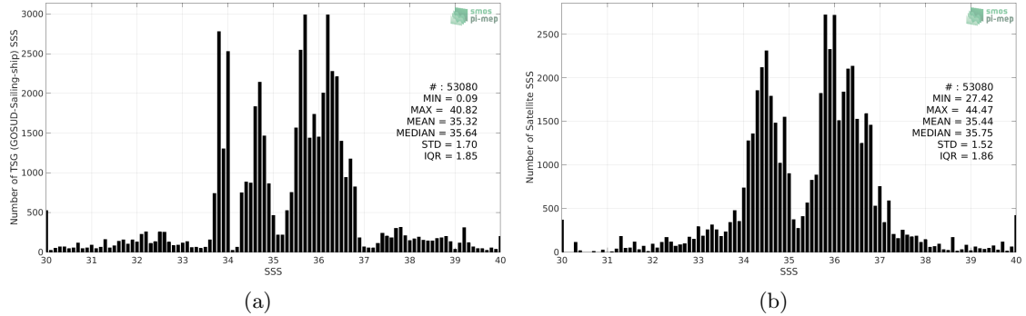
Figure 2: Histograms of SSS from TSG (GOSUD-Sailing-ship) (a) and SMAP SSS L3 v5.0 - 8-Day running (JPL) (b) considering all match-up pairs per bins of 0.1 over the SMOS coastal zone (<800km) 60N-60S Pi-MEP region and for the full satellite product period.
