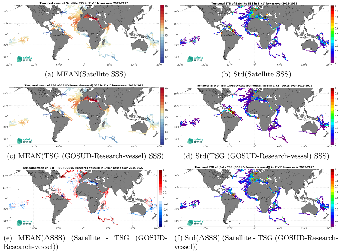
Figure 7: Temporal mean (left) and Std (right) of SSS from SMAP SSS L3 v5.0 - 8-Day running (JPL) (top), TSG (GOSUD-Research-vessel) (middle), and of \Delta SSS (Satellite - TSG (GOSUD-Research-vessel)). Only match-up pairs are used to generate these maps.
