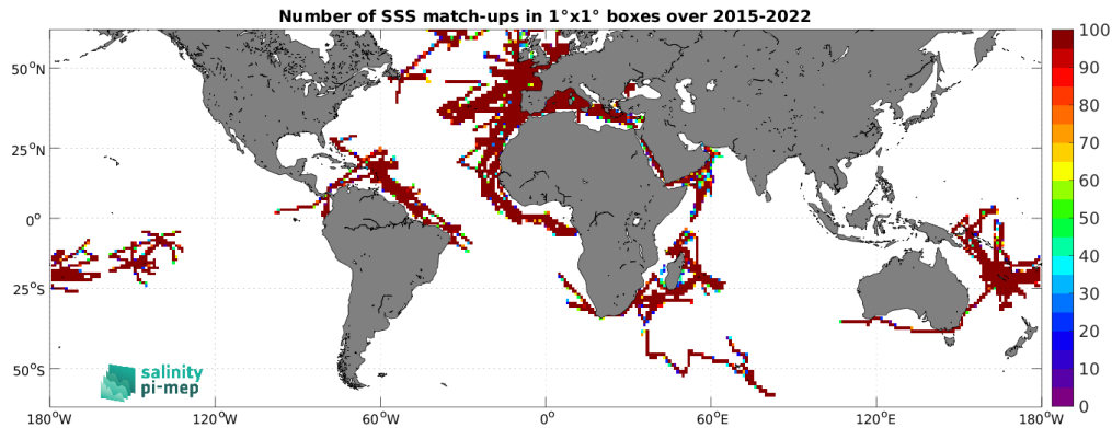
Figure 5: Number of SSS match-ups between TSG (GOSUD-Research-vessel) SSS and the SMAP SSS L3 v5.0 - 8-Day running (JPL) SSS product for the SMOS coastal zone ( <800\text{km} ) 60\text{N} - 60\text{S} Pi-MEP region over 1^\circ \times 1^\circ boxes and for the full satellite product period.
