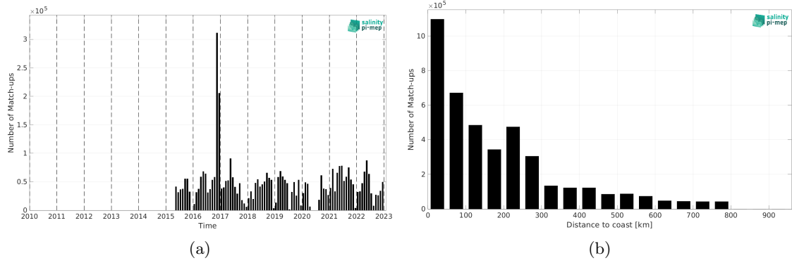
Figure 2: Number of match-ups between TSG (GOSUD-Research-vessel) and SMAP SSS L3 v5.0 - 8-Day running (JPL) SSS as a function of time (a) and as function of the distance to coast (b) over the SMOS coastal zone (<800km) 60N-60S Pi-MEP region and for the full satellite product period.
