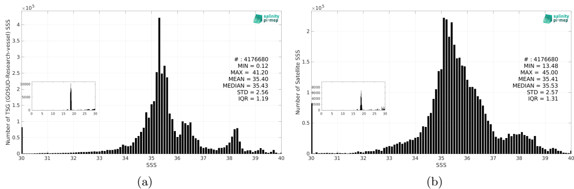
Figure 3: Histograms of SSS from TSG (GOSUD-Research-vessel) (a) and SMAP SSS L3 v5.0 - 8-Day running (JPL) (b) considering all match-up pairs per bins of 0.1 over the SMOS coastal zone (<800km) 60N-60S Pi-MEP region and for the full satellite product period.
