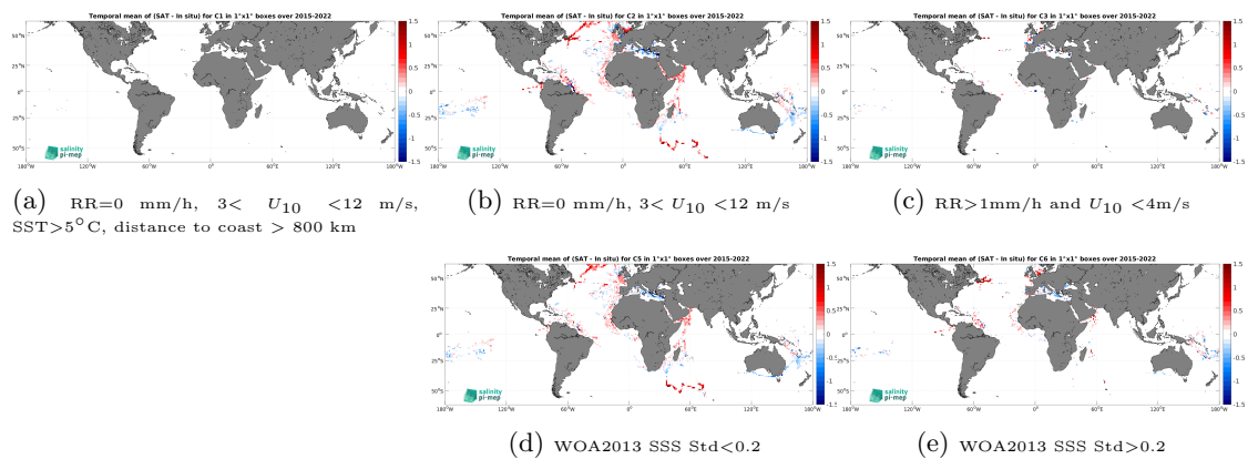
Figure 14: Temporal mean gridded over spatial boxes of size 1^\circ \times 1^\circ of \Delta\text{SSS} (SMAP SSS L3 v5.0 - 8-Day running (JPL) - TSG (GOSUD-Research-vessel)) for 5 different subdatasets corresponding to:RR=0 mm/h, 3 < U_{10} < 12 m/s, SST >5^\circ\text{C} , distance to coast > 800 km (a), RR=0 mm/h, 3 < U_{10} < 12 m/s (b), RR >1 mm/h and U_{10} < 4 m/s (c), WOA2013 SSS Std <0.2 (d), WOA2013 SSS Std >0.2 (e).
