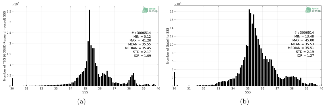
Figure 2: Histograms of SSS from TSG (GOSUD-Research-vessel) (a) and SMAP SSS L3 v5.0 - 8-Day running (JPL) (b) considering all match-up pairs per bins of 0.1 over the SMOS coastal zone (<800km) 60N-60S Pi-MEP region and for the full satellite product period.
