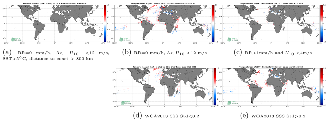
Figure 12: Temporal mean gridded over spatial boxes of size 1^\circ \times 1^\circ of \Delta SSS (SMAP SSS L3 v5.0 - 8-Day running (JPL) - TSG (GOSUD-Research-vessel)) for 5 different subdatasets corresponding to:RR=0 mm/h, 3 < U_{10} < 12 m/s, SST>5°C, distance to coast > 800 km (a), RR=0 mm/h, 3 < U_{10} < 12 m/s (b), RR>1mm/h and U_{10} < 4 m/s (c), WOA2013 SSS Std<0.2 (d), WOA2013 SSS Std>0.2 (e).
