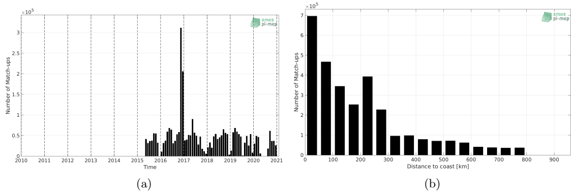
Figure 1: Number of match-ups between TSG (GOSUD-Research-vessel) and SMAP SSS L3 v5.0 - 8-Day running (JPL) SSS as a function of time (a) and as function of the distance to coast (b) over the SMOS coastal zone (<800km) 60N-60S Pi-MEP region and for the full satellite product period.
