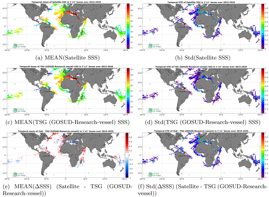
Figure 6: Temporal mean (left) and Std (right) of SSS from SMAP SSS L3 v5.0 - 8-Day running (JPL) (top), TSG (GOSUD-Research-vessel) (middle), and of \Delta SSS (Satellite - TSG (GOSUD-Research-vessel)). Only match-up pairs are used to generate these maps.
