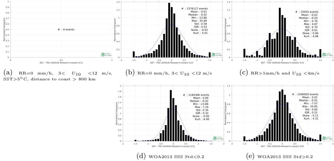
Figure 13: Normalized histogram of \Delta SSS (SMAP SSS L3 v5.0 - 8-Day running (JPL) - TSG (GOSUD-Research-vessel)) for 5 different subdatasets corresponding to: RR=0 mm/h, 3 < U_{10} < 12 m/s, SST>5°C, distance to coast > 800 km (a), RR=0 mm/h, 3 < U_{10} < 12 m/s (b), RR>1mm/h and U_{10} < 4 m/s (c), WOA2013 SSS Std<0.2 (d), WOA2013 SSS Std>0.2 (e).
