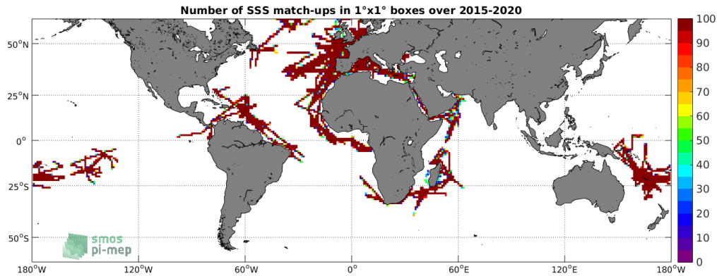
Figure 4: Number of SSS match-ups between TSG (GOSUD-Research-vessel) SSS and the SMAP SSS L3 v5.0 - 8-Day running (JPL) SSS product for the SMOS coastal zone (<800km) 60N-60S Pi-MEP region over 1°×1° boxes and for the full satellite product period.
