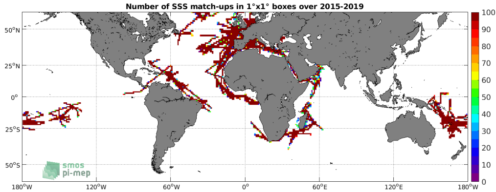
Figure 4: Number of SSS match-ups between TSG (GOSUD-Research-vessel) SSS and the SMAP SSS L3 v5.0 - 8-Day running (JPL) SSS product for the SMOS coastal zone (<800km) 60N-60S Pi-MEP region over 1^\circ \times 1^\circ boxes and for the full satellite product period.
