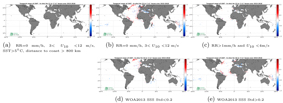
Figure 12: Temporal mean gridded over spatial boxes of size 1^\circ \times 1^\circ of \Delta\text{SSS} (SMAP SSS L3 v5.0 - 8-Day running (JPL) - TSG (GOSUD-Research-vessel)) for 5 different subdatasets corresponding to: RR=0 mm/h, 3 < U_{10} < 12 m/s, SST > 5°C, distance to coast > 800 km (a), RR=0 mm/h, 3 < U_{10} < 12 m/s (b), RR > 1mm/h and U_{10} < 4 m/s (c), WOA2013 SSS Std < 0.2 (d), WOA2013 SSS Std > 0.2 (e).
