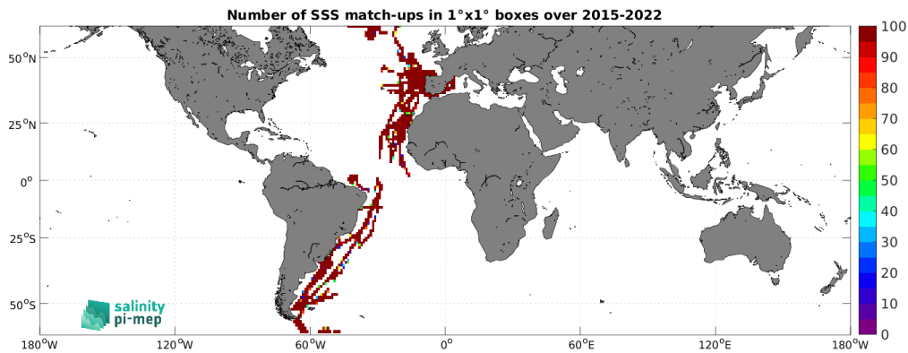
Figure 5: Number of SSS match-ups between TSG (CSIC-UTM) SSS and the SMAP SSS L3 v5.0 - 8-Day running (JPL) SSS product for the SMOS coastal zone (<800km) 60N-60S Pi-MEP region over 1^\circ \times 1^\circ boxes and for the full satellite product period.
