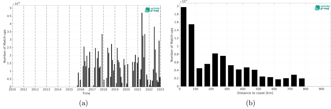
Figure 2: Number of match-ups between TSG (CSIC-UTM) and SMAP SSS L3 v5.0 - 8-Day running (JPL) SSS as a function of time (a) and as function of the distance to coast (b) over the SMOS coastal zone (<800km) 60N-60S Pi-MEP region and for the full satellite product period.
