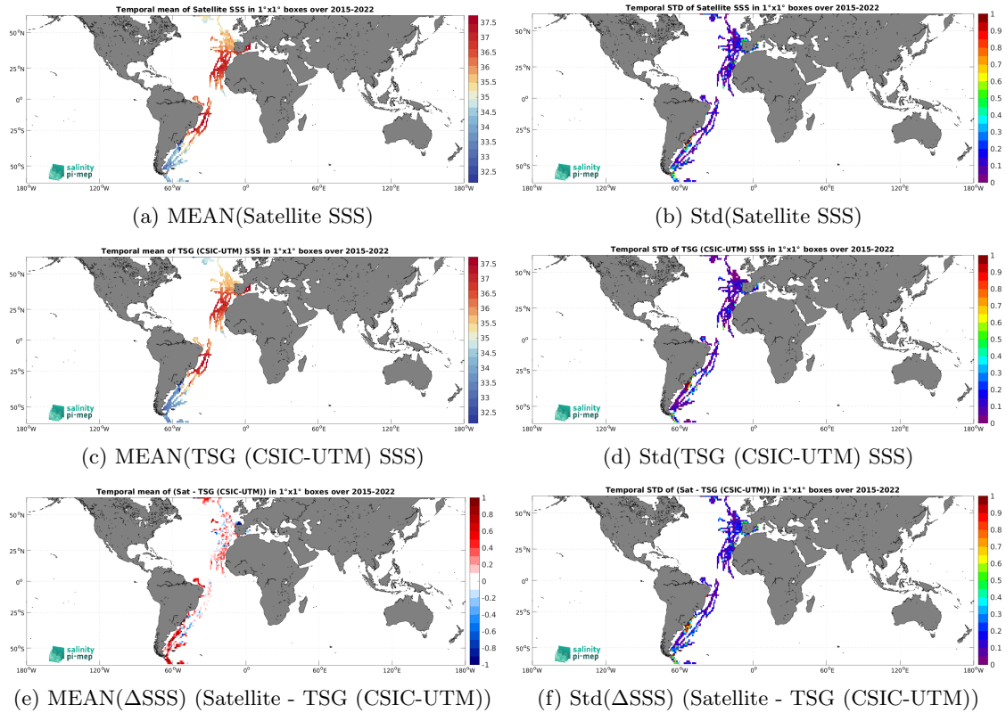
Figure 7: Temporal mean (left) and Std (right) of SSS from SMAP SSS L3 v5.0 - 8-Day running (JPL) (top), TSG (CSIC-UTM) (middle), and of \Delta SSS (Satellite - TSG (CSIC-UTM)). Only match-up pairs are used to generate these maps.
