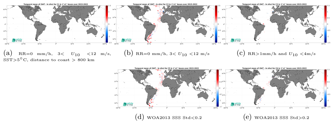
Figure 14: Temporal mean gridded over spatial boxes of size 1^\circ \times 1^\circ of \Delta SSS (SMAP SSS L3 v5.0 - 8-Day running (JPL) - TSG (CSIC-UTM)) for 5 different subdatasets corresponding to:RR=0 mm/h, 3 < U_{10} < 12 m/s, SST >5^\circ\text{C} , distance to coast > 800 km (a), RR=0 mm/h, 3 < U_{10} < 12 m/s (b), RR >1 mm/h and U_{10} < 4 m/s (c), WOA2013 SSS Std <0.2 (d), WOA2013 SSS Std >0.2 (e).
