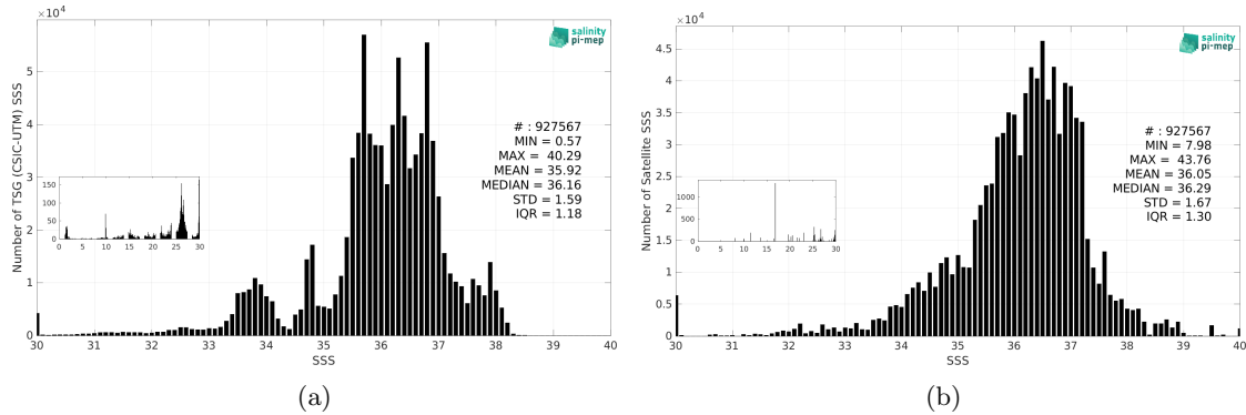
Figure 3: Histograms of SSS from TSG (CSIC-UTM) (a) and SMAP SSS L3 v5.0 - 8-Day running (JPL) (b) considering all match-up pairs per bins of 0.1 over the SMOS coastal zone (<800km) 60N-60S Pi-MEP region and for the full satellite product period.
