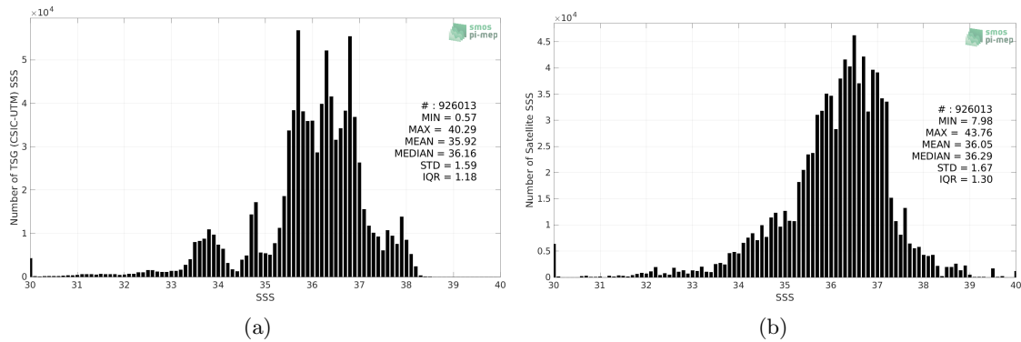
Figure 2: Histograms of SSS from TSG (CSIC-UTM) (a) and SMAP SSS L3 v5.0 - 8-Day running (JPL) (b) considering all match-up pairs per bins of 0.1 over the SMOS coastal zone (<800km) 60N-60S Pi-MEP region and for the full satellite product period.
