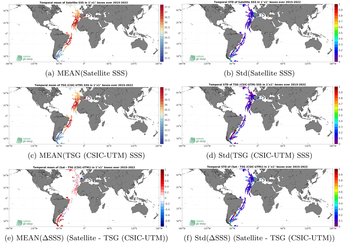
Figure 6: Temporal mean (left) and Std (right) of SSS from SMAP SSS L3 v5.0 - 8-Day running (JPL) (top), TSG (CSIC-UTM) (middle), and of \Delta SSS (Satellite - TSG (CSIC-UTM)). Only match-up pairs are used to generate these maps.
