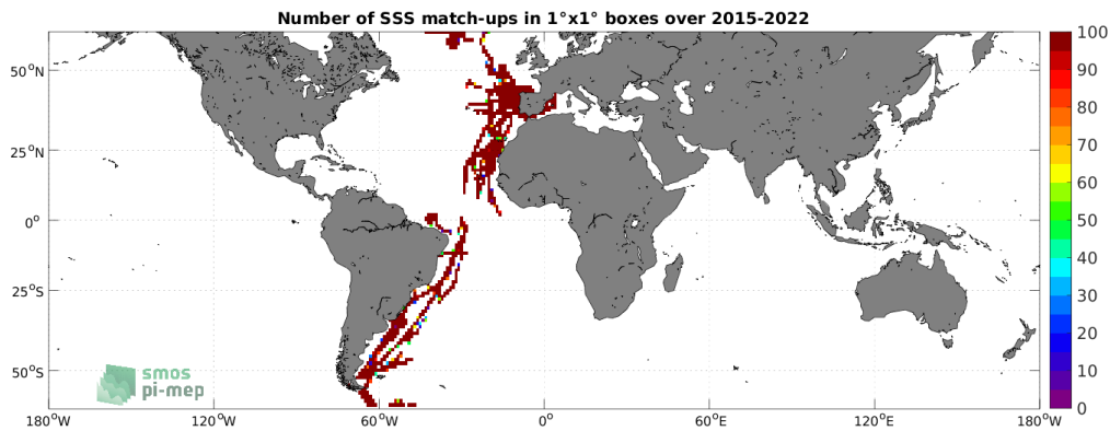
Figure 4: Number of SSS match-ups between TSG (CSIC-UTM) SSS and the SMAP SSS L3 v5.0 - 8-Day running (JPL) SSS product for the SMOS coastal zone (<800km) 60N-60S Pi-MEP region over 1^\circ \times 1^\circ boxes and for the full satellite product period.
