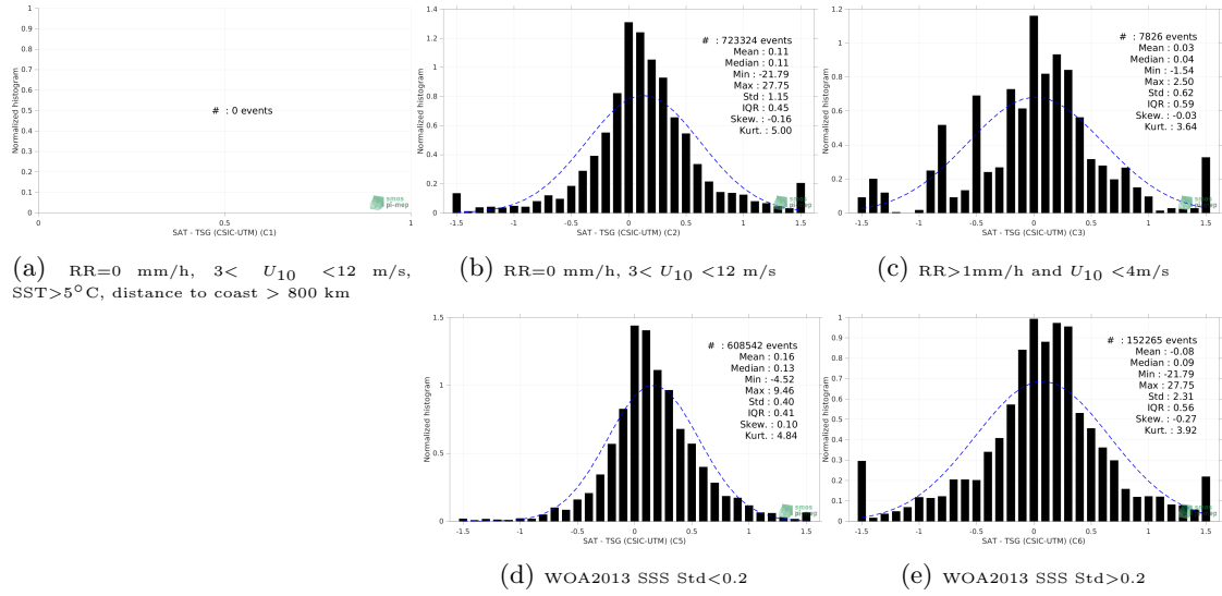
Figure 13: Normalized histogram of \Delta SSS (SMAP SSS L3 v5.0 - 8-Day running (JPL) - TSG (CSIC-UTM)) for 5 different subdatasets corresponding to: RR=0 mm/h, 3 < U_{10} < 12 m/s, SST > 5°C, distance to coast > 800 km (a), RR=0 mm/h, 3 < U_{10} < 12 m/s (b), RR > 1mm/h and U_{10} < 4 m/s (c), WOA2013 SSS Std < 0.2 (d), WOA2013 SSS Std > 0.2 (e).
