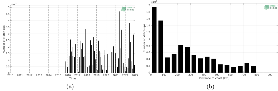
Figure 1: Number of match-ups between TSG (CSIC-UTM) and SMAP SSS L3 v5.0 - 8-Day running (JPL) SSS as a function of time (a) and as function of the distance to coast (b) over the SMOS coastal zone (<800km) 60N-60S Pi-MEP region and for the full satellite product period.
