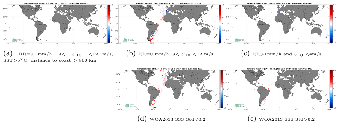
Figure 12: Temporal mean gridded over spatial boxes of size 1^\circ \times 1^\circ of \Delta SSS (SMAP SSS L3 v5.0 - 8-Day running (JPL) - TSG (CSIC-UTM)) for 5 different subdatasets corresponding to:RR=0 mm/h, 3 < U_{10} < 12 m/s, SST >5^\circ C, distance to coast > 800 km (a), RR=0 mm/h, 3 < U_{10} < 12 m/s (b), RR >1 mm/h and U_{10} < 4 m/s (c), WOA2013 SSS Std <0.2 (d), WOA2013 SSS Std >0.2 (e).
