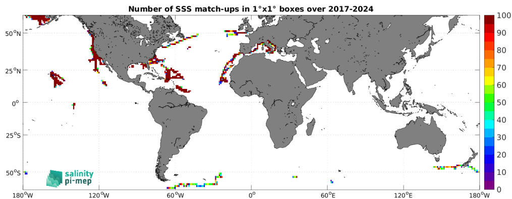
Figure 5: Number of SSS match-ups between Saildrone SSS and the SMAP SSS L3 v5.0 - 8-Day running (JPL) SSS product for the SMOS coastal zone (<800km) 60N-60S Pi-MEP region over 1^\circ \times 1^\circ boxes and for the full satellite product period.
