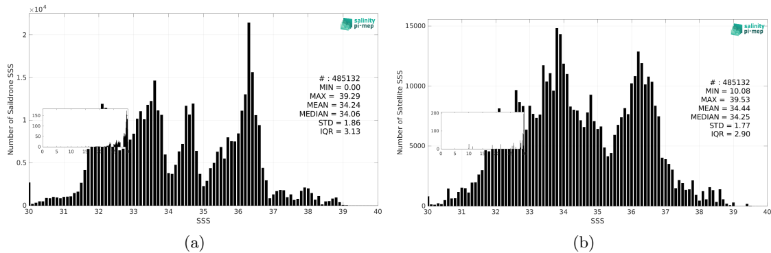
Figure 3: Histograms of SSS from Sairdrone (a) and SMAP SSS L3 v5.0 - 8-Day running (JPL) (b) considering all match-up pairs per bins of 0.1 over the SMOS coastal zone (<800km) 60N-60S Pi-MEP region and for the full satellite product period.
