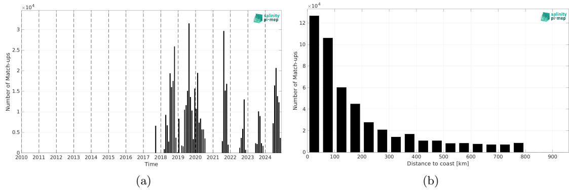
Figure 2: Number of match-ups between Sairdrone and SMAP SSS L3 v5.0 - 8-Day running (JPL) SSS as a function of time (a) and as function of the distance to coast (b) over the SMOS coastal zone (<800km) 60N-60S Pi-MEP region and for the full satellite product period.
