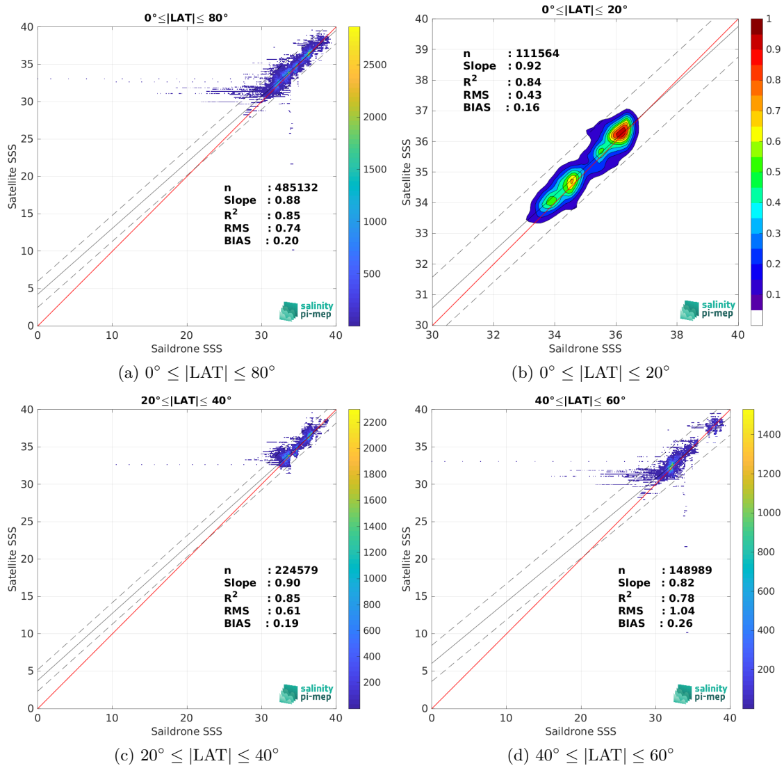
Figure 10: Contour maps of the concentration of SMAP SSS L3 v5.0 - 8-Day running (JPL) SSS (y-axis) versus Saildrone SSS (x-axis) at match-up pairs for different latitude bands. For each plot, the red line shows x=y . The black thin and dashed lines indicate a linear fit through the data cloud and the \pm 95\% confidence levels, respectively. The number match-up pairs n , the slope and R^2 coefficient of the linear fit, the root mean square (RMS) and the mean bias between satellite and in situ data are indicated for each latitude band in each plots.
