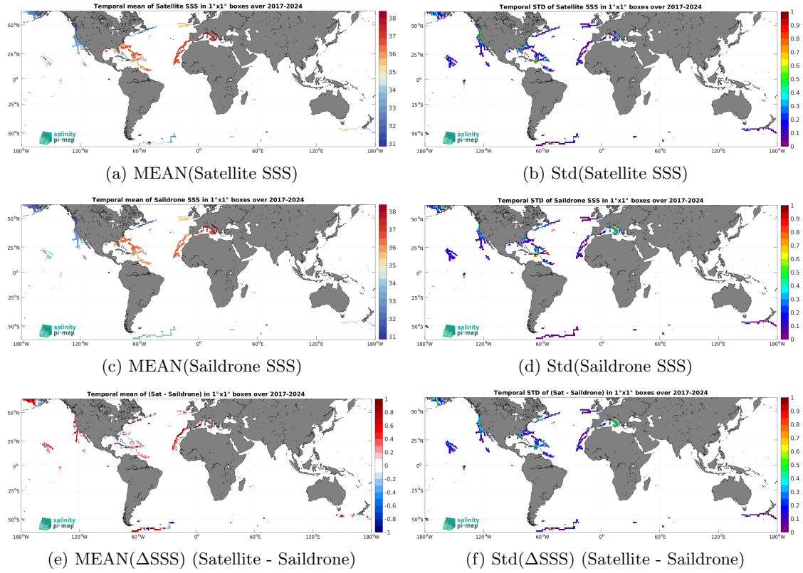
Figure 7: Temporal mean (left) and Std (right) of SSS from SMAP SSS L3 v5.0 - 8-Day running (JPL) (top), Saildrone (middle), and of \Delta SSS (Satellite - Saildrone). Only match-up pairs are used to generate these maps.
