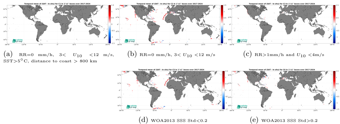
Figure 14: Temporal mean gridded over spatial boxes of size 1^\circ \times 1^\circ of \Delta\text{SSS} (SMAP SSS L3 v5.0 - 8-Day running (JPL) - Saildrone) for 5 different subdatasets corresponding to:RR=0 mm/h, 3 < U_{10} < 12 m/s, SST>5°C, distance to coast > 800 km (a), RR=0 mm/h, 3 < U_{10} < 12 m/s (b), RR>1mm/h and U_{10} < 4 m/s (c), WOA2013 SSS Std<0.2 (d), WOA2013 SSS Std>0.2 (e).
