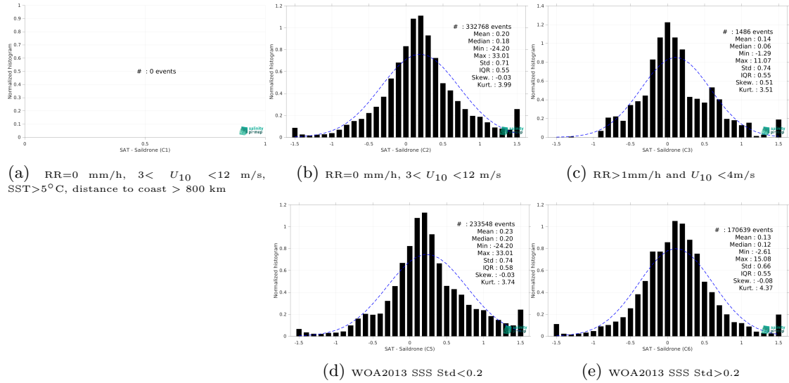
Figure 15: Normalized histogram of \Delta SSS (SMAP SSS L3 v5.0 - 8-Day running (JPL) - Saildrone) for 5 different subdatasets corresponding to: RR=0 mm/h, 3 < U_{10} < 12 m/s, SST > 5°C, distance to coast > 800 km (a), RR=0 mm/h, 3 < U_{10} < 12 m/s (b), RR > 1mm/h and U_{10} < 4 m/s (c), WOA2013 SSS Std < 0.2 (d), WOA2013 SSS Std > 0.2 (e).
