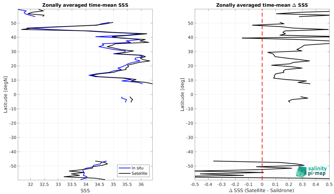
Figure 9: Left panel: Zonal mean SSS from SMAP SSS L3 v5.0 - 8-Day running (JPL) satellite product (black) and from Saildrone (blue). Right panel: Zonal mean of \Delta SSS (Satellite - Saildrone) for all the collected Pi-MEP match-up pairs estimated over the full satellite product period.
