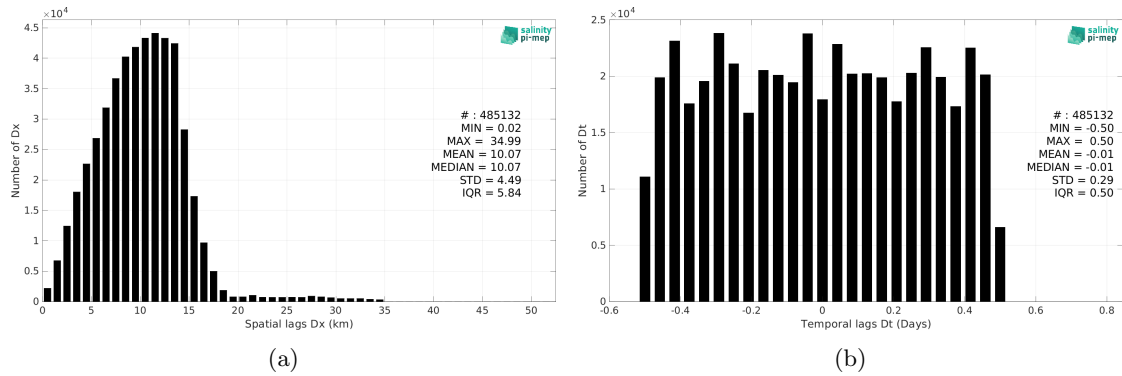
Figure 6: Histograms of the spatial (a) and temporal (b) lags between the location/time of the Saildrone measurement and the date of the corresponding SMAP SSS L3 v5.0 - 8-Day running (JPL) SSS pixel.
