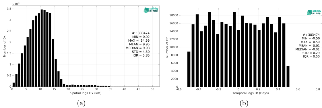
Figure 6: Histograms of the spatial (a) and temporal (b) lags between the location/time of the Sailability measurement and the date of the corresponding SMAP SSS L3 v5.0 - 8-Day running (JPL) SSS pixel.
