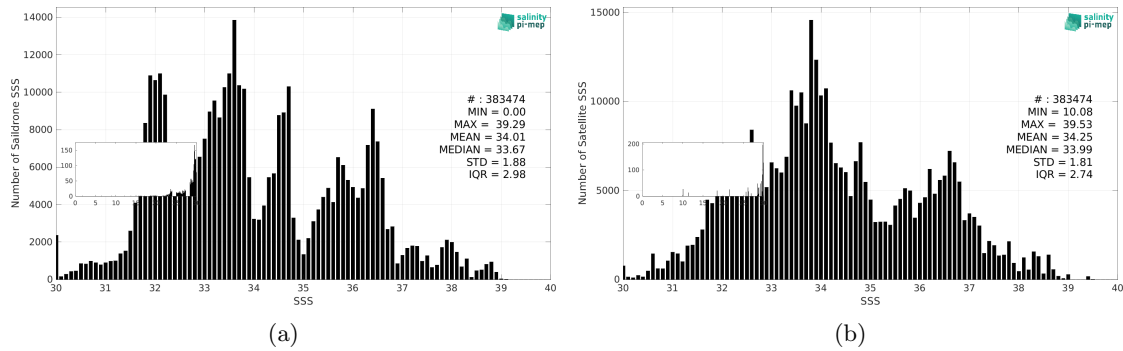
Figure 3: Histograms of SSS from Sairdrone (a) and SMAP SSS L3 v5.0 - 8-Day running (JPL) (b) considering all match-up pairs per bins of 0.1 over the SMOS coastal zone (<800km) 60N-60S Pi-MEP region and for the full satellite product period.
