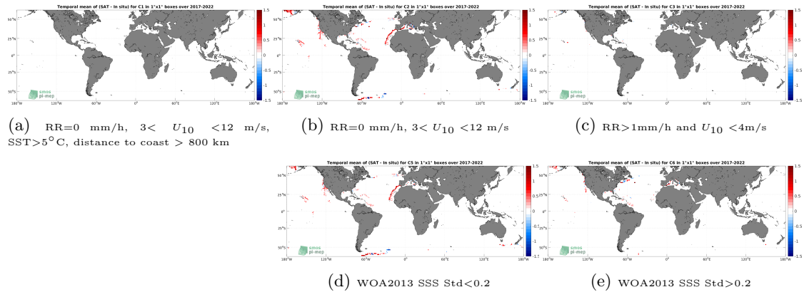
Figure 12: Temporal mean gridded over spatial boxes of size 1^\circ \times 1^\circ of \Delta\text{SSS} (SMAP SSS L3 v5.0 - 8-Day running (JPL) - Saildrone) for 5 different subdatasets corresponding to:RR=0 mm/h, 3 < U_{10} < 12 m/s, SST >5^\circ\text{C} , distance to coast > 800 km (a), RR=0 mm/h, 3 < U_{10} < 12 m/s (b), RR >1 mm/h and U_{10} < 4 m/s (c), WOA2013 SSS Std <0.2 (d), WOA2013 SSS Std >0.2 (e).
