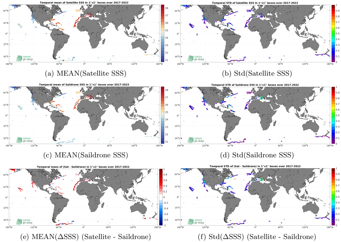
Figure 6: Temporal mean (left) and Std (right) of SSS from SMAP SSS L3 v5.0 - 8-Day running (JPL) (top), Saildrone (middle), and of \Delta SSS (Satellite - Saildrone). Only match-up pairs are used to generate these maps.
