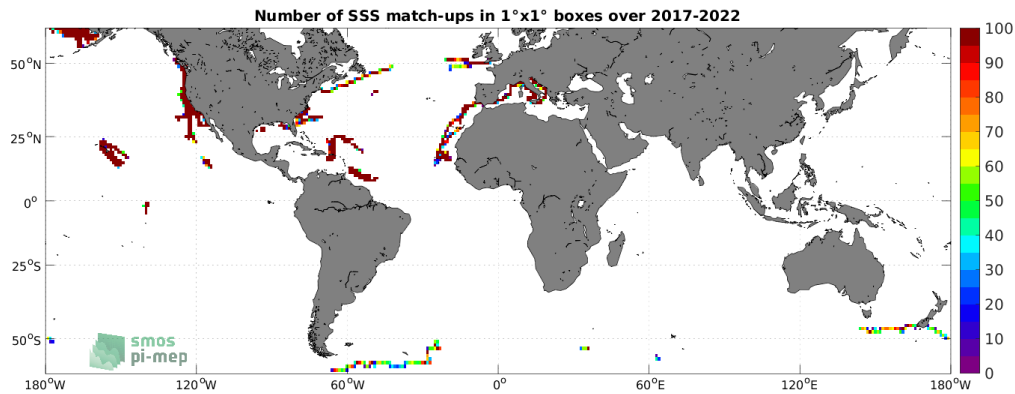
Figure 4: Number of SSS match-ups between Saildrone SSS and the SMAP SSS L3 v5.0 - 8-Day running (JPL) SSS product for the SMOS coastal zone (<800km) 60N-60S Pi-MEP region over 1^\circ \times 1^\circ boxes and for the full satellite product period.
