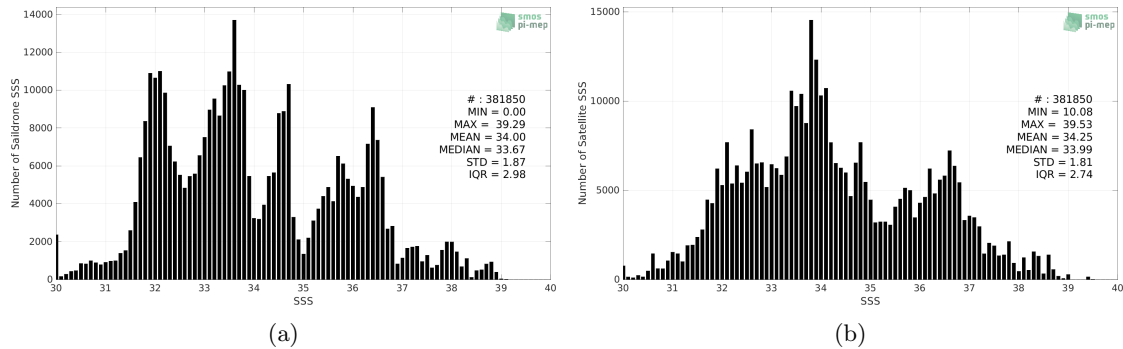
Figure 2: Histograms of SSS from Sairdrone (a) and SMAP SSS L3 v5.0 - 8-Day running (JPL) (b) considering all match-up pairs per bins of 0.1 over the SMOS coastal zone (<800km) 60N-60S Pi-MEP region and for the full satellite product period.
