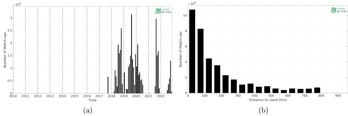
Figure 1: Number of match-ups between Sairdrone and SMAP SSS L3 v5.0 - 8-Day running (JPL) SSS as a function of time (a) and as function of the distance to coast (b) over the SMOS coastal zone (<800km) 60N-60S Pi-MEP region and for the full satellite product period.
