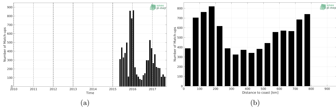
Figure 1: Number of match-ups between Sea mammals and SMAP SSS L3 v5.0 - 8-Day running (JPL) SSS as a function of time (a) and as function of the distance to coast (b) over the SMOS coastal zone (<800km) 60N-60S Pi-MEP region and for the full satellite product period.
