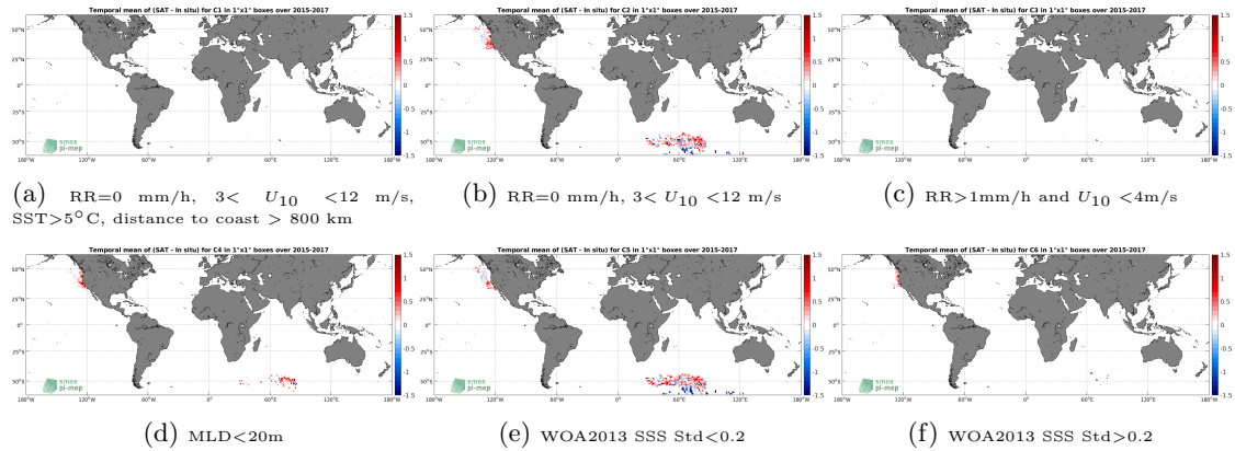
Figure 12: Temporal mean gridded over spatial boxes of size 1°x1° of \Delta SSS (SMAP SSS L3 v5.0 - 8-Day running (JPL) - Sea mammals) for 6 different subdatasets corresponding to: RR=0 mm/h, 3 < U_{10} < 12 m/s, SST > 5°C, distance to coast > 800 km (a), RR=0 mm/h, 3 < U_{10} < 12 m/s (b), RR > 1mm/h and U_{10} < 4 m/s (c), MLD < 20m (d), WOA2013 SSS Std < 0.2 (e), WOA2013 SSS Std > 0.2 (f).
