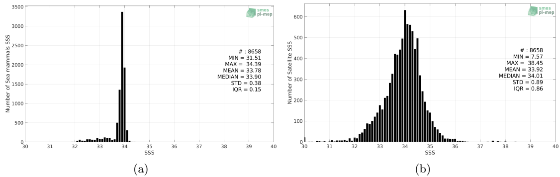
Figure 2: Histograms of SSS from Sea mammals (a) and SMAP SSS L3 v5.0 - 8-Day running (JPL) (b) considering all match-up pairs per bins of 0.1 over the SMOS coastal zone (<800km) 60N-60S Pi-MEP region and for the full satellite product period.
