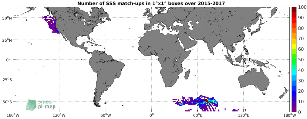
Figure 4: Number of SSS match-ups between Sea mammals SSS and the SMAP SSS L3 v5.0 - 8-Day running (JPL) SSS product for the SMOS coastal zone (<800km) 60N-60S Pi-MEP region over 1^\circ \times 1^\circ boxes and for the full satellite product period.
