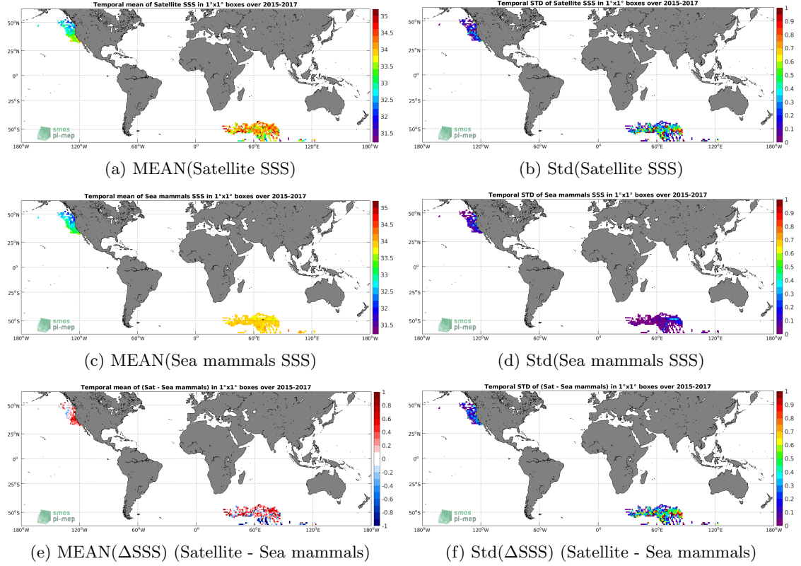
Figure 6: Temporal mean (left) and Std (right) of SSS from SMAP SSS L3 v5.0 - 8-Day running (JPL) (top), Sea mammals (middle), and of \Delta SSS (Satellite - Sea mammals). Only match-up pairs are used to generate these maps.
