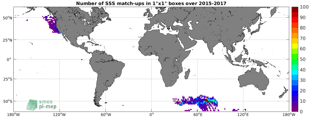
Figure 4: Number of SSS match-ups between Sea mammals SSS and the SMAP SSS L3 v5.0 - 8-Day running (JPL) SSS product for the SMOS coastal zone (<800km) 60N-60S Pi-MEP region over 1°x1° boxes and for the full satellite product period.
