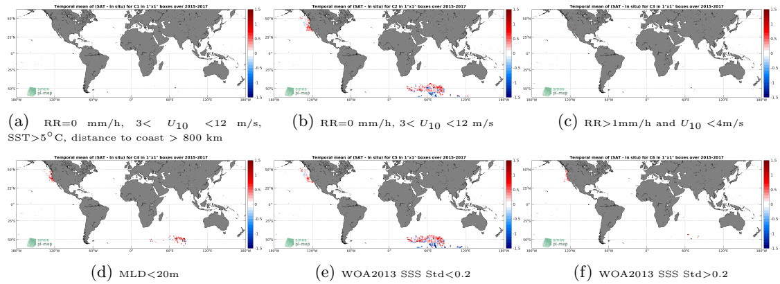
Figure 12: Temporal mean gridded over spatial boxes of size 1^\circ \times 1^\circ of \Delta SSS (SMAP SSS L3 v5.0 - 8-Day running (JPL) - Sea mammals) for 6 different subdatasets corresponding to:RR=0 mm/h, 3 < U_{10} < 12 m/s, SST >5^\circ C, distance to coast > 800 km (a), RR=0 mm/h, 3 < U_{10} < 12 m/s (b), RR >1 mm/h and U_{10} < 4 m/s (c),MLD <20 m (d),WOA2013 SSS Std <0.2 (e),WOA2013 SSS Std >0.2 (f).
