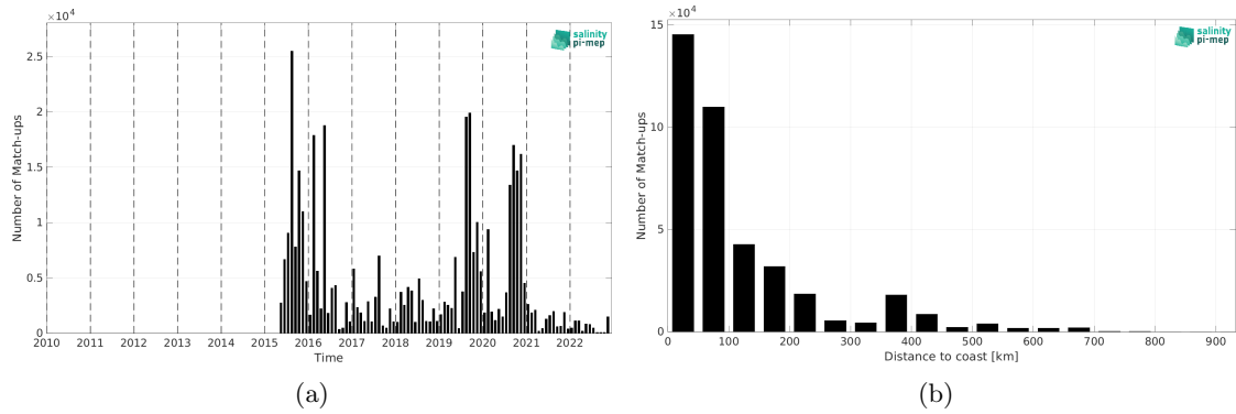
Figure 1: Number of match-ups between ICES and SMAP SSS L3 v5.0 - 8-Day running (JPL) SSS as a function of time (a) and as function of the distance to coast (b) over the SMOS coastal zone (<800km) 60N-60S Pi-MEP region and for the full satellite product period.
