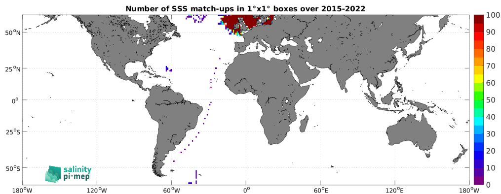
Figure 4: Number of SSS match-ups between ICES SSS and the SMAP SSS L3 v5.0 - 8-Day running (JPL) SSS product for the SMOS coastal zone (<800km) 60N-60S Pi-MEP region over 1^\circ \times 1^\circ boxes and for the full satellite product period.
