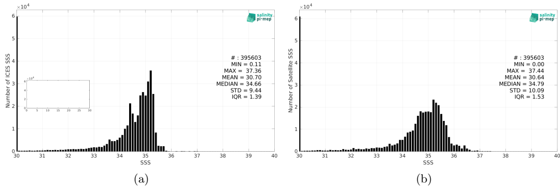
Figure 2: Histograms of SSS from ICES (a) and SMAP SSS L3 v5.0 - 8-Day running (JPL) (b) considering all match-up pairs per bins of 0.1 over the SMOS coastal zone (<800km) 60N-60S Pi-MEP region and for the full satellite product period.
