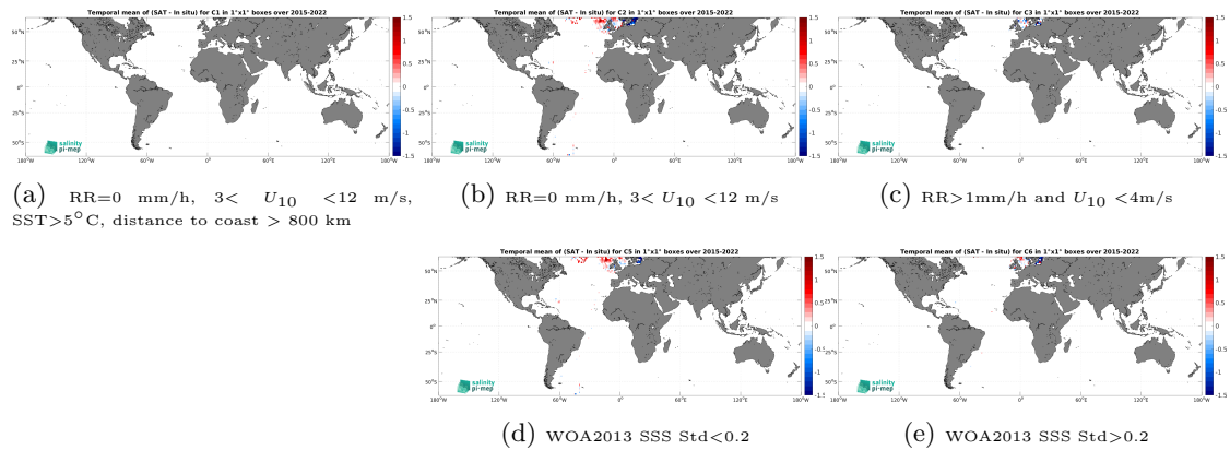
Figure 12: Temporal mean gridded over spatial boxes of size 1^\circ \times 1^\circ of \Delta SSS (SMAP SSS L3 v5.0 - 8-Day running (JPL) - ICES) for 5 different subdatasets corresponding to: RR=0 mm/h, 3 < U_{10} < 12 m/s, SST > 5^\circ\text{C} , distance to coast > 800 km (a), RR=0 mm/h, 3 < U_{10} < 12 m/s (b), RR > 1 mm/h and U_{10} < 4 m/s (c), WOA2013 SSS Std < 0.2 (d), WOA2013 SSS Std > 0.2 (e).
