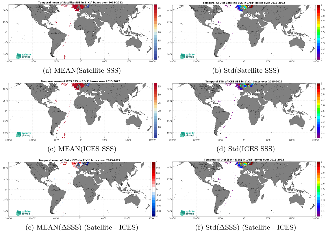
Figure 6: Temporal mean (left) and Std (right) of SSS from SMAP SSS L3 v5.0 - 8-Day running (JPL) (top), ICES (middle), and of \Delta SSS (Satellite - ICES). Only match-up pairs are used to generate these maps.
