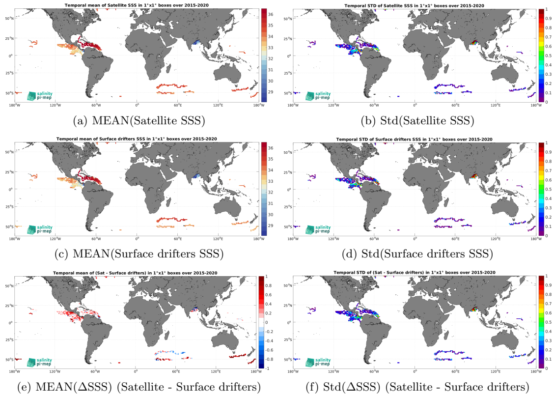
Figure 6: Temporal mean (left) and Std (right) of SSS from SMAP SSS L3 v5.0 - 8-Day running (JPL) (top), Surface drifters (middle), and of \Delta SSS (Satellite - Surface drifters). Only match-up pairs are used to generate these maps.
