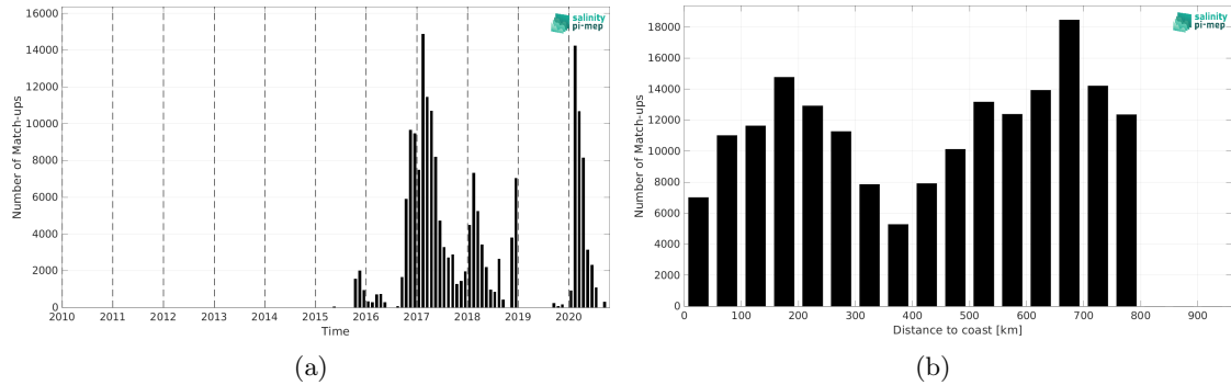
Figure 2: Number of match-ups between Surface drifters and SMAP SSS L3 v5.0 - 8-Day running (JPL) SSS as a function of time (a) and as function of the distance to coast (b) over the SMOS coastal zone (<800km) 60N-60S Pi-MEP region and for the full satellite product period.
