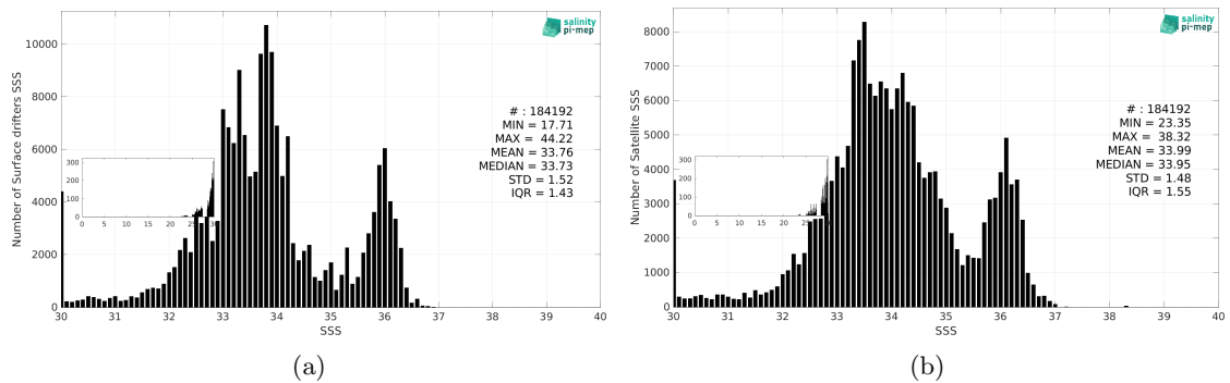
Figure 3: Histograms of SSS from Surface drifters (a) and SMAP SSS L3 v5.0 - 8-Day running (JPL) (b) considering all match-up pairs per bins of 0.1 over the SMOS coastal zone (<800km) 60N-60S Pi-MEP region and for the full satellite product period.
