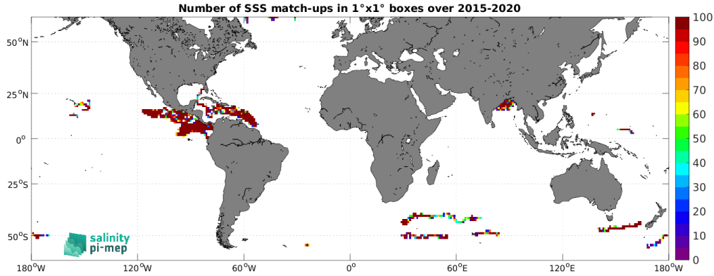
Figure 4: Number of SSS match-ups between Surface drifters SSS and the SMAP SSS L3 v5.0 - 8-Day running (JPL) SSS product for the SMOS coastal zone (<800km) 60N-60S Pi-MEP region over 1^\circ \times 1^\circ boxes and for the full satellite product period.
