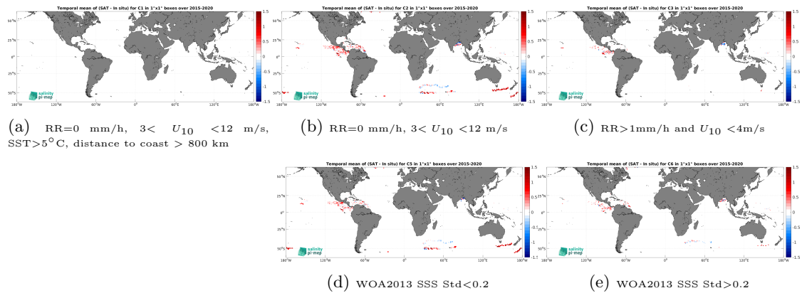
Figure 13: Temporal mean gridded over spatial boxes of size 1^\circ \times 1^\circ of \Delta\text{SSS} (SMAP SSS L3 v5.0 - 8-Day running (JPL) - Surface drifters) for 5 different subdatasets corresponding to:RR=0 mm/h, 3 < U_{10} < 12 m/s, SST >5^\circ\text{C} , distance to coast > 800 km (a), RR=0 mm/h, 3 < U_{10} < 12 m/s (b), RR >1 mm/h and U_{10} < 4 m/s (c), WOA2013 SSS Std <0.2 (d), WOA2013 SSS Std >0.2 (e).
