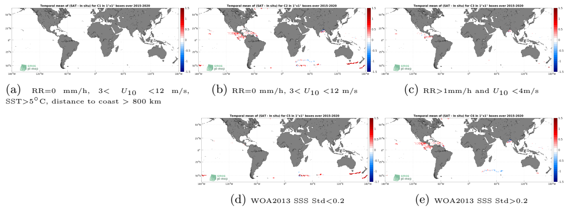
Figure 11: Temporal mean gridded over spatial boxes of size 1^\circ \times 1^\circ of \Delta SSS (SMAP SSS L3 v5.0 - 8-Day running (JPL) - Surface drifters) for 5 different subdatasets corresponding to:RR=0 mm/h, 3 < U_{10} < 12 m/s, SST >5^\circ\text{C} , distance to coast > 800 km (a), RR=0 mm/h, 3 < U_{10} < 12 m/s (b), RR >1 mm/h and U_{10} < 4 m/s (c), WOA2013 SSS Std <0.2 (d), WOA2013 SSS Std >0.2 (e).
