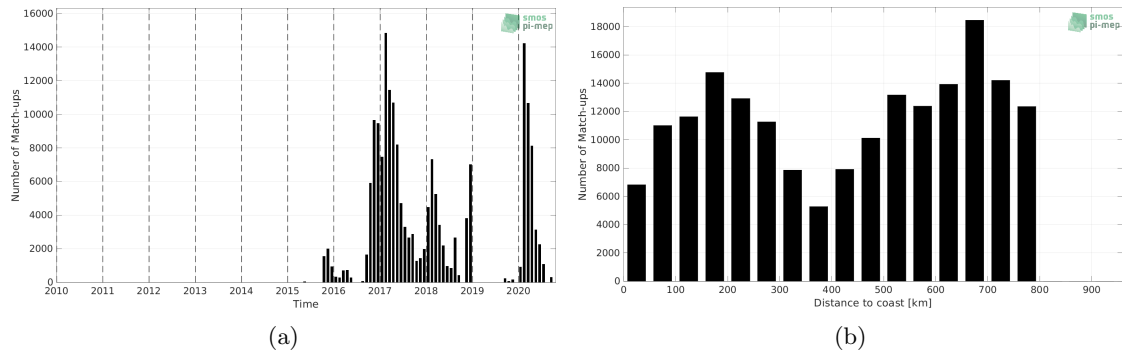
Figure 1: Number of match-ups between Surface drifters and SMAP SSS L3 v5.0 - 8-Day running (JPL) SSS as a function of time (a) and as function of the distance to coast (b) over the SMOS coastal zone (<800km) 60N-60S Pi-MEP region and for the full satellite product period.
