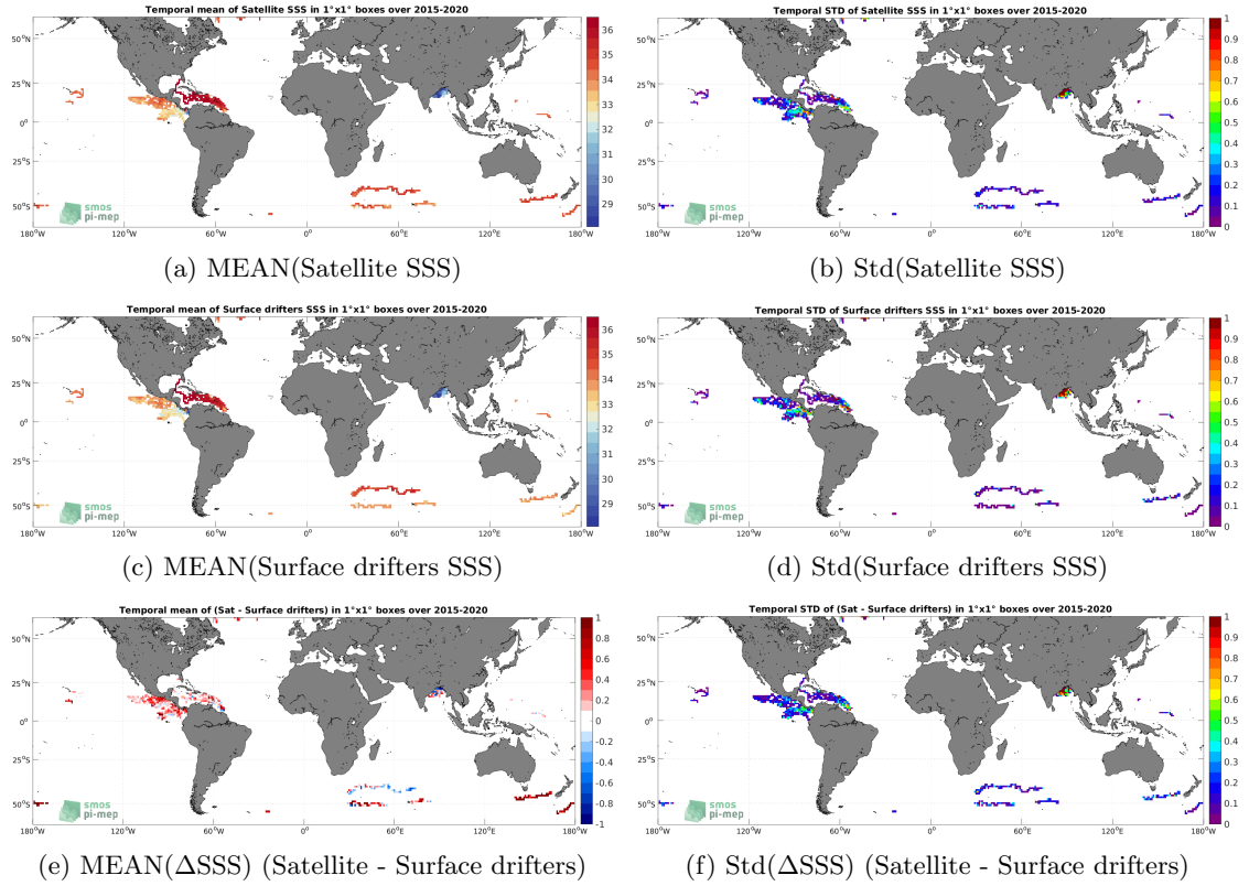
Figure 5: Temporal mean (left) and Std (right) of SSS from SMAP SSS L3 v5.0 - 8-Day running (JPL) (top), Surface drifters (middle), and of \Delta SSS (Satellite - Surface drifters). Only match-up pairs are used to generate these maps.
