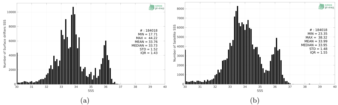
Figure 2: Histograms of SSS from Surface drifters (a) and SMAP SSS L3 v5.0 - 8-Day running (JPL) (b) considering all match-up pairs per bins of 0.1 over the SMOS coastal zone (<800km) 60N-60S Pi-MEP region and for the full satellite product period.
