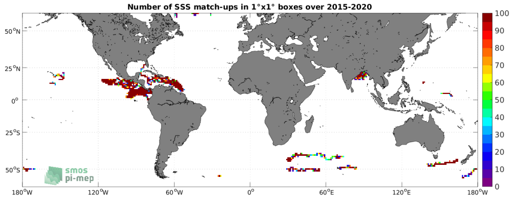
Figure 3: Number of SSS match-ups between Surface drifters SSS and the SMAP SSS L3 v5.0 - 8-Day running (JPL) SSS product for the SMOS coastal zone (<800km) 60N-60S Pi-MEP region over 1^\circ \times 1^\circ boxes and for the full satellite product period.
