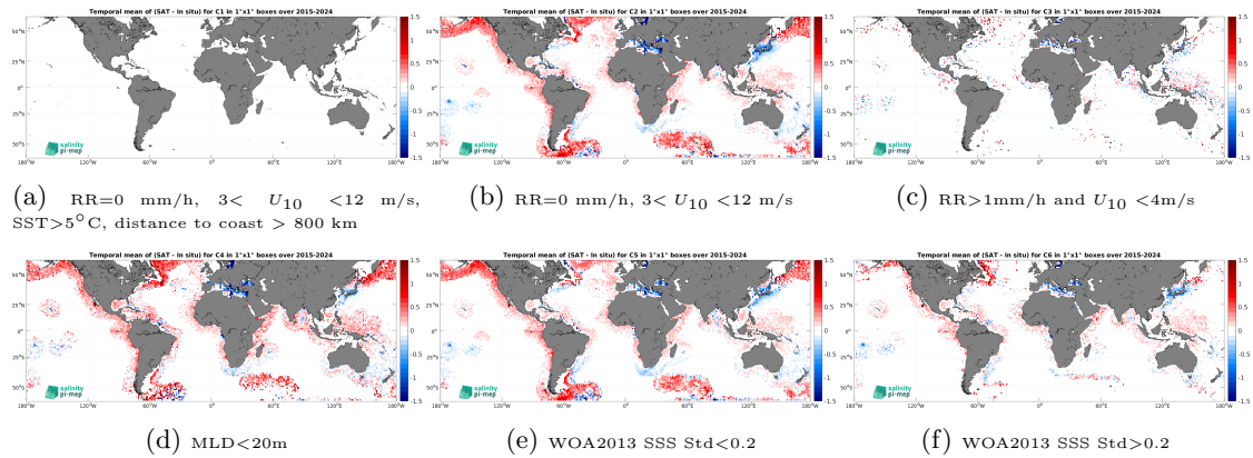
Figure 14: Temporal mean gridded over spatial boxes of size 1^\circ \times 1^\circ of \Delta SSS (SMAP SSS L3 v5.0 - 8-Day running (JPL) - Argo) for 6 different subdatasets corresponding to:RR=0 mm/h, 3 < U_{10} < 12 m/s, SST >5^\circ C, distance to coast > 800 km (a), RR=0 mm/h, 3 < U_{10} < 12 m/s (b), RR >1 mm/h and U_{10} < 4 m/s (c),MLD <20 m (d),WOA2013 SSS Std <0.2 (e),WOA2013 SSS Std >0.2 (f).
