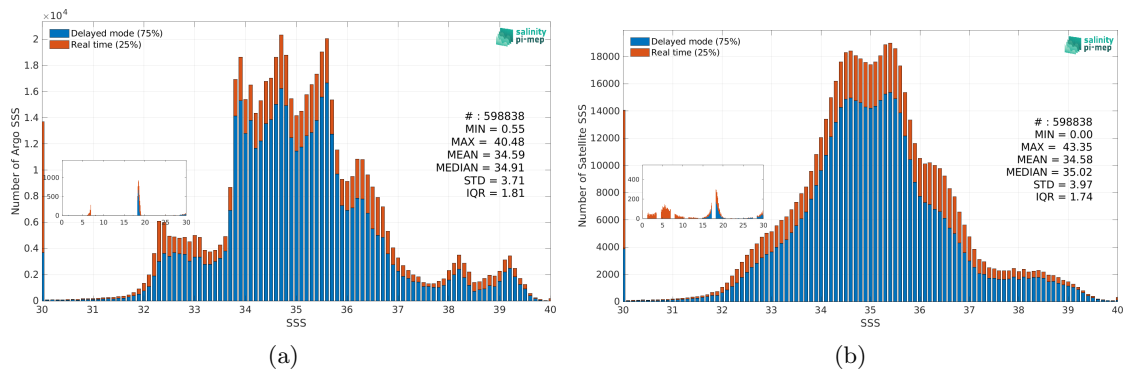
Figure 3: Histograms of SSS from Argo (a) and SMAP SSS L3 v5.0 - 8-Day running (JPL) (b) considering all match-up pairs per bins of 0.1 over the SMOS coastal zone (<800km) 60N-60S Pi-MEP region and for the full satellite product period.
