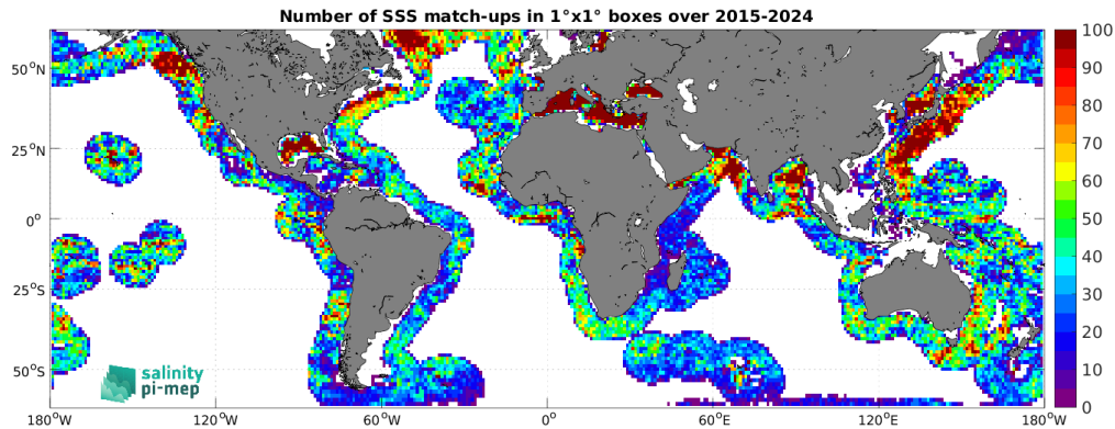
Figure 5: Number of SSS match-ups between Argo SSS and the SMAP SSS L3 v5.0 - 8-Day running (JPL) SSS product for the SMOS coastal zone ( <800\text{km} ) 60N-60S Pi-MEP region over 1^\circ \times 1^\circ boxes and for the full satellite product period.
