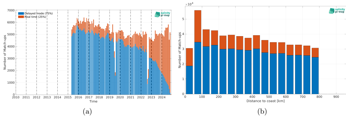
Figure 2: Number of match-ups between Argo and SMAP SSS L3 v5.0 - 8-Day running (JPL) SSS as a function of time (a) and as function of the distance to coast (b) over the SMOS coastal zone (<800km) 60N-60S Pi-MEP region and for the full satellite product period.
