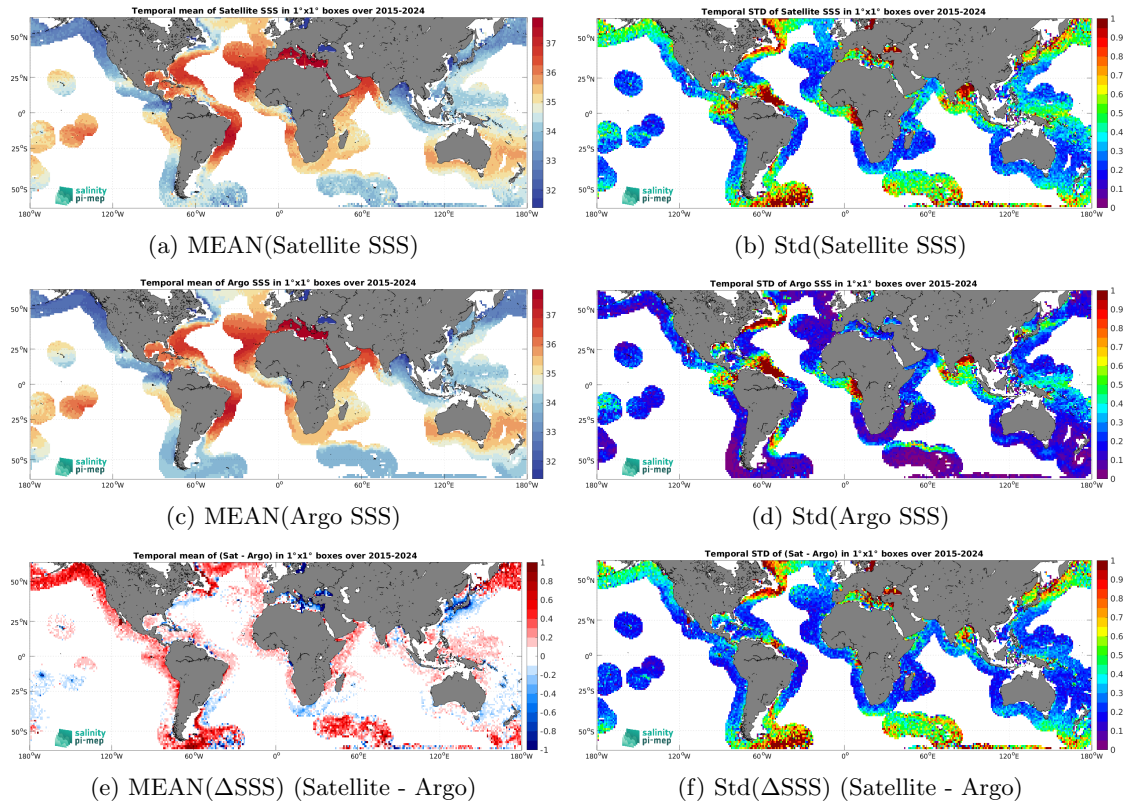
Figure 7: Temporal mean (left) and Std (right) of SSS from SMAP SSS L3 v5.0 - 8-Day running (JPL) (top), Argo (middle), and of \Delta SSS (Satellite - Argo). Only match-up pairs are used to generate these maps.
