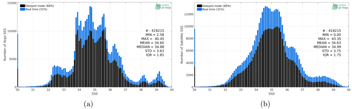
Figure 2: Histograms of SSS from Argo (a) and SMAP SSS L3 v5.0 - 8-Day running (JPL) (b) considering all match-up pairs per bins of 0.1 over the SMOS coastal zone (<800km) 60N-60S Pi-MEP region and for the full satellite product period.
