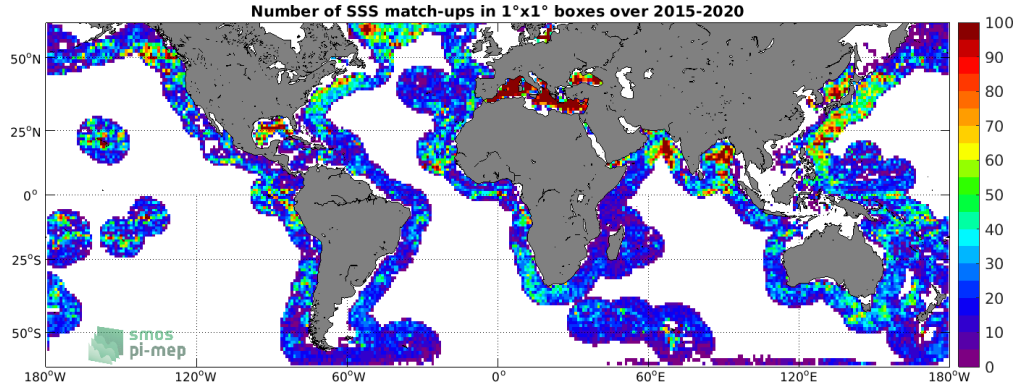
Figure 4: Number of SSS match-ups between Argo SSS and the SMAP SSS L3 v5.0 - 8-Day running (JPL) SSS product for the SMOS coastal zone (<800km) 60N-60S Pi-MEP region over 1°x1° boxes and for the full satellite product period.
