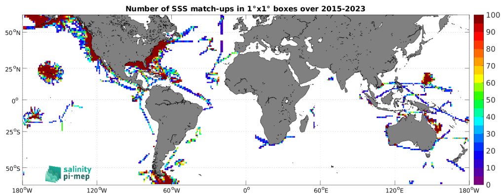
Figure 5: Number of SSS match-ups between TSG (SAMOS) SSS and the SMAP SSS L3 v5.0 - Monthly (JPL) SSS product for the SMOS coastal zone ( <800\text{km} ) 60\text{N} - 60\text{S} Pi-MEP region over 1^\circ \times 1^\circ boxes and for the full satellite product period.
