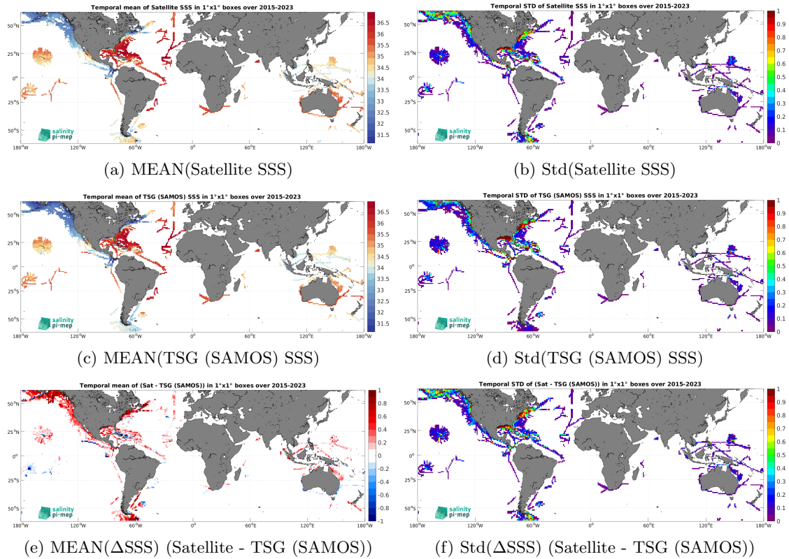
Figure 7: Temporal mean (left) and Std (right) of SSS from SMAP SSS L3 v5.0 - Monthly (JPL) (top), TSG (SAMOS) (middle), and of \Delta SSS (Satellite - TSG (SAMOS)). Only match-up pairs are used to generate these maps.
