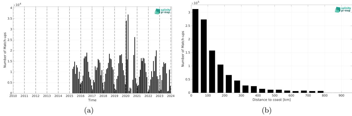
Figure 2: Number of match-ups between TSG (SAMOS) and SMAP SSS L3 v5.0 - Monthly (JPL) SSS as a function of time (a) and as function of the distance to coast (b) over the SMOS coastal zone ( <800\text{km} ) 60N-60S Pi-MEP region and for the full satellite product period.
