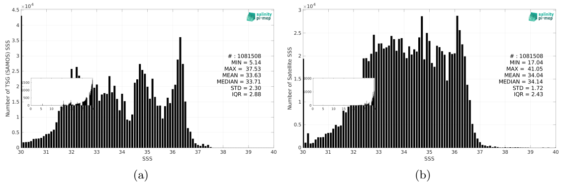
Figure 3: Histograms of SSS from TSG (SAMOS) (a) and SMAP SSS L3 v5.0 - Monthly (JPL) (b) considering all match-up pairs per bins of 0.1 over the SMOS coastal zone ( <800\text{km} ) 60N-60S Pi-MEP region and for the full satellite product period.
