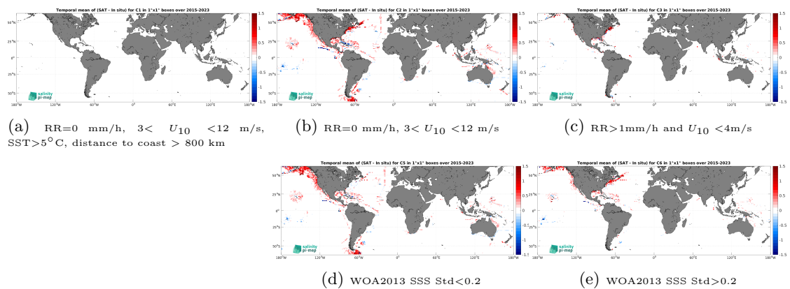
Figure 14: Temporal mean gridded over spatial boxes of size 1^\circ \times 1^\circ of \Delta SSS (SMAP SSS L3 v5.0 - Monthly (JPL) - TSG (SAMOS)) for 5 different subdatasets corresponding to:RR=0 mm/h, 3 < U_{10} < 12 m/s, SST >5^\circ\text{C} , distance to coast > 800 km (a), RR=0 mm/h, 3 < U_{10} < 12 m/s (b), RR >1 mm/h and U_{10} < 4 m/s (c), WOA2013 SSS Std <0.2 (d), WOA2013 SSS Std >0.2 (e).
